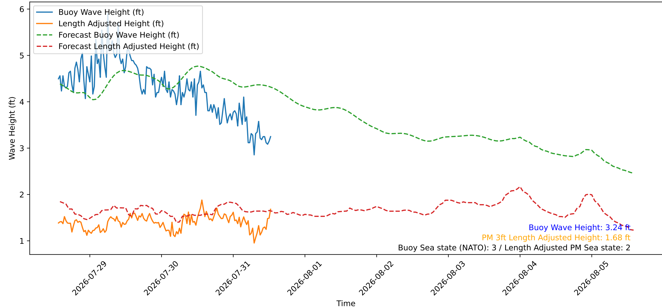
Wave Heights over Time for Oceanside Harbor at 2026-07-31 13:30:26
