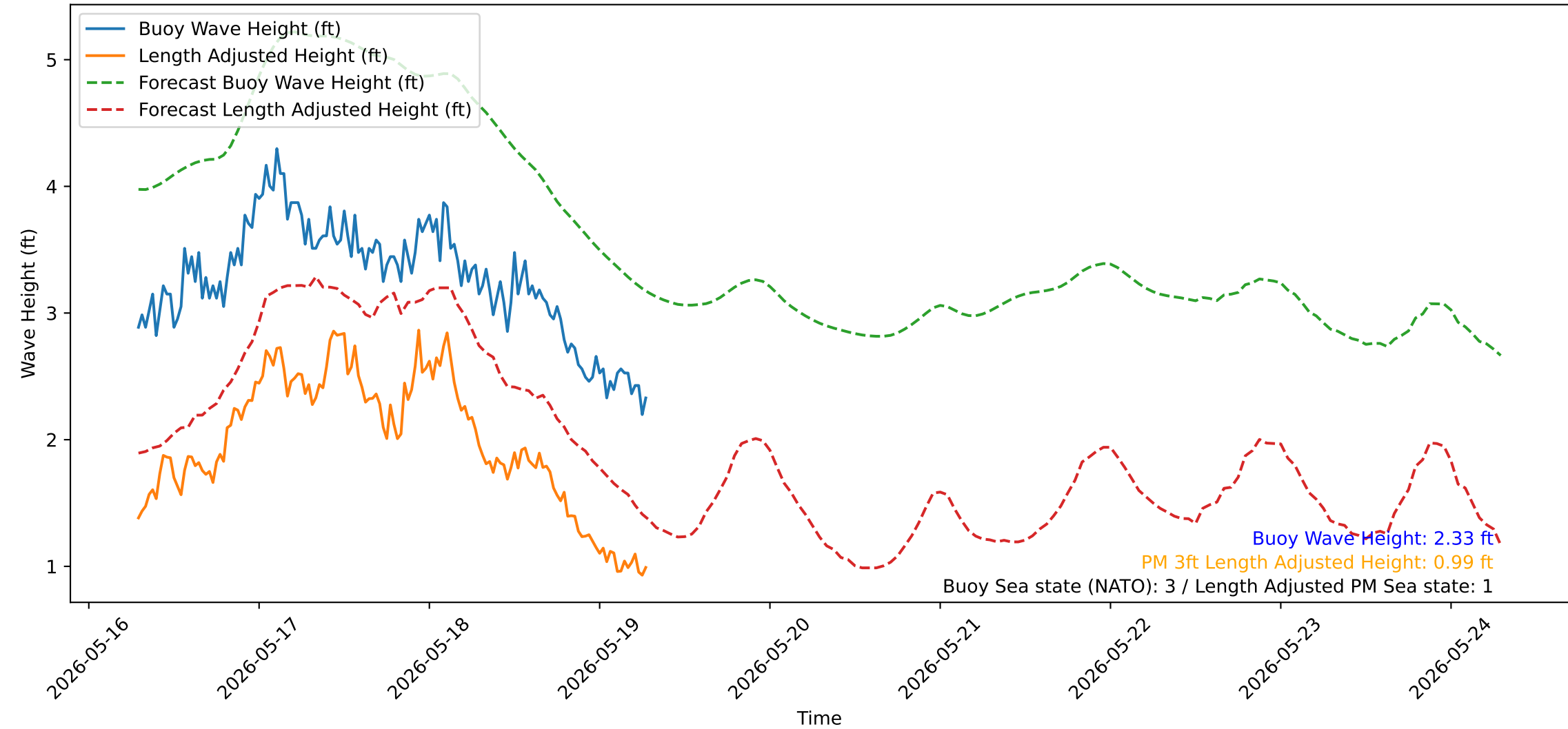
Wave Heights over Time for Oceanside Harbor at 2026-05-19 07:00:31
