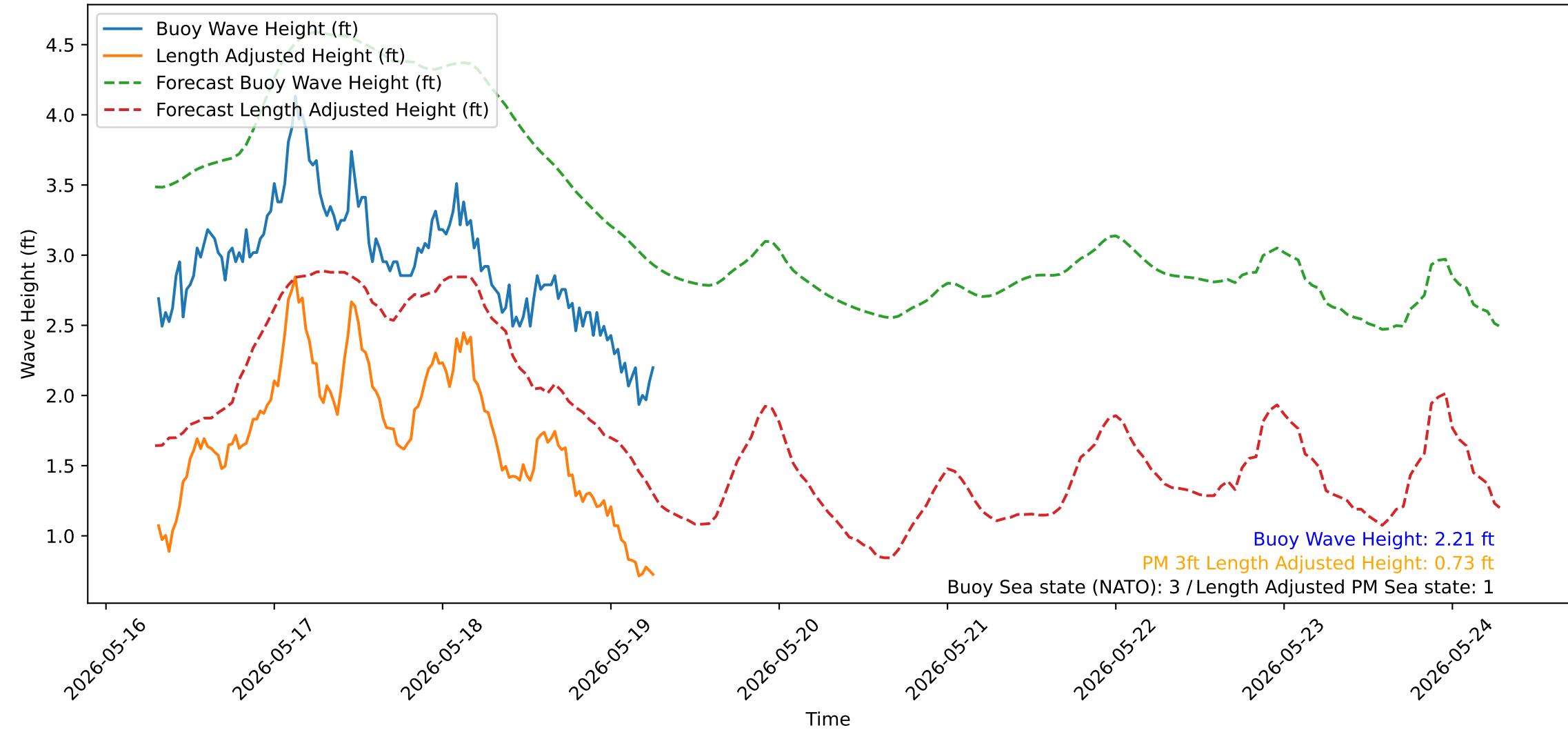
Wave Heights over Time for Red Beach at 2026-05-19 07:00:51
