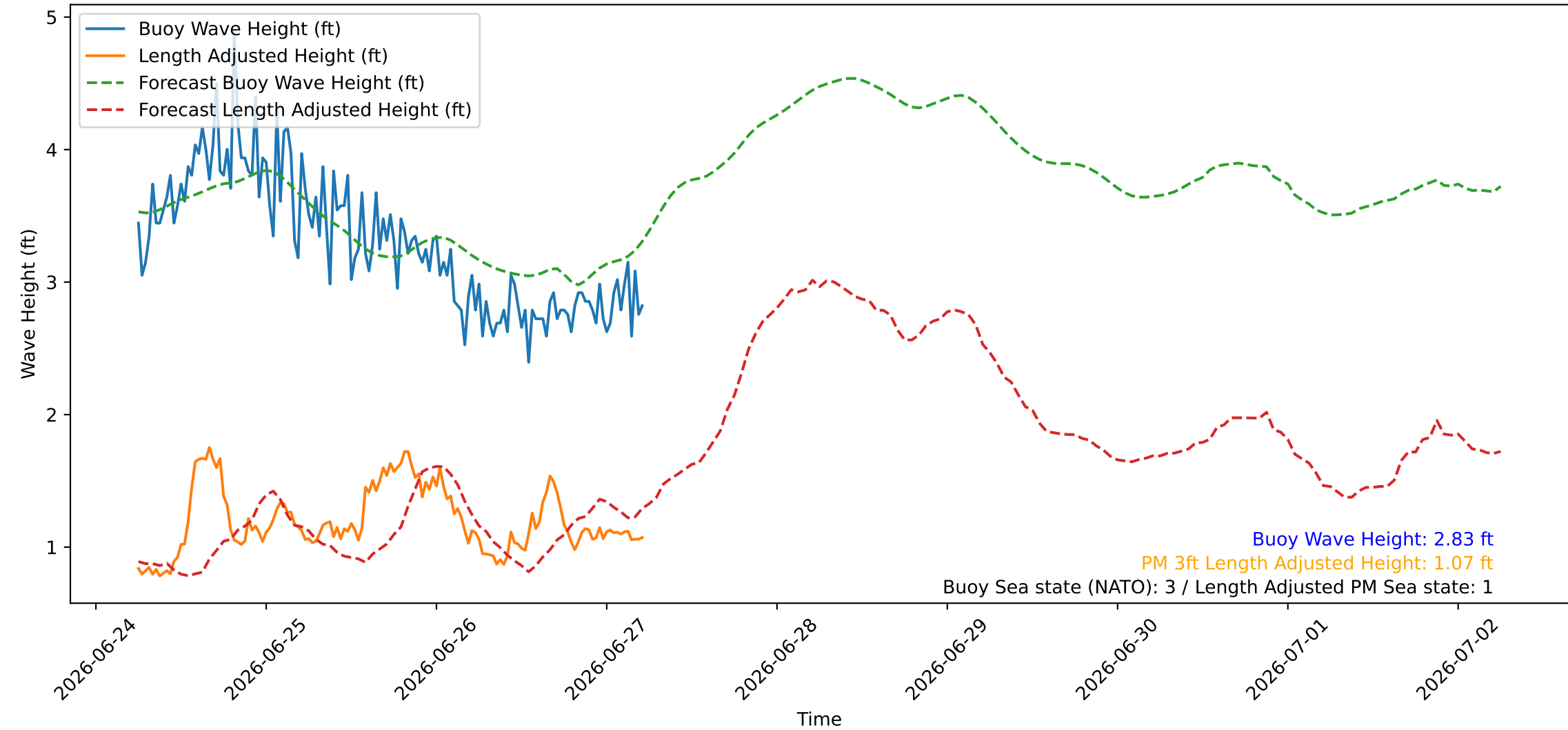
Wave Heights over Time for Oceanside Harbor at 2026-06-27 06:00:26
