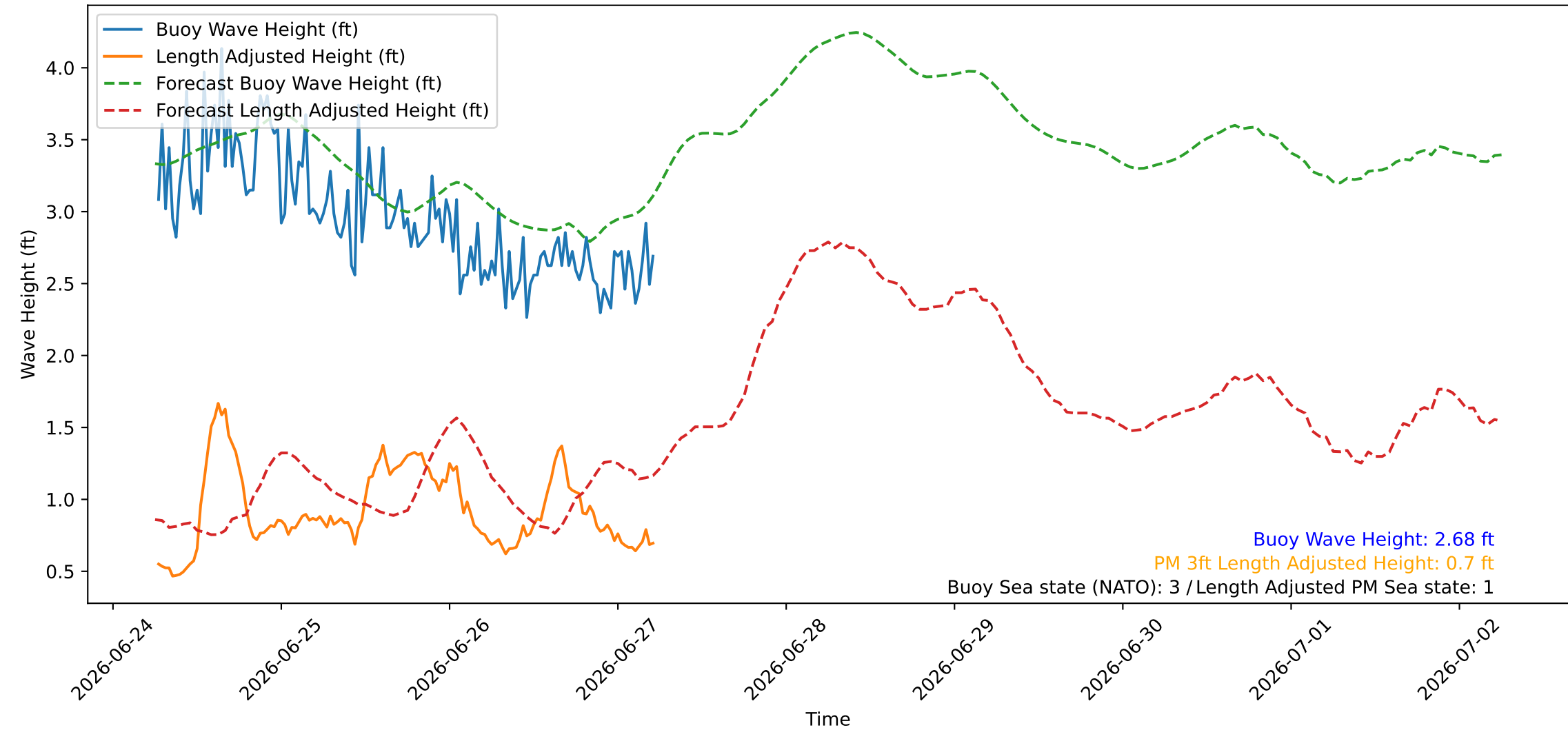
Wave Heights over Time for Red Beach at 2026-06-27 06:00:45
