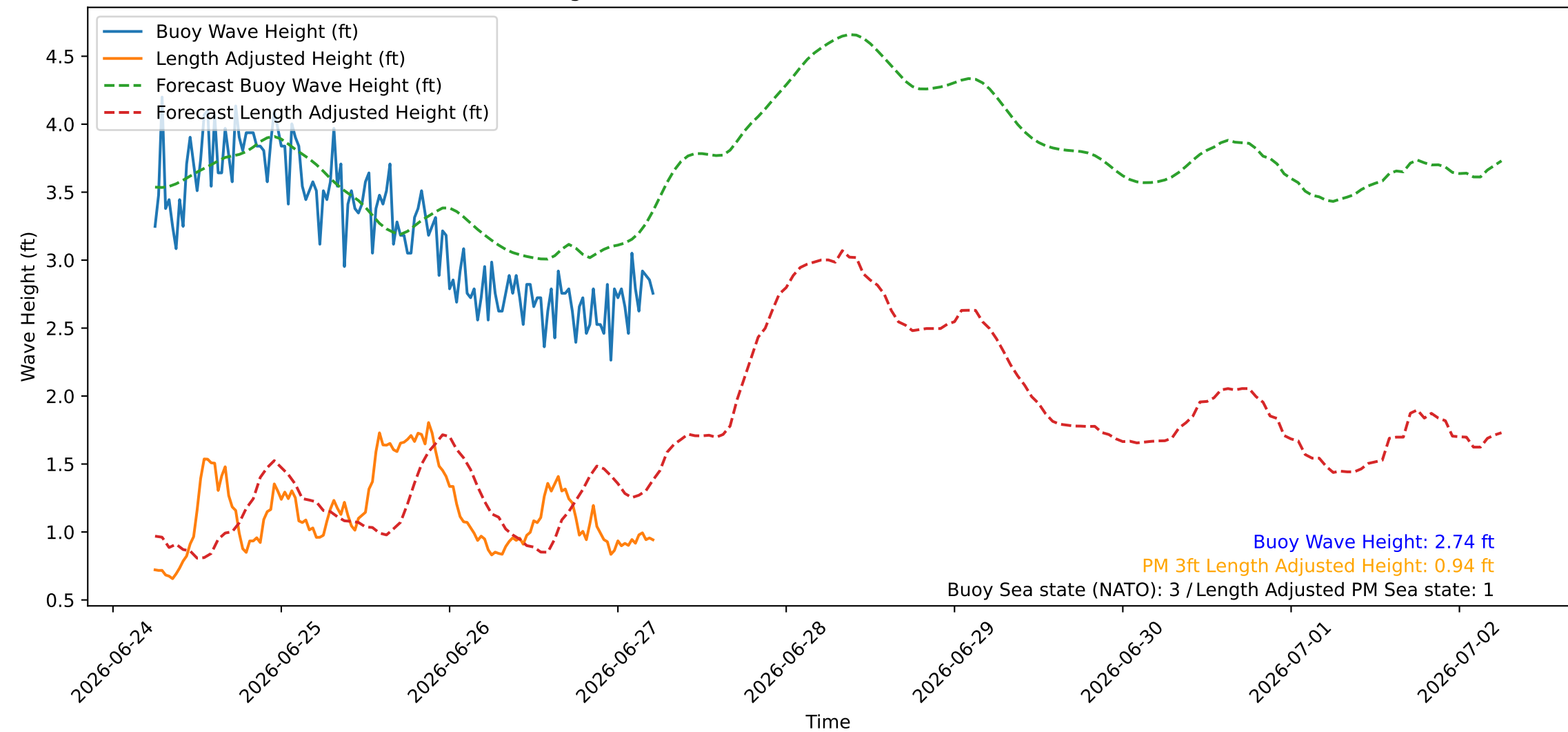
Wave Heights over Time for Green Beach at 2026-06-27 06:01:07
