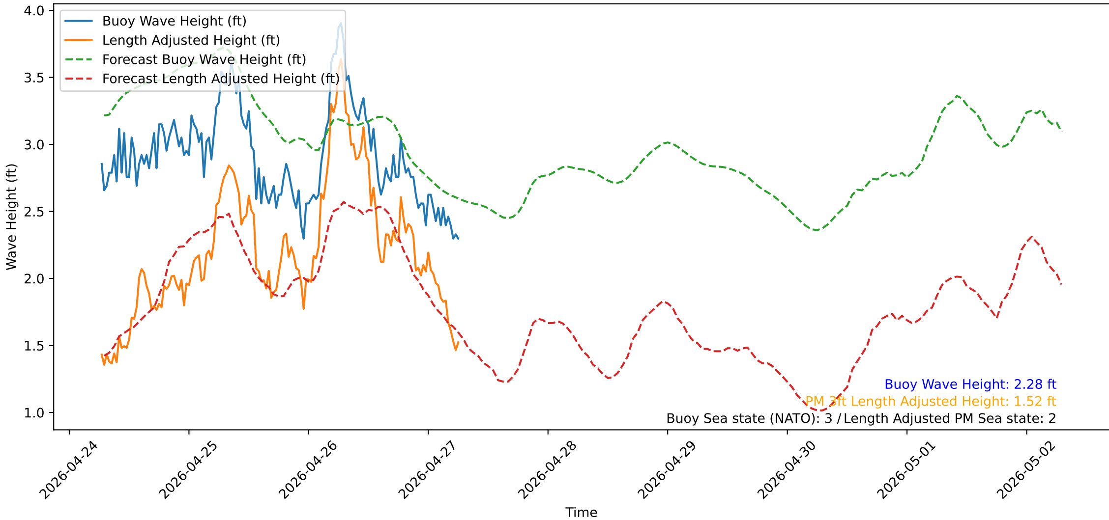
Wave Heights over Time for Oceanside Harbor at 2026-04-27 06:30:31
