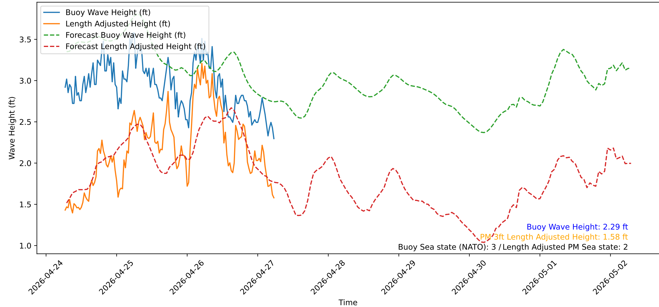
Wave Heights over Time for Green Beach at 2026-04-27 06:31:12
