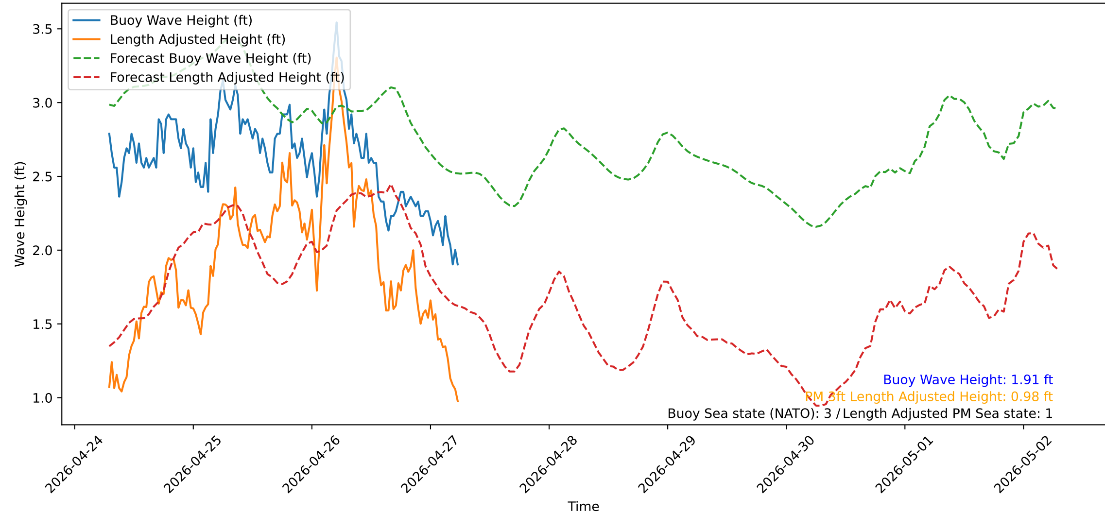
Wave Heights over Time for Red Beach at 2026-04-27 06:30:50
