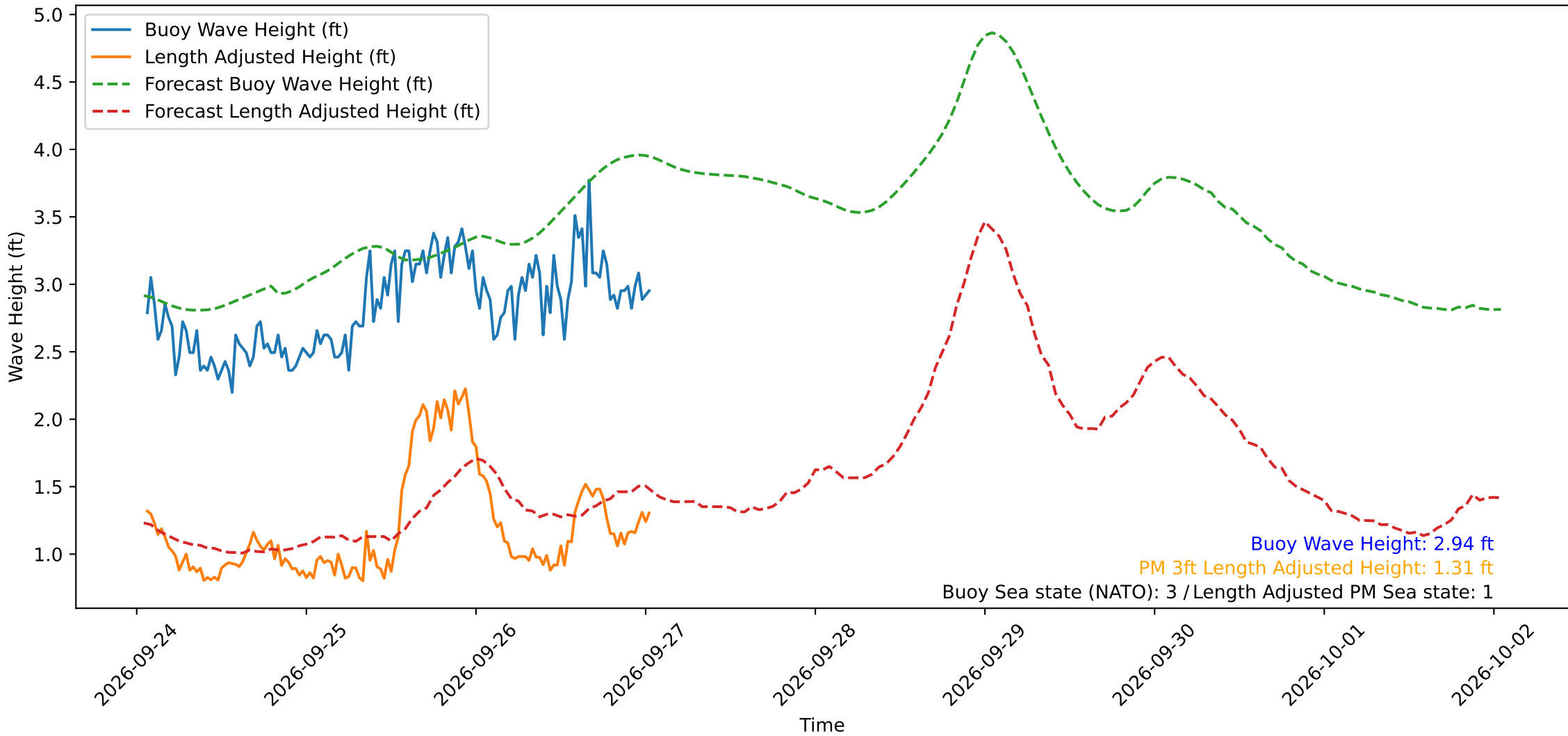
Wave Heights over Time for Oceanside Harbor at 2026-09-27 01:20:29
