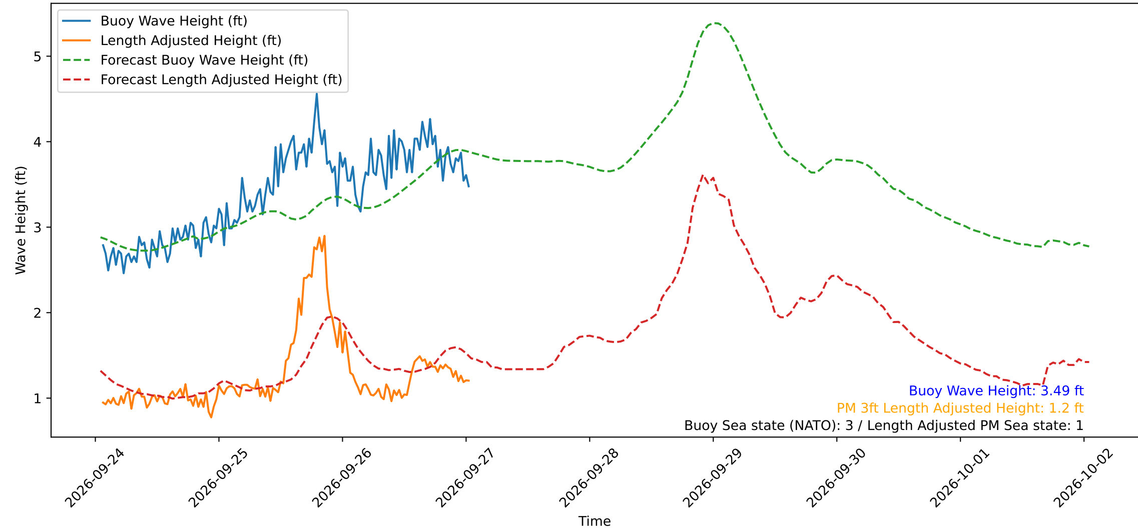
Wave Heights over Time for Green Beach at 2026-09-27 01:21:15
