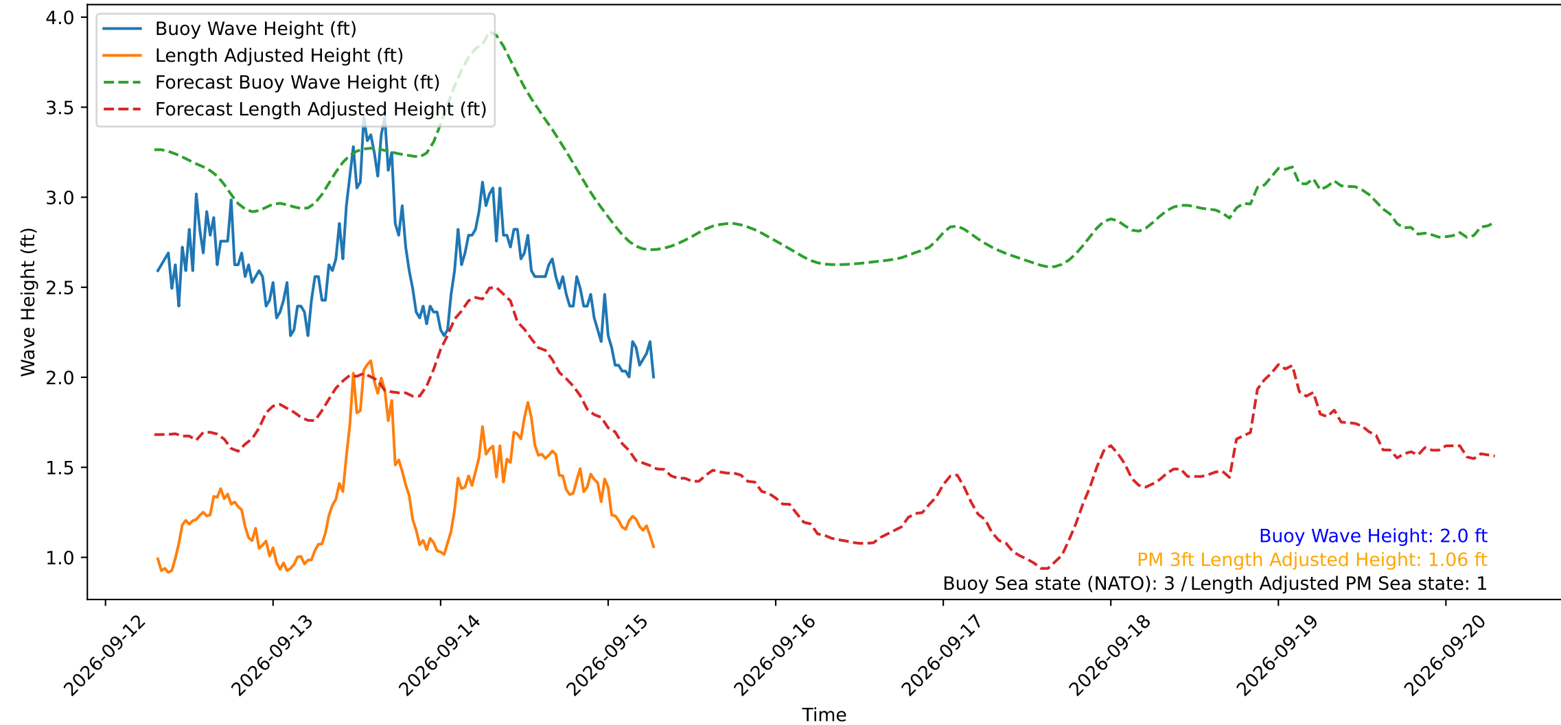
Wave Heights over Time for Red Beach at 2026-09-15 07:10:49
