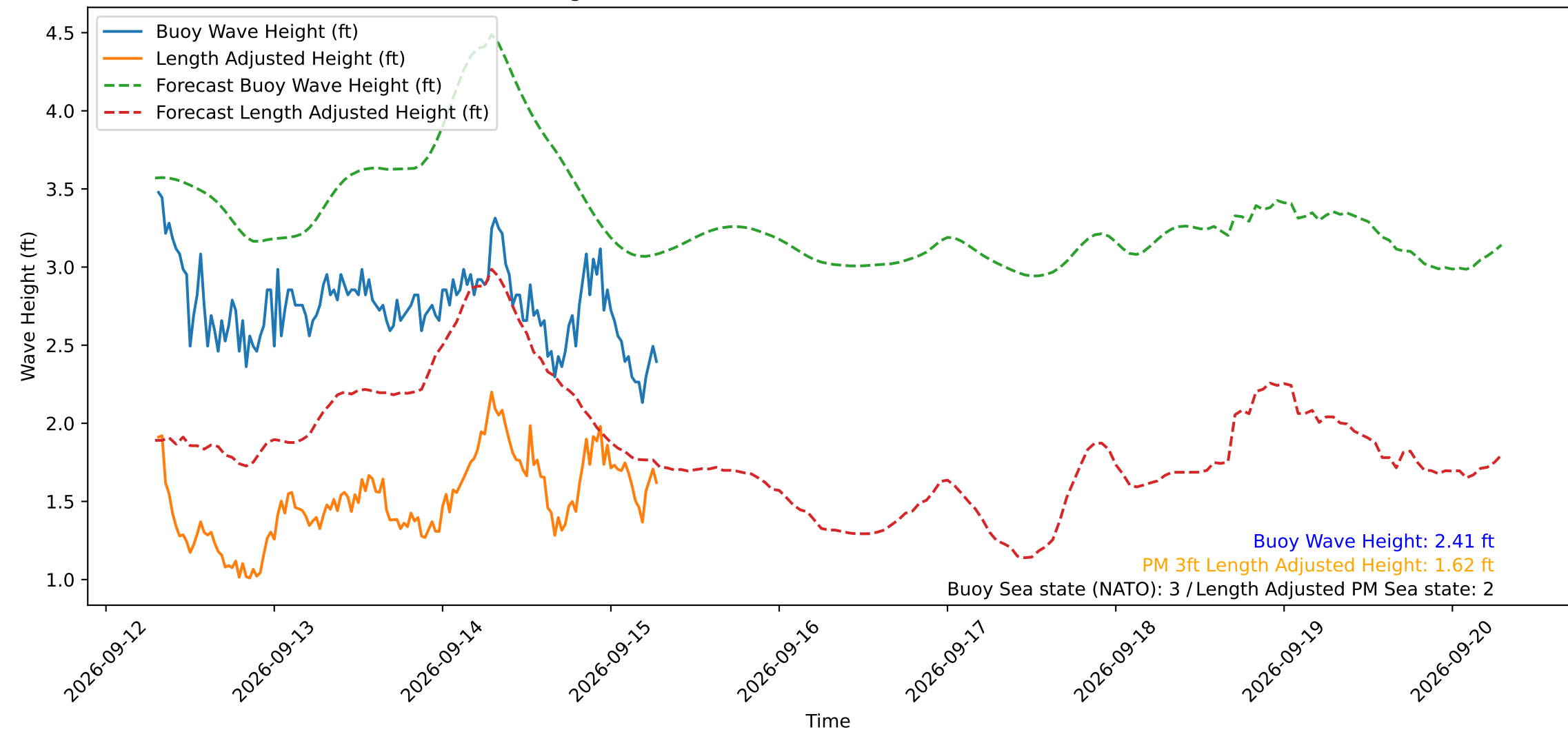
Wave Heights over Time for Green Beach at 2026-09-15 07:11:11
