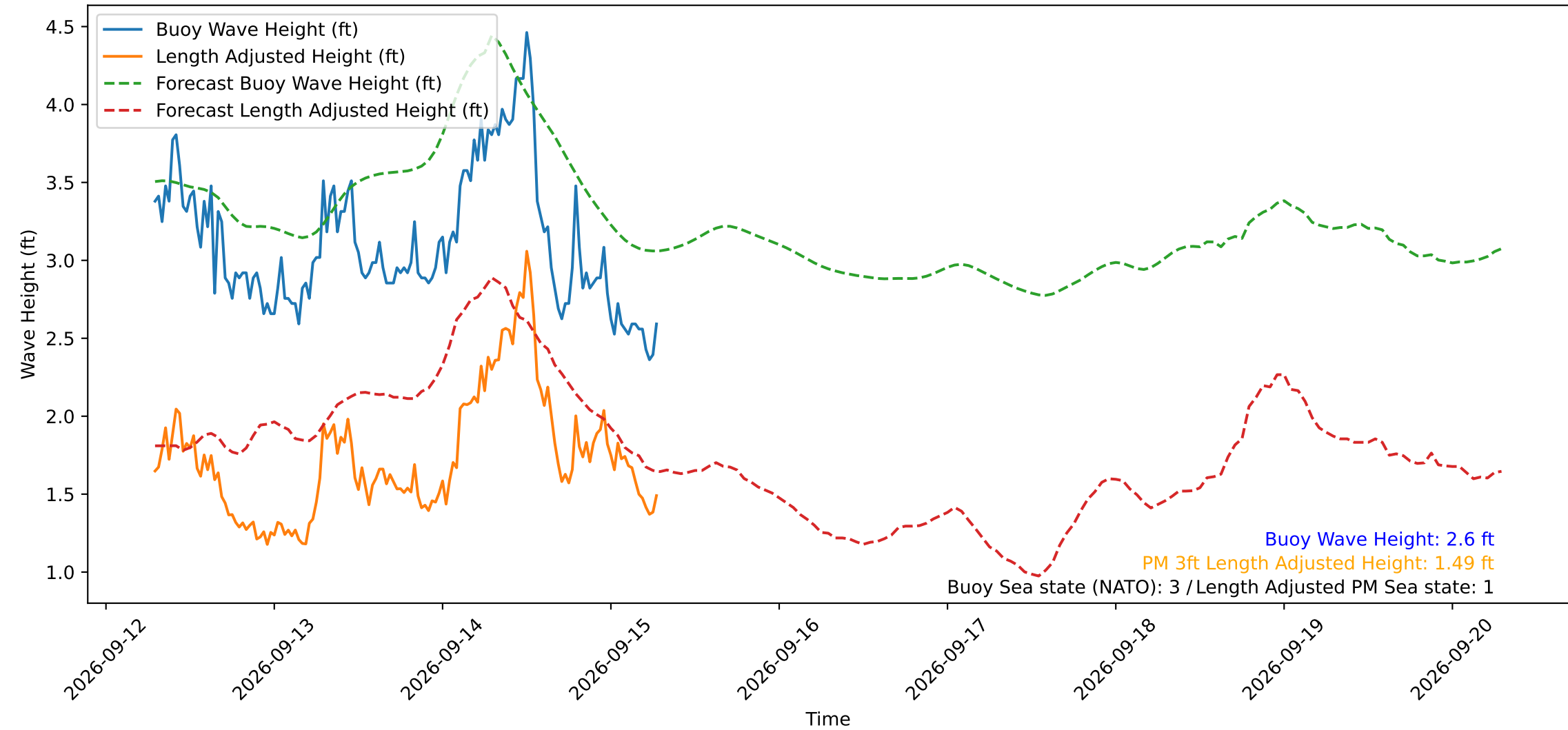
Wave Heights over Time for Oceanside Harbor at 2026-09-15 07:10:29
