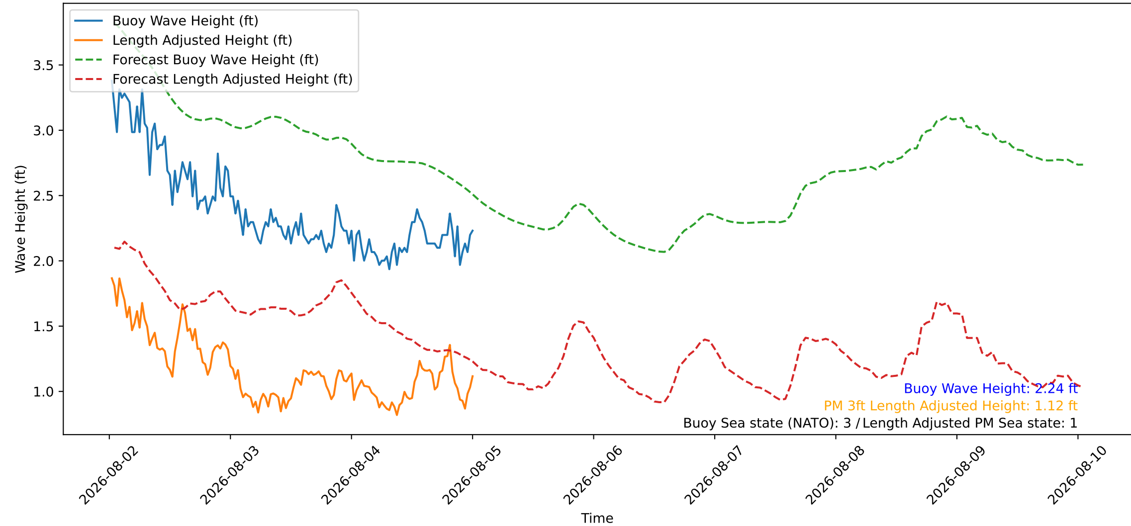
Wave Heights over Time for Green Beach at 2026-08-05 00:41:10
