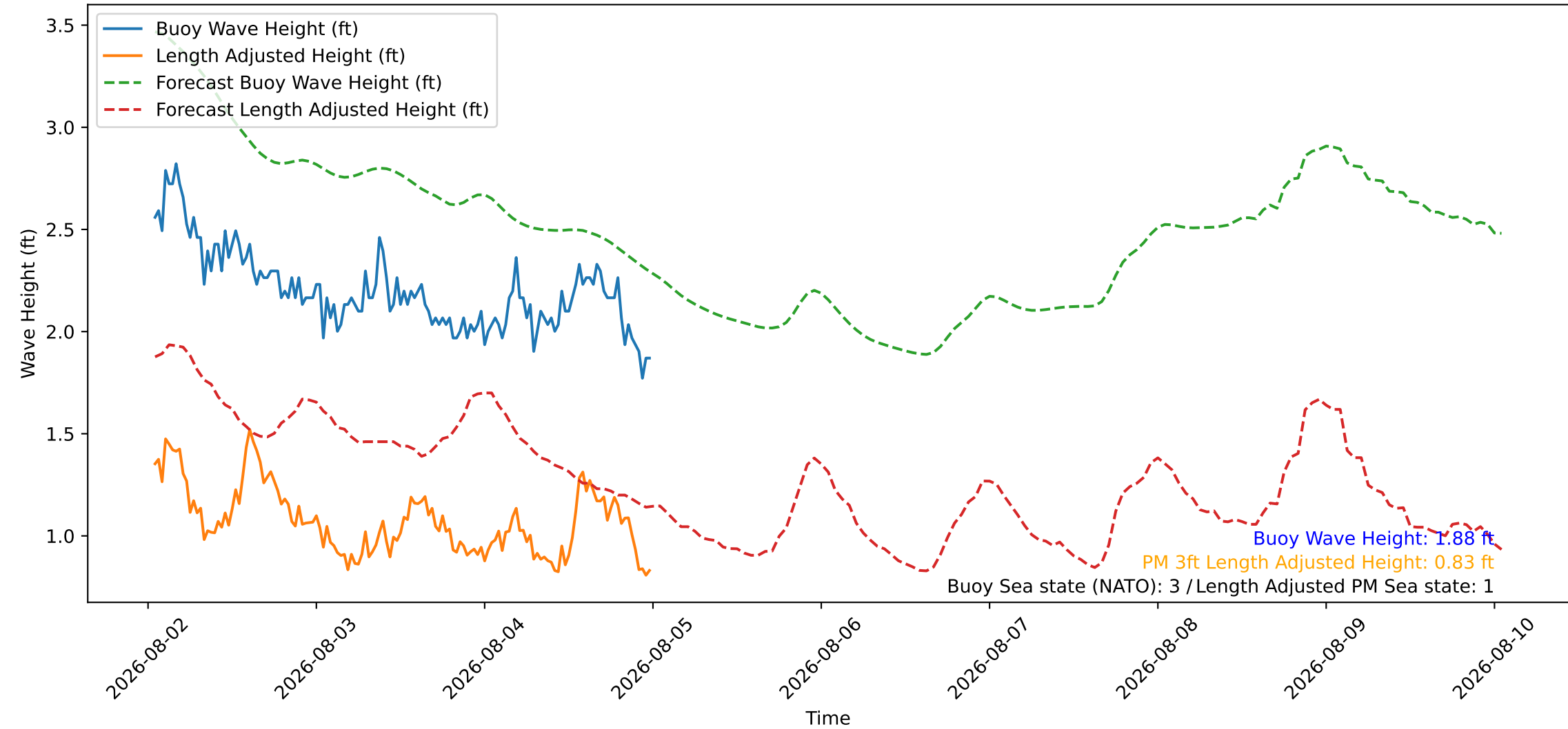
Wave Heights over Time for Red Beach at 2026-08-05 00:40:46
