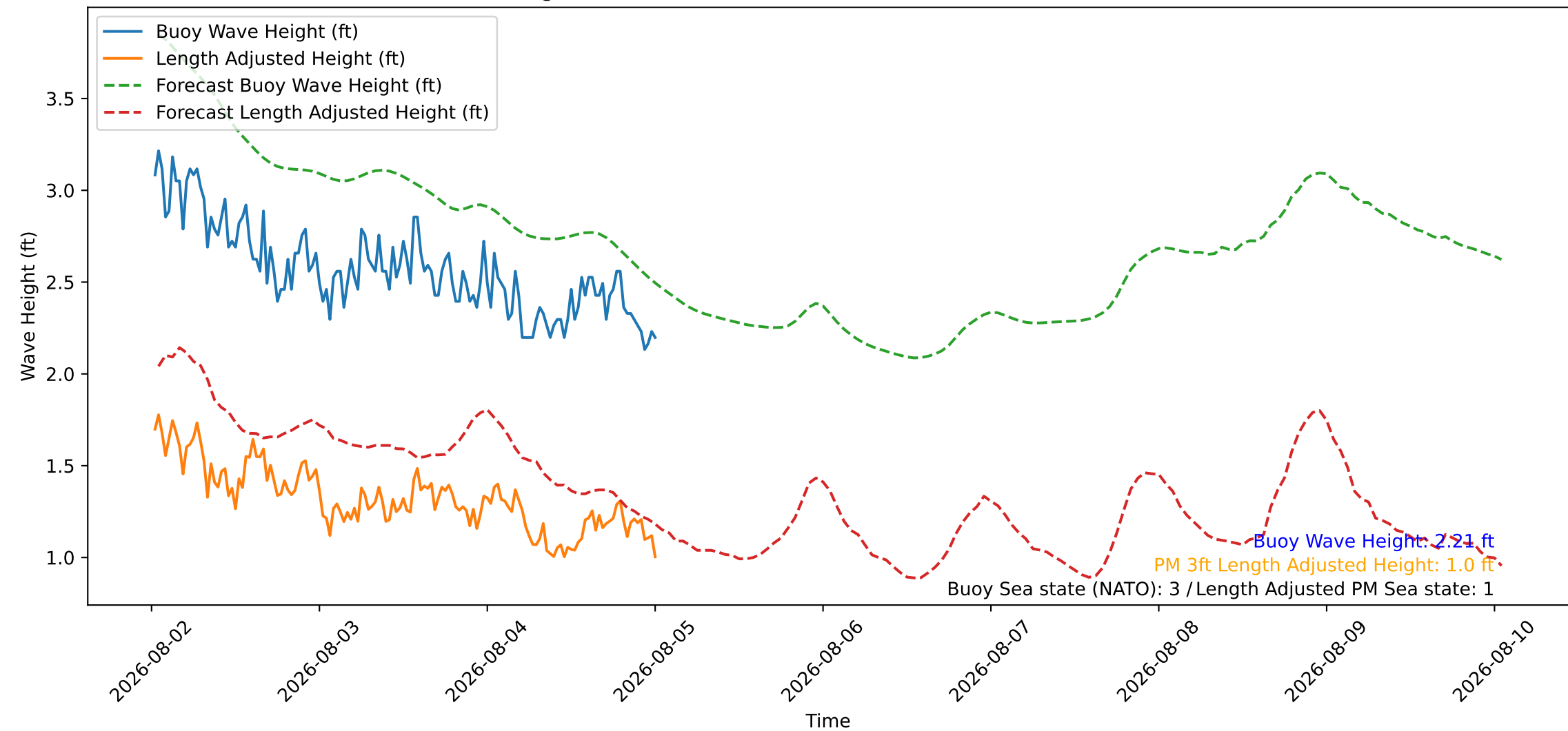
Wave Heights over Time for Oceanside Harbor at 2026-08-05 00:40:26
