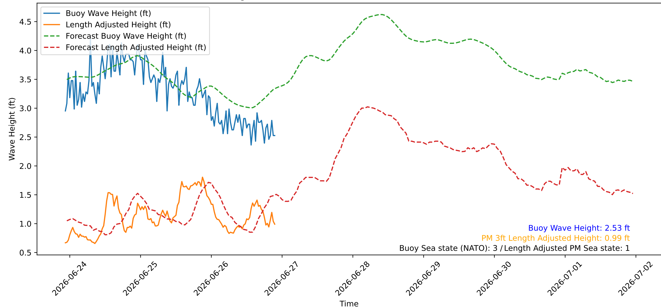
Wave Heights over Time for Green Beach at 2026-06-26 22:31:09
