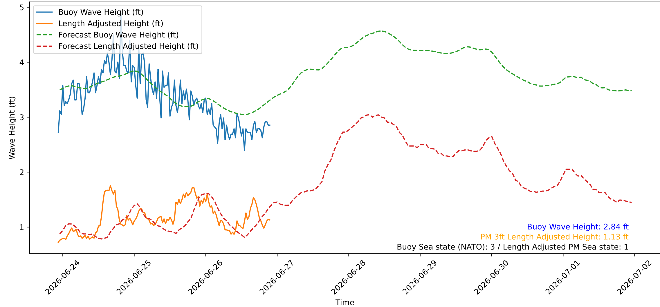
Wave Heights over Time for Oceanside Harbor at 2026-06-26 22:30:27
