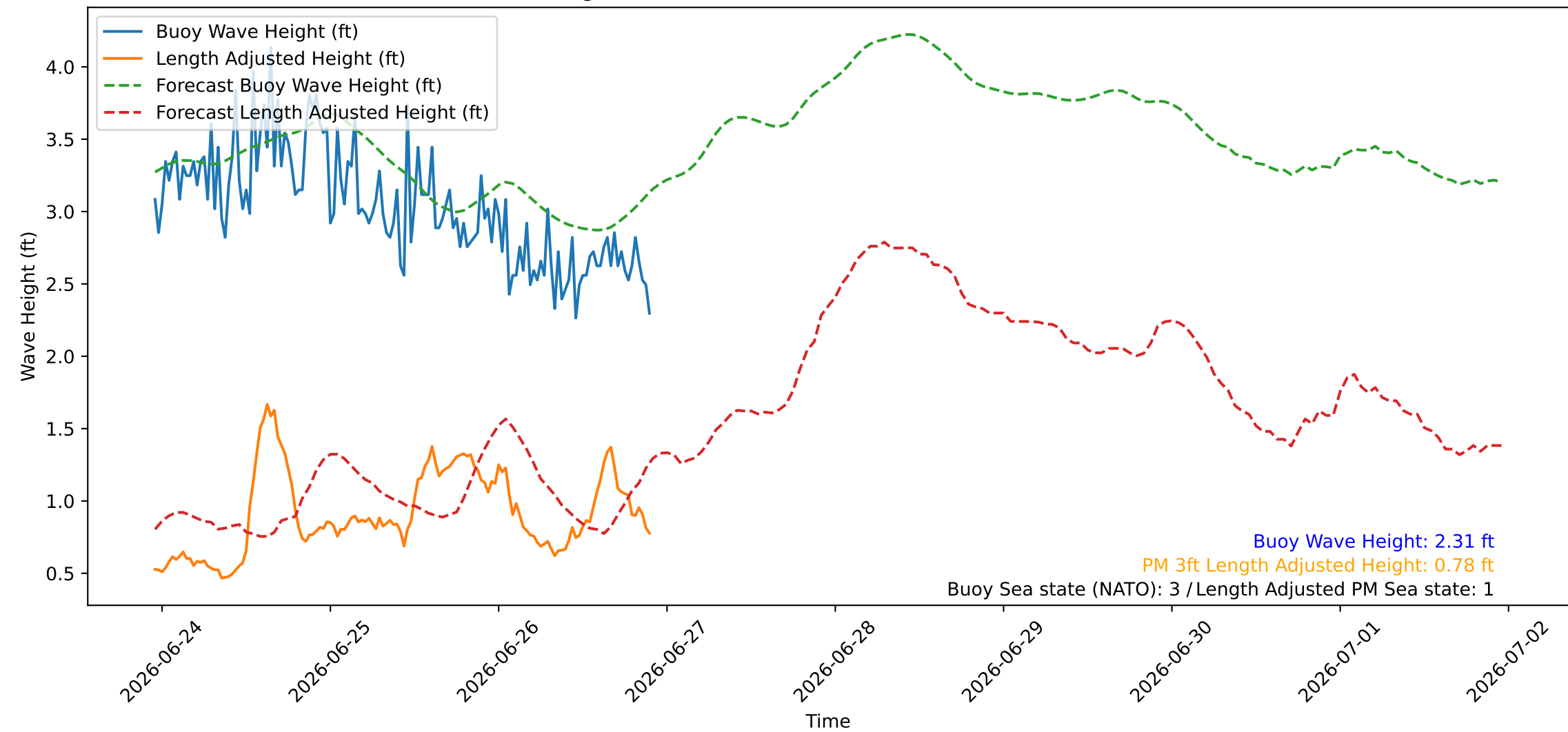
Wave Heights over Time for Red Beach at 2026-06-26 22:30:46
