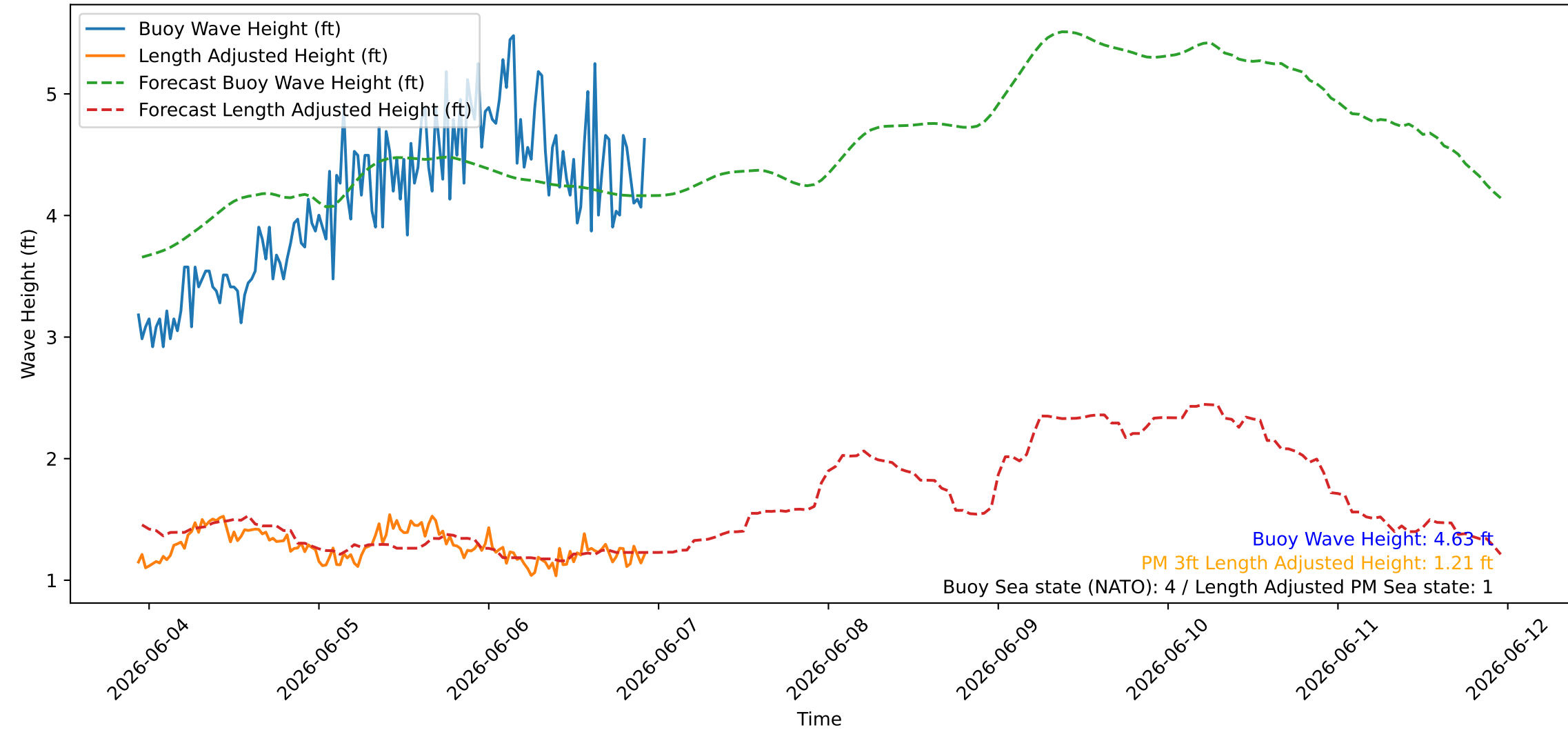
Wave Heights over Time for Oceanside Harbor at 2026-06-06 22:40:25
