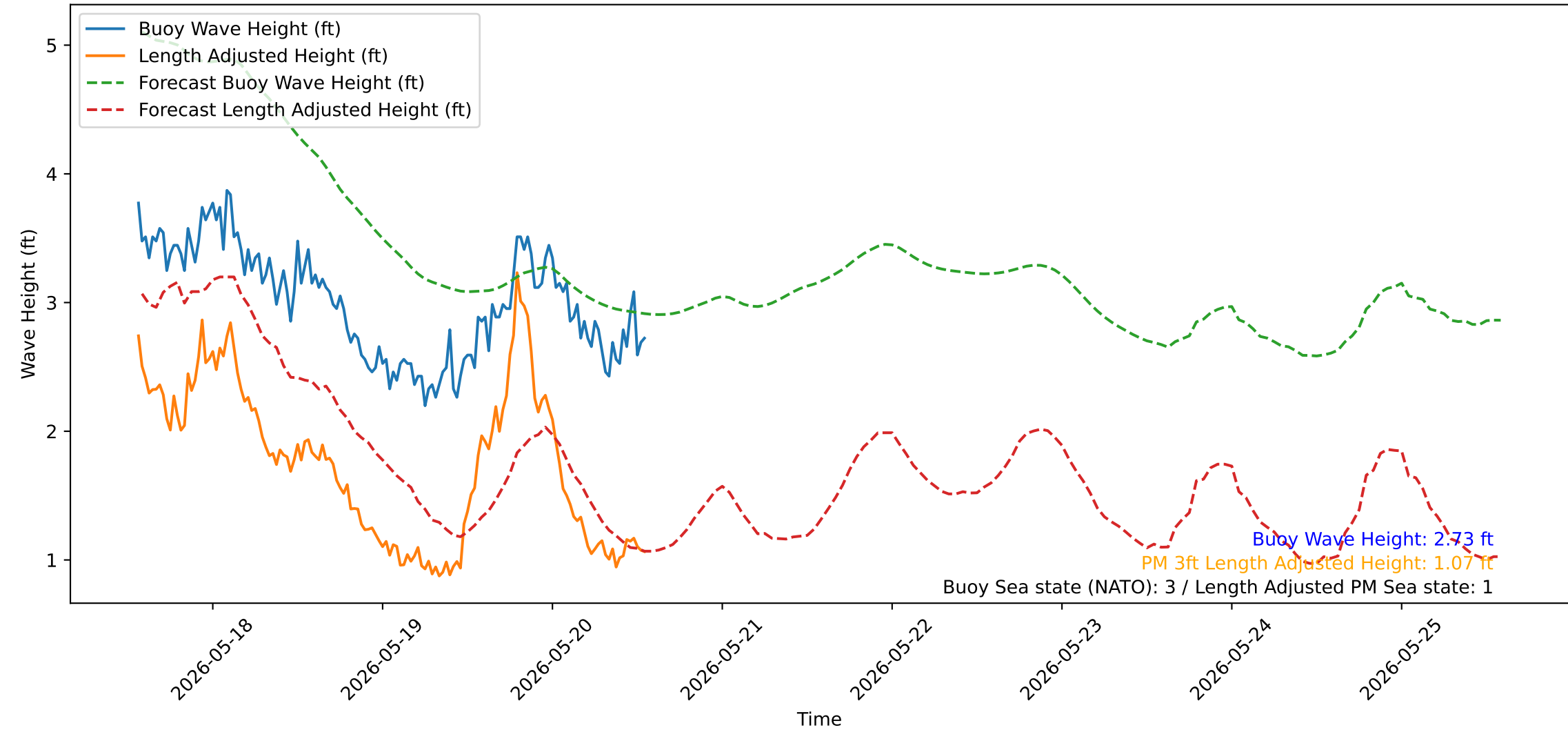
Wave Heights over Time for Oceanside Harbor at 2026-05-20 13:30:31
