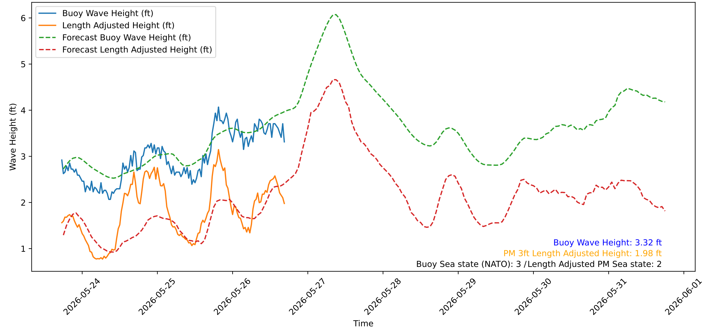
Wave Heights over Time for Green Beach at 2026-05-26 17:31:09
