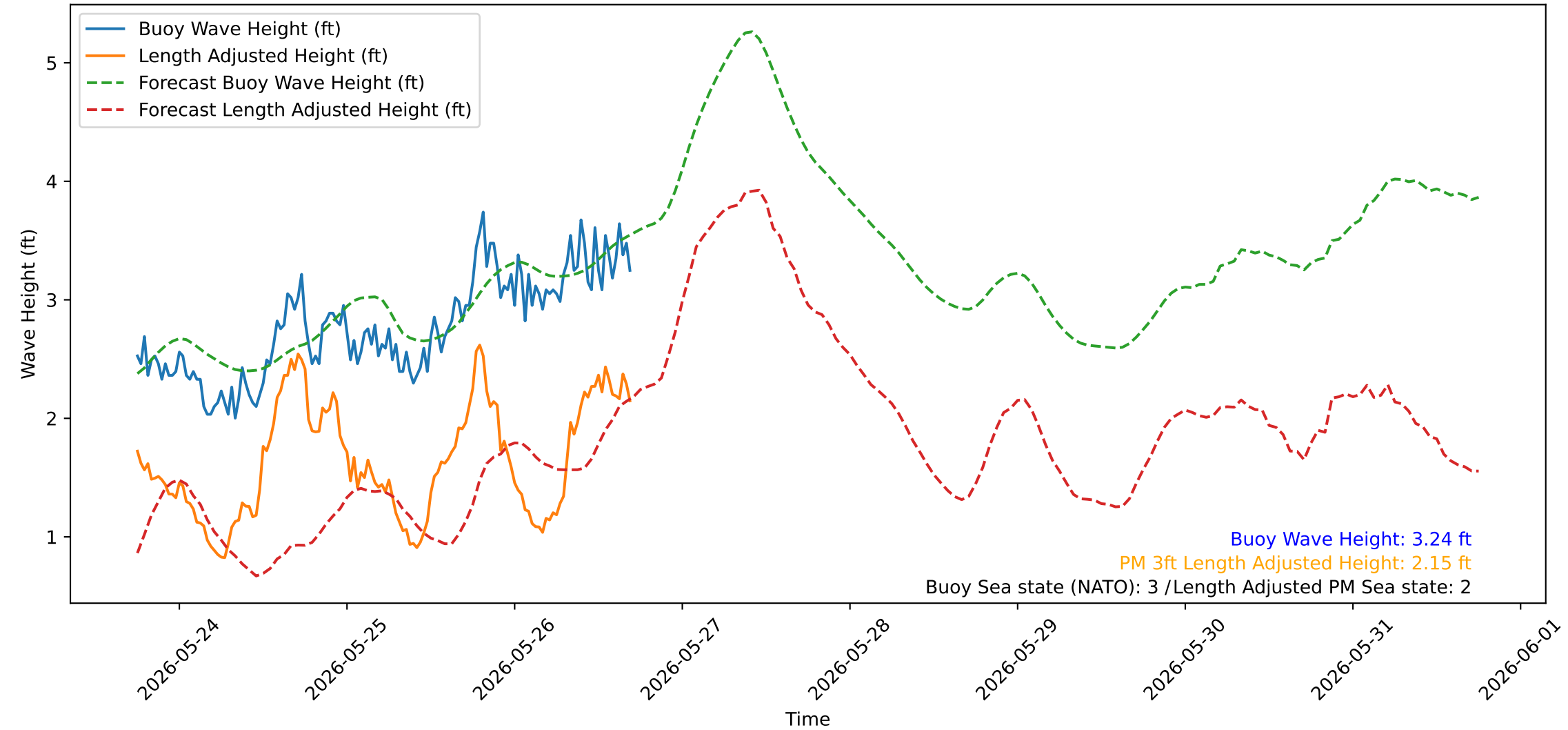
Wave Heights over Time for Red Beach at 2026-05-26 17:30:46
