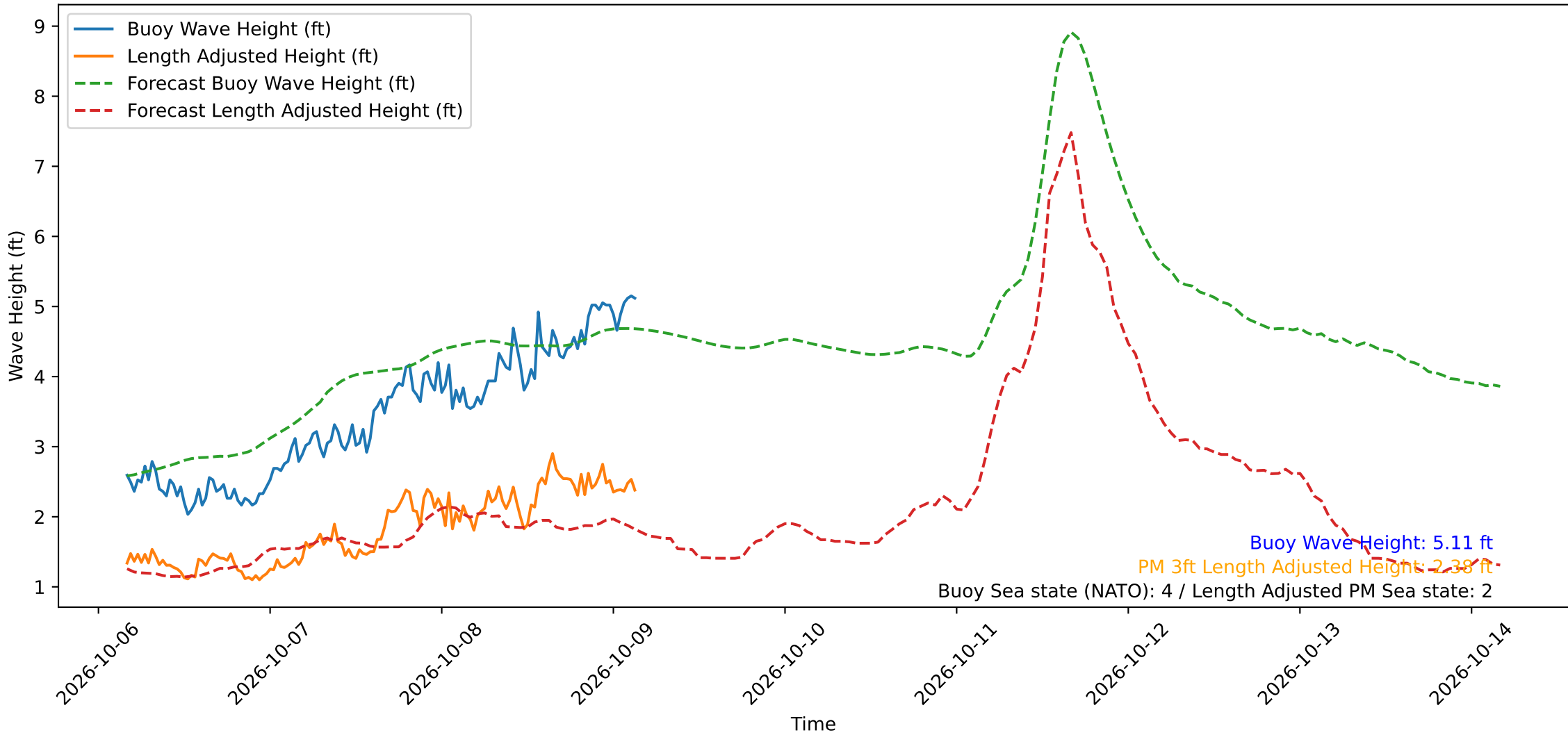
Wave Heights over Time for Oceanside Harbor at 2026-10-09 04:00:30
