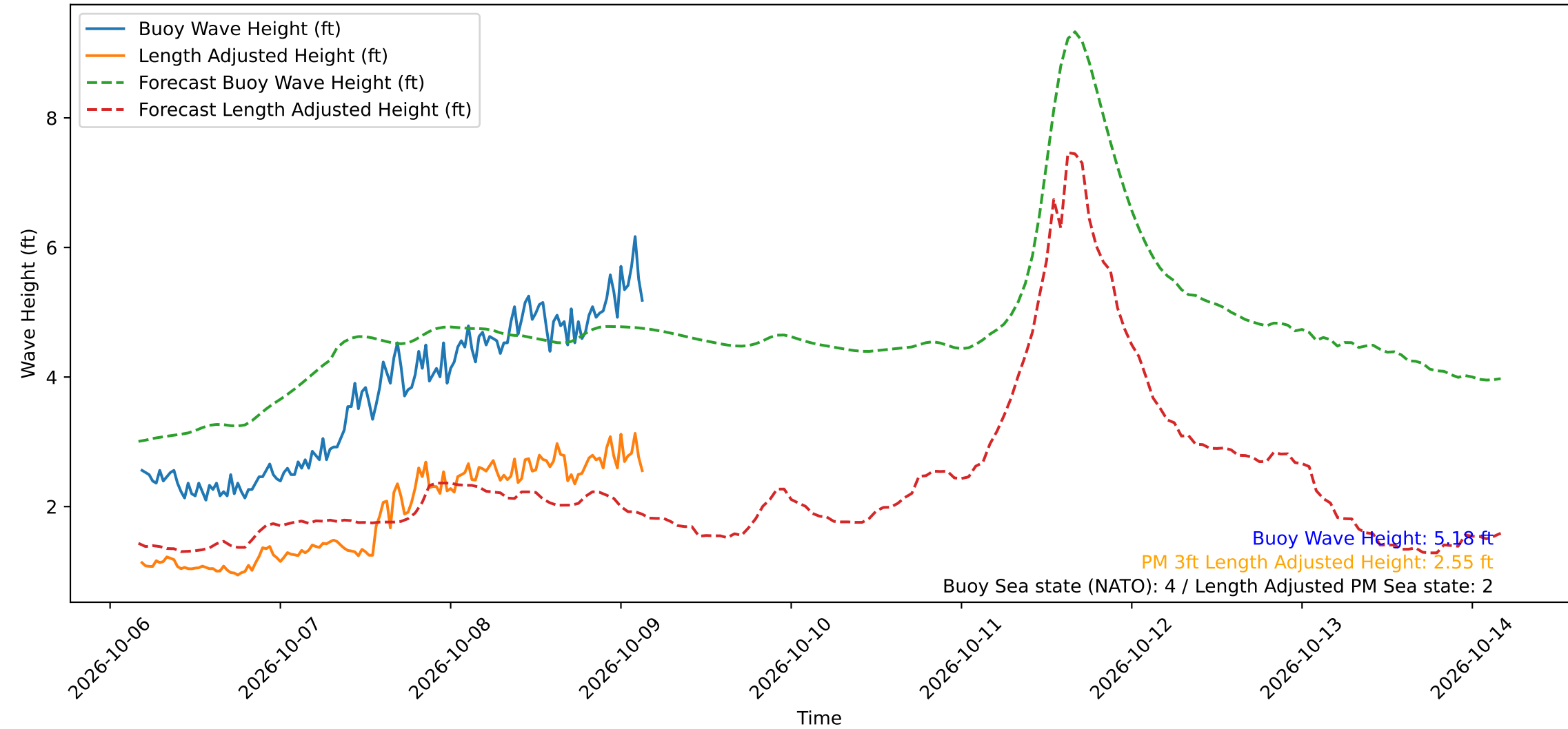
Wave Heights over Time for Green Beach at 2026-10-09 04:01:12
