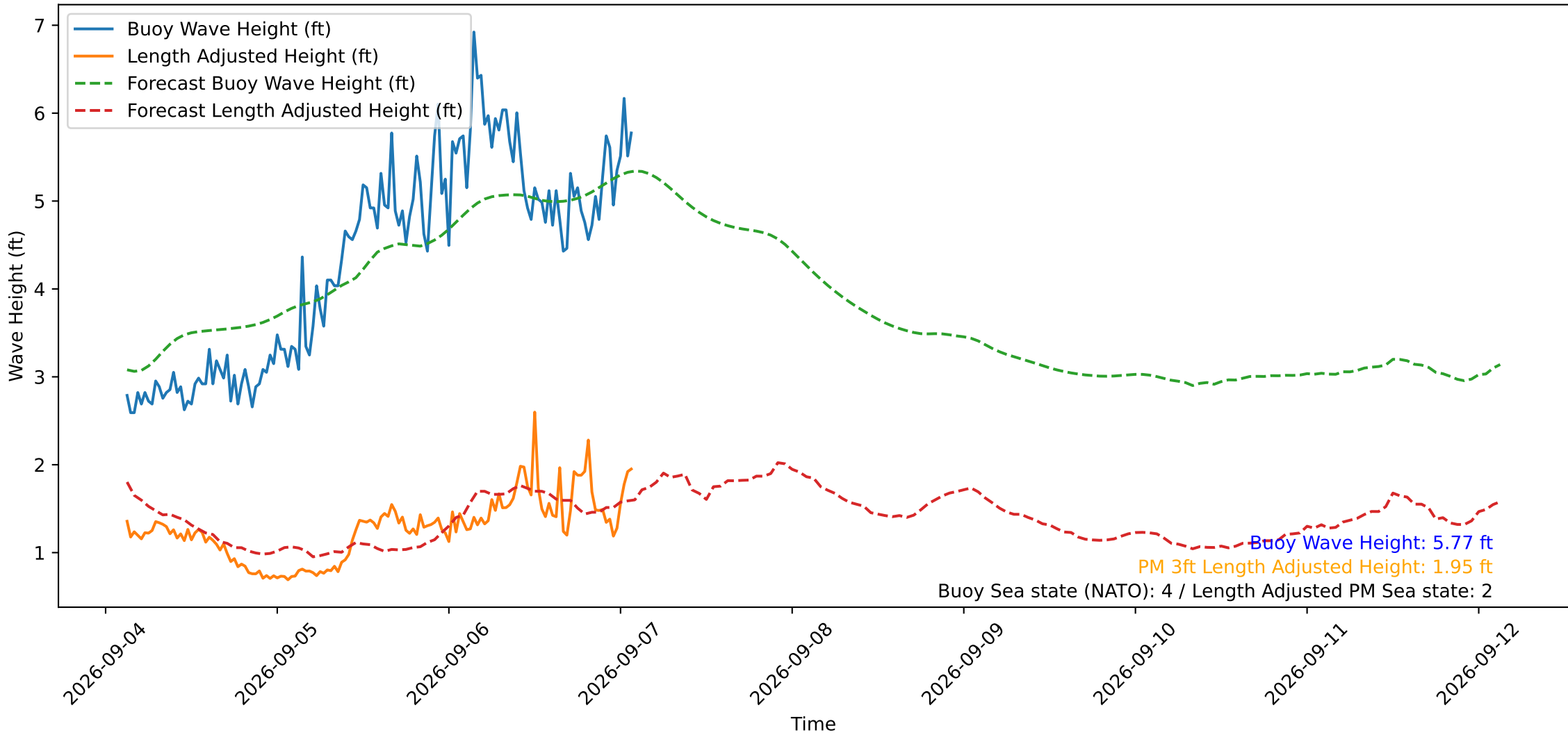
Wave Heights over Time for Red Beach at 2026-09-07 02:30:49
