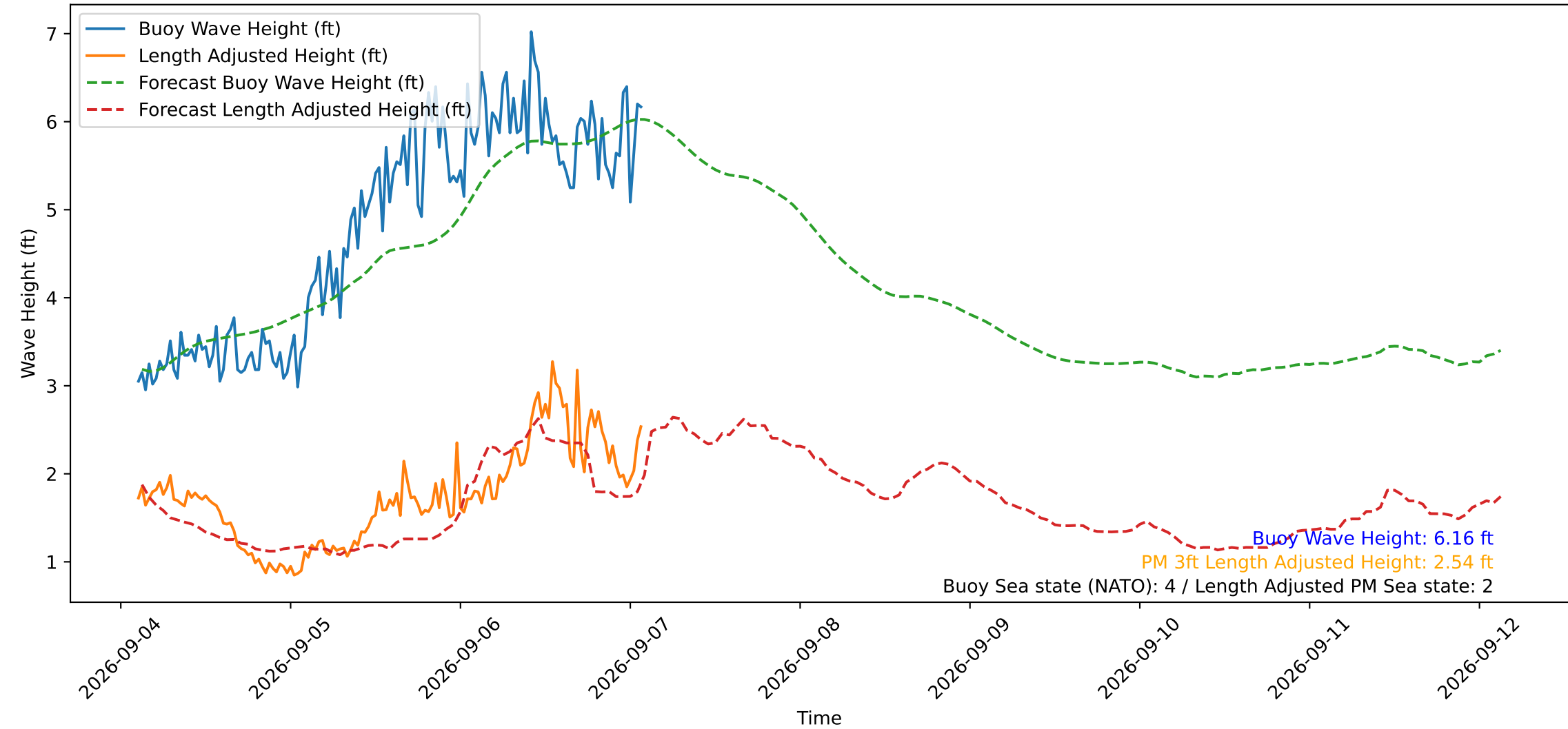
Wave Heights over Time for Oceanside Harbor at 2026-09-07 02:30:30
