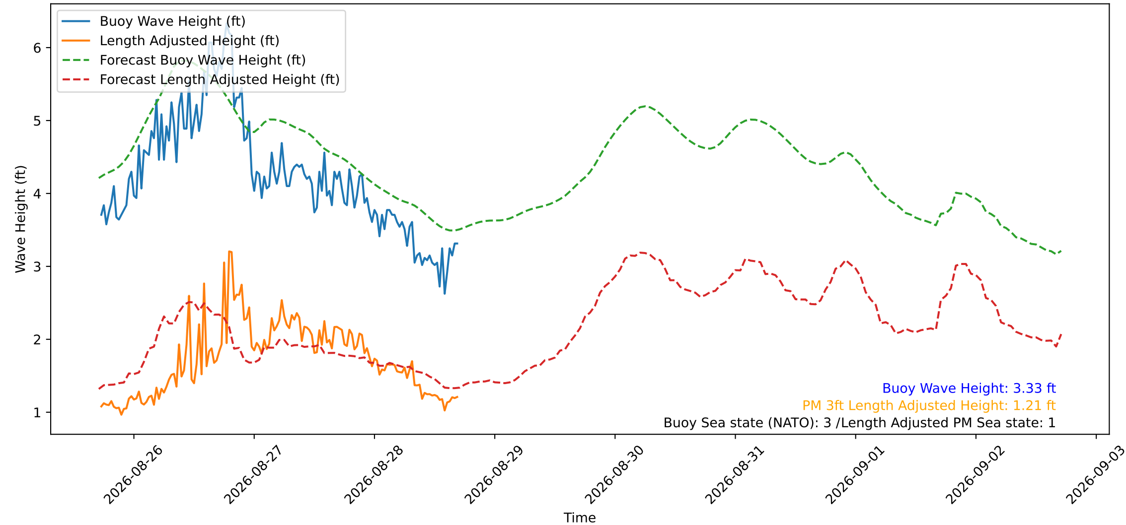
Wave Heights over Time for Green Beach at 2026-08-28 17:21:15
