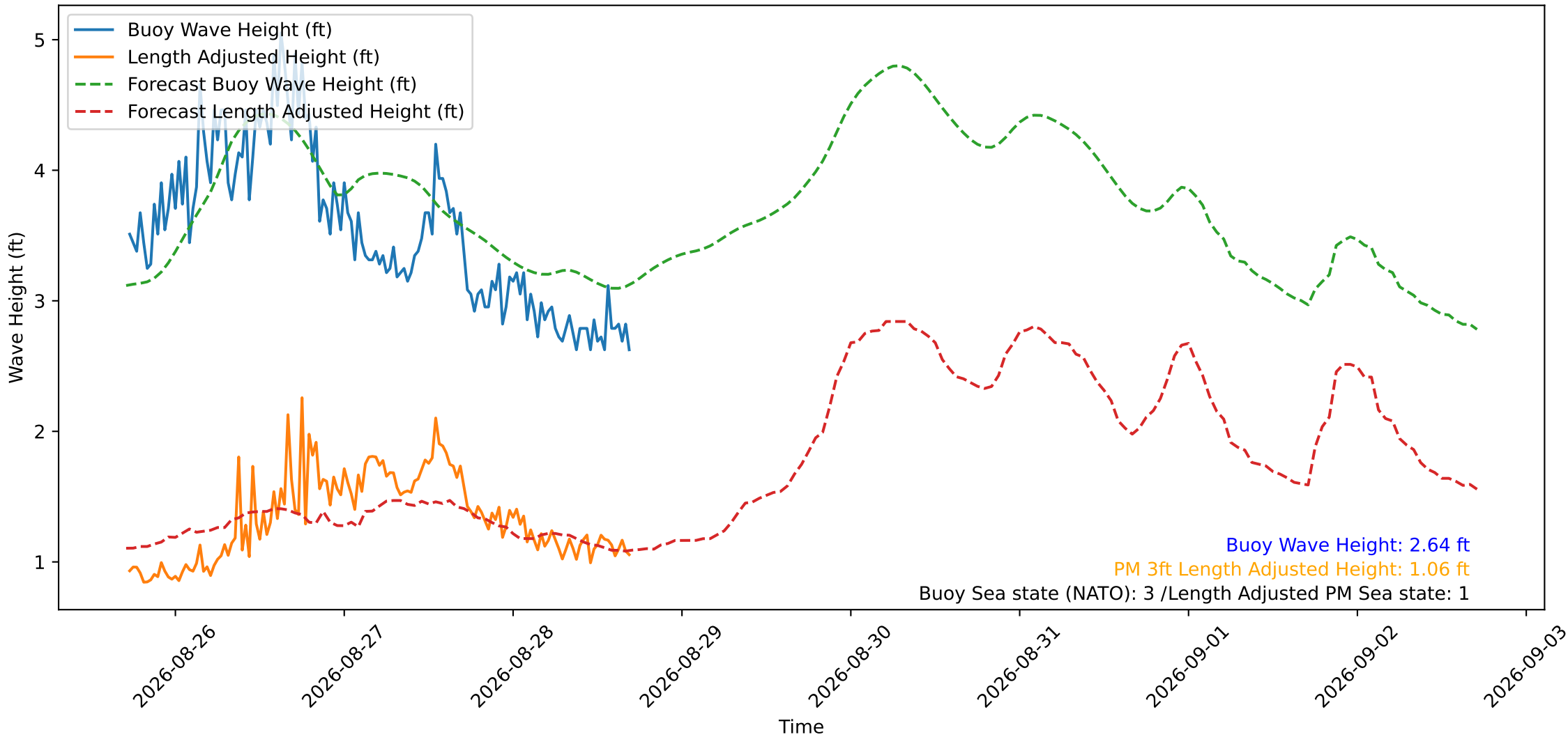
Wave Heights over Time for Red Beach at 2026-08-28 17:20:51
