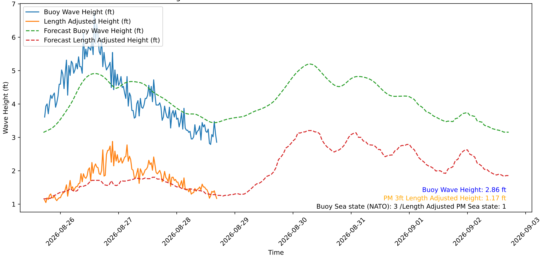
Wave Heights over Time for Oceanside Harbor at 2026-08-28 17:20:30
