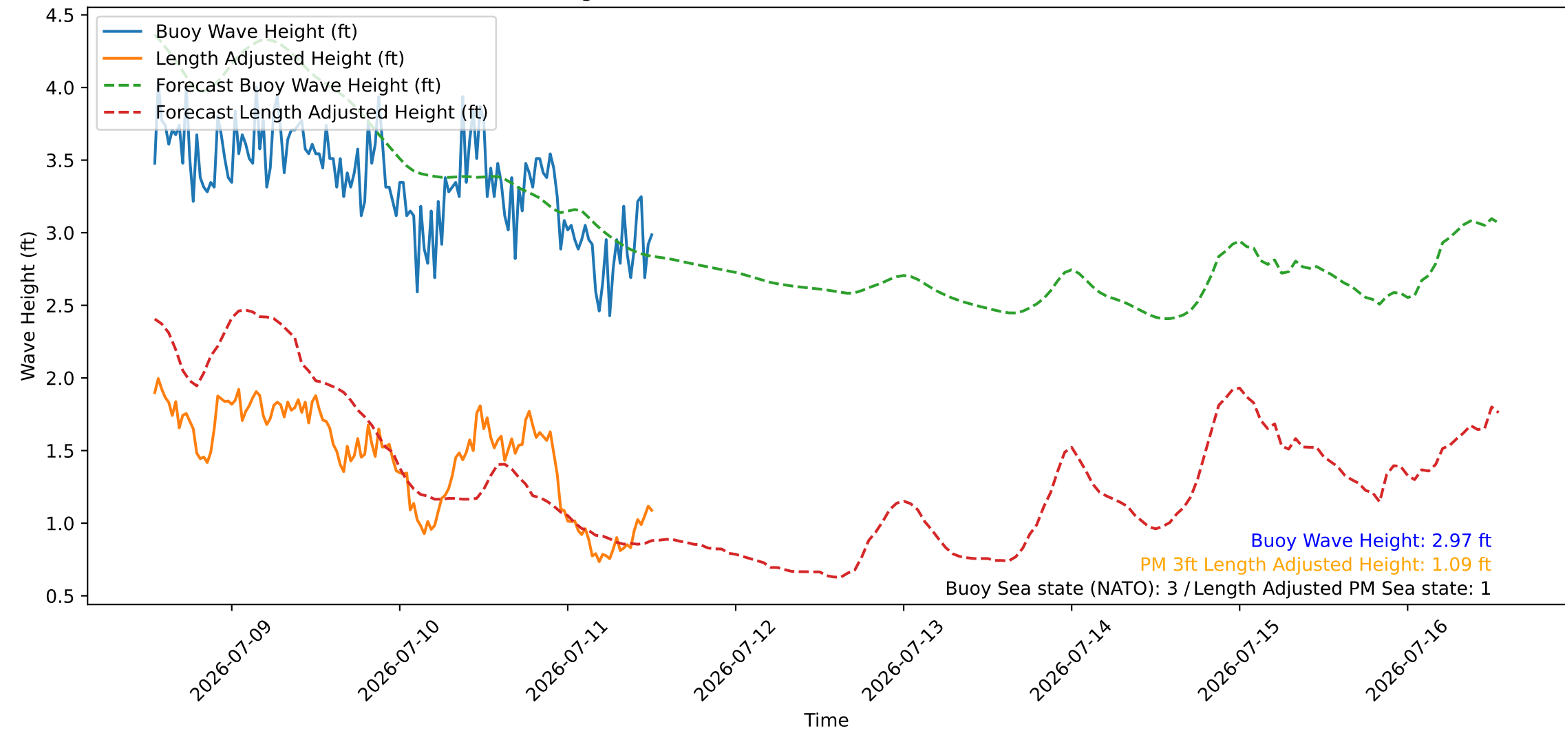
Wave Heights over Time for Red Beach at 2026-07-11 12:40:46
