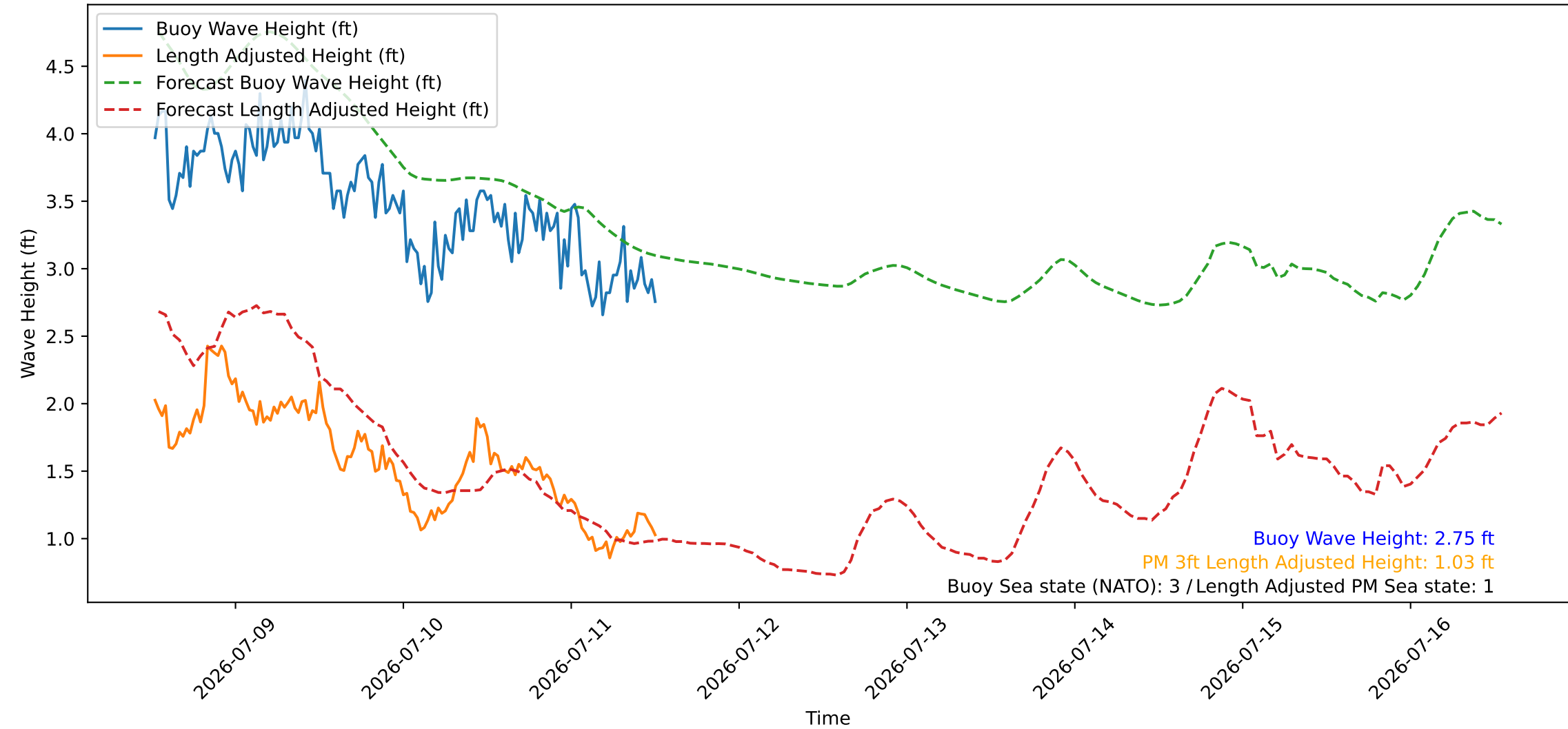
Wave Heights over Time for Green Beach at 2026-07-11 12:41:08
