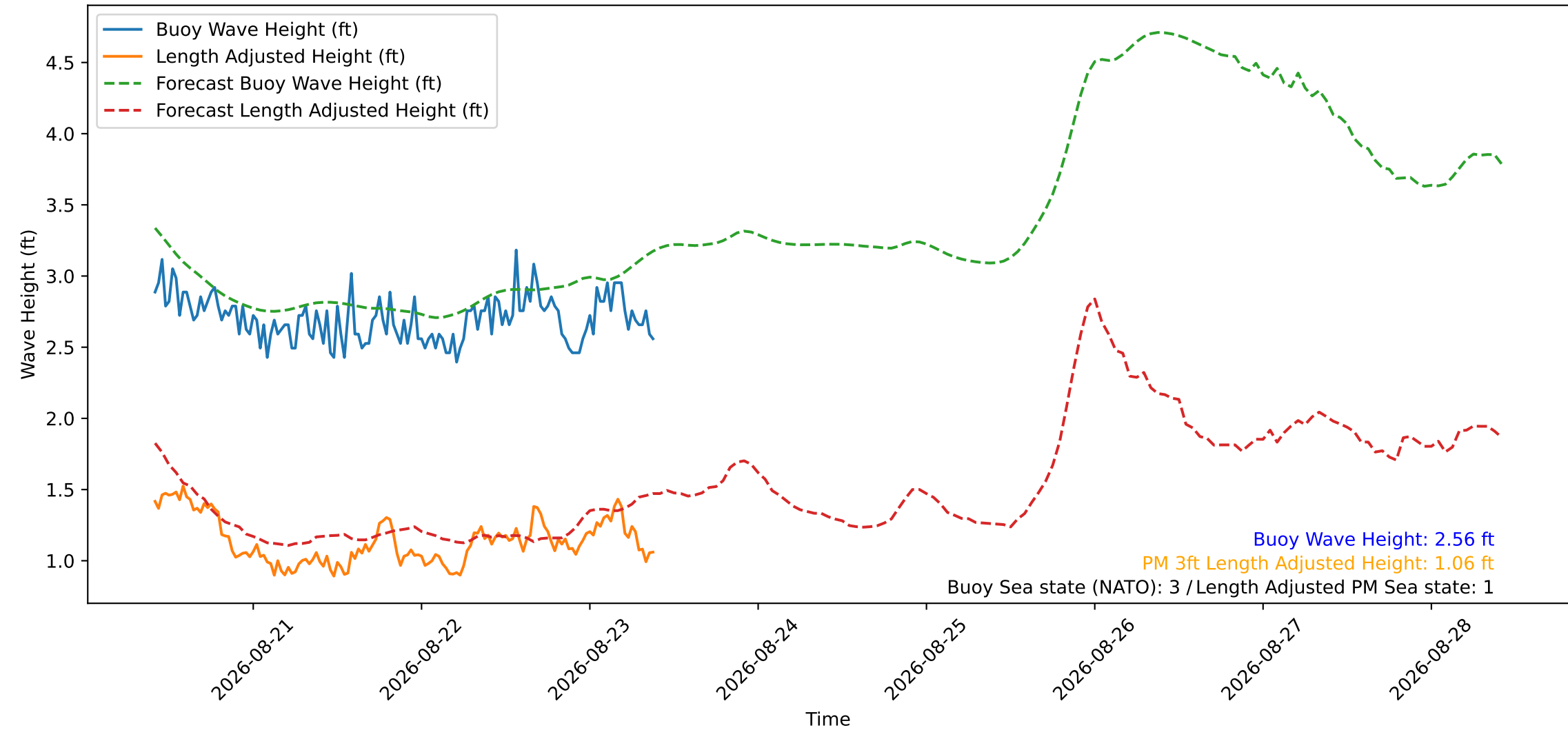
Wave Heights over Time for Green Beach at 2026-08-23 09:51:14
