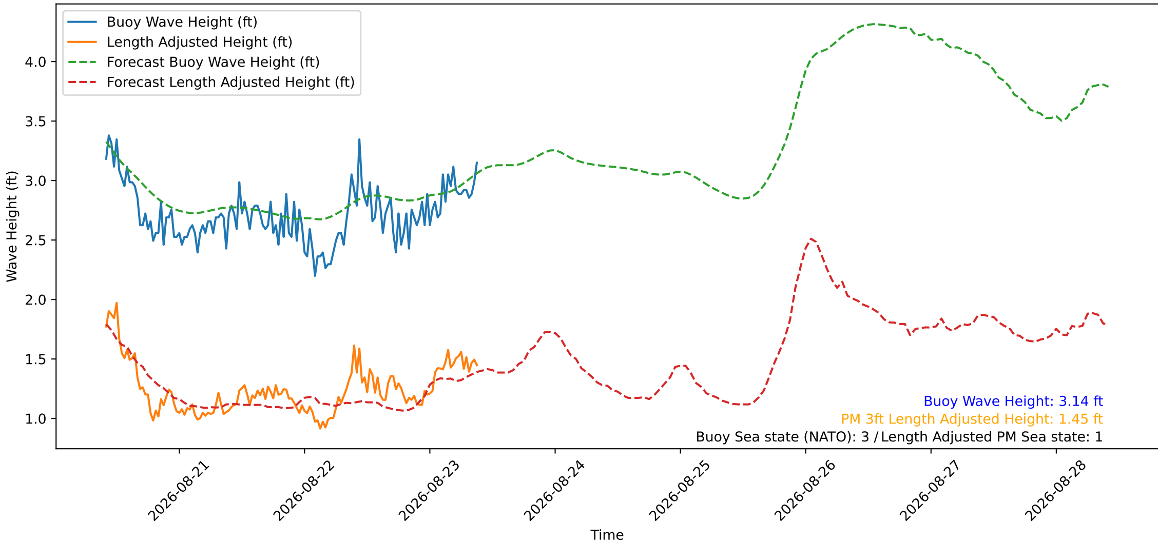
Wave Heights over Time for Oceanside Harbor at 2026-08-23 09:50:29
