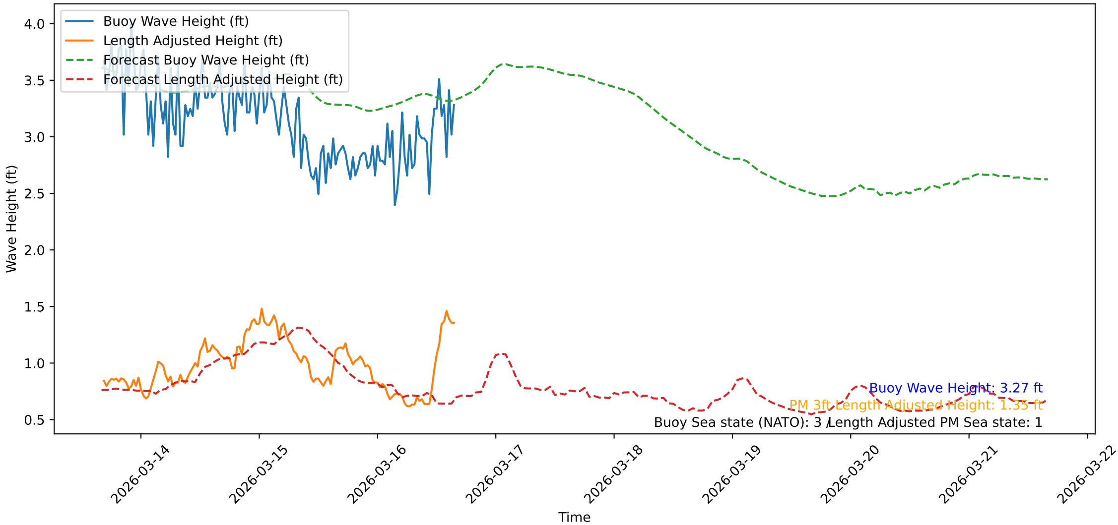
Wave Heights over Time for Oceanside Harbor at 2026-03-16 16:20:45
