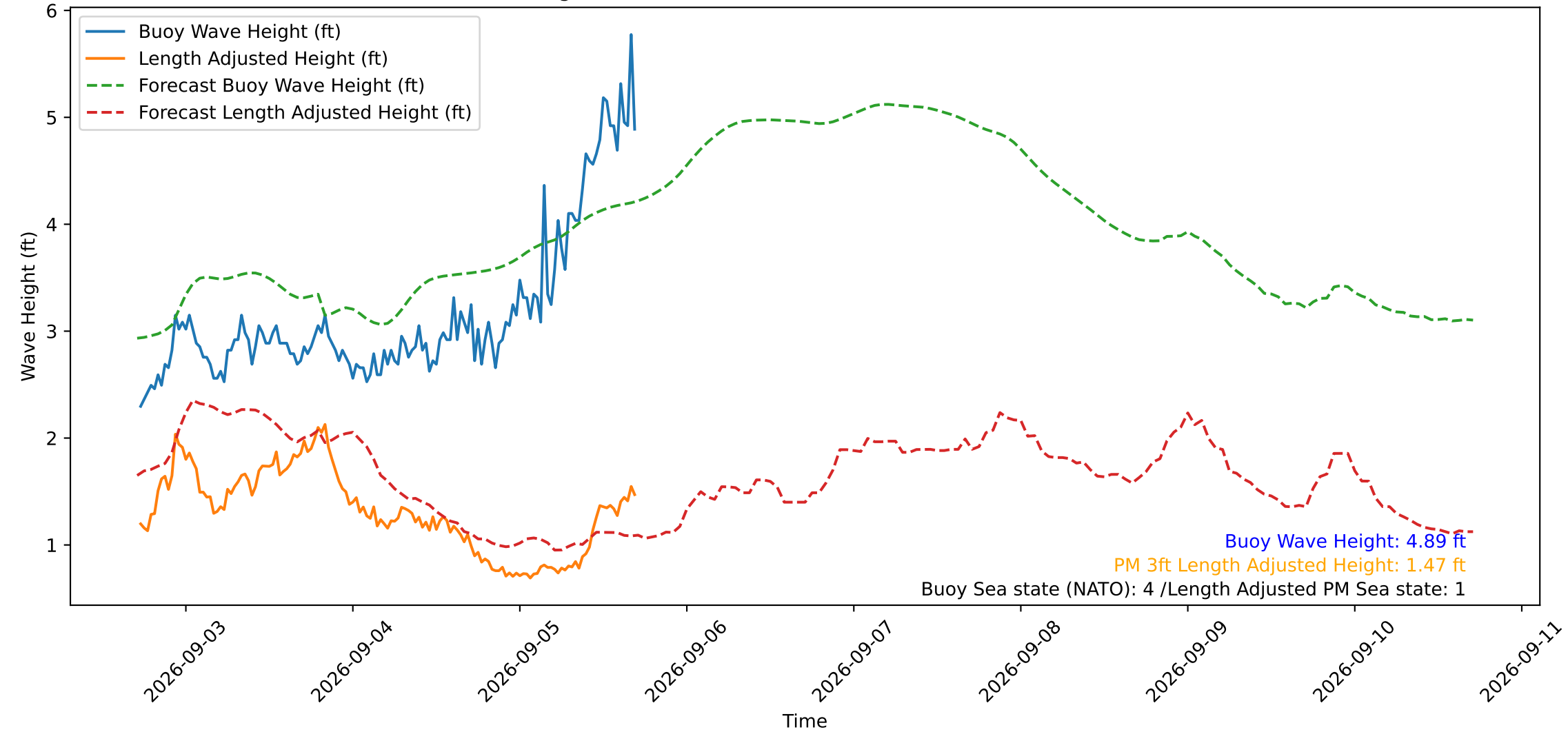
Wave Heights over Time for Red Beach at 2026-09-05 17:20:51
