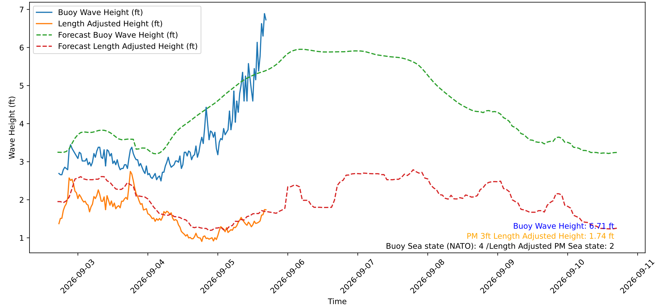
Wave Heights over Time for Green Beach at 2026-09-05 17:21:15
