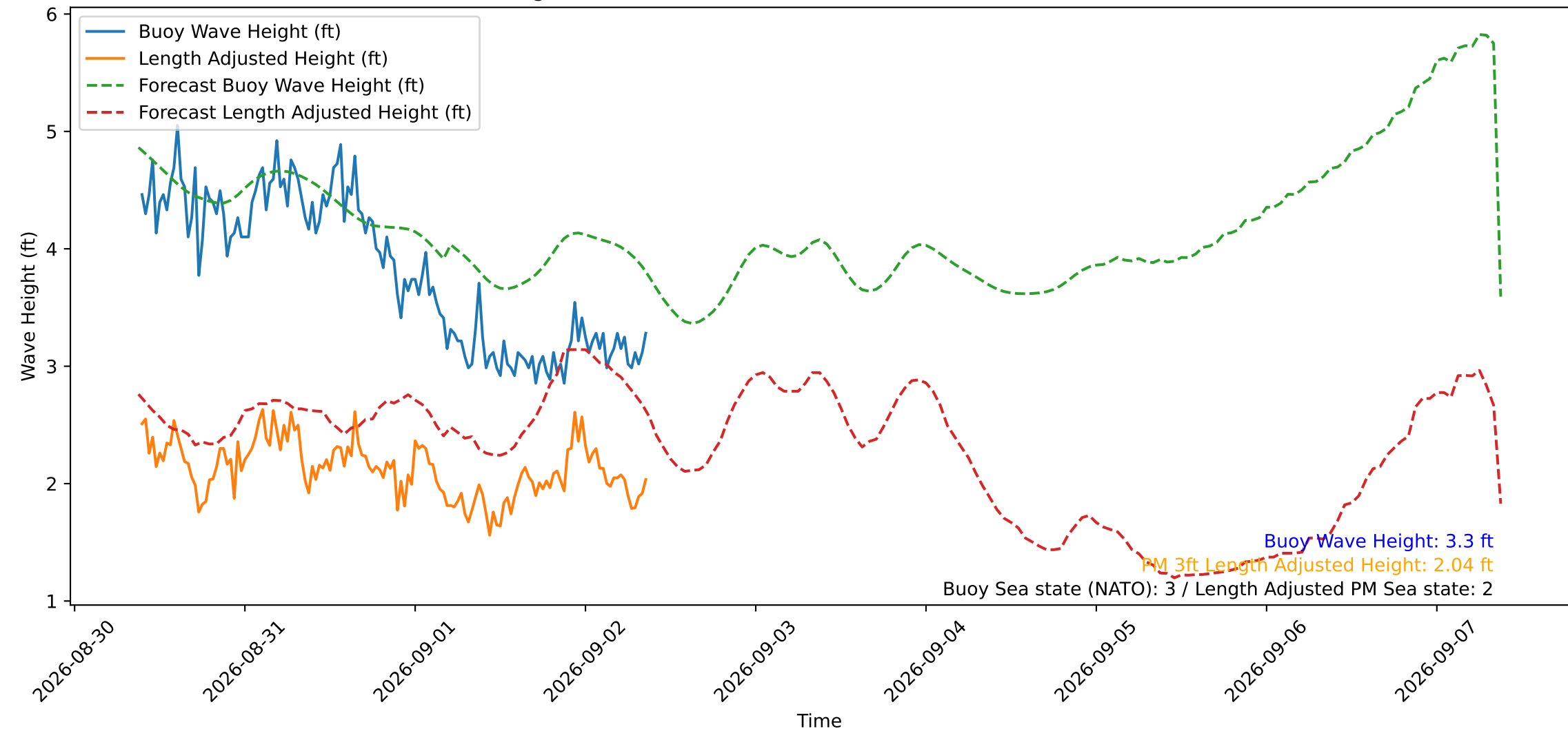
Wave Heights over Time for Oceanside Harbor at 2026-09-02 09:20:29
