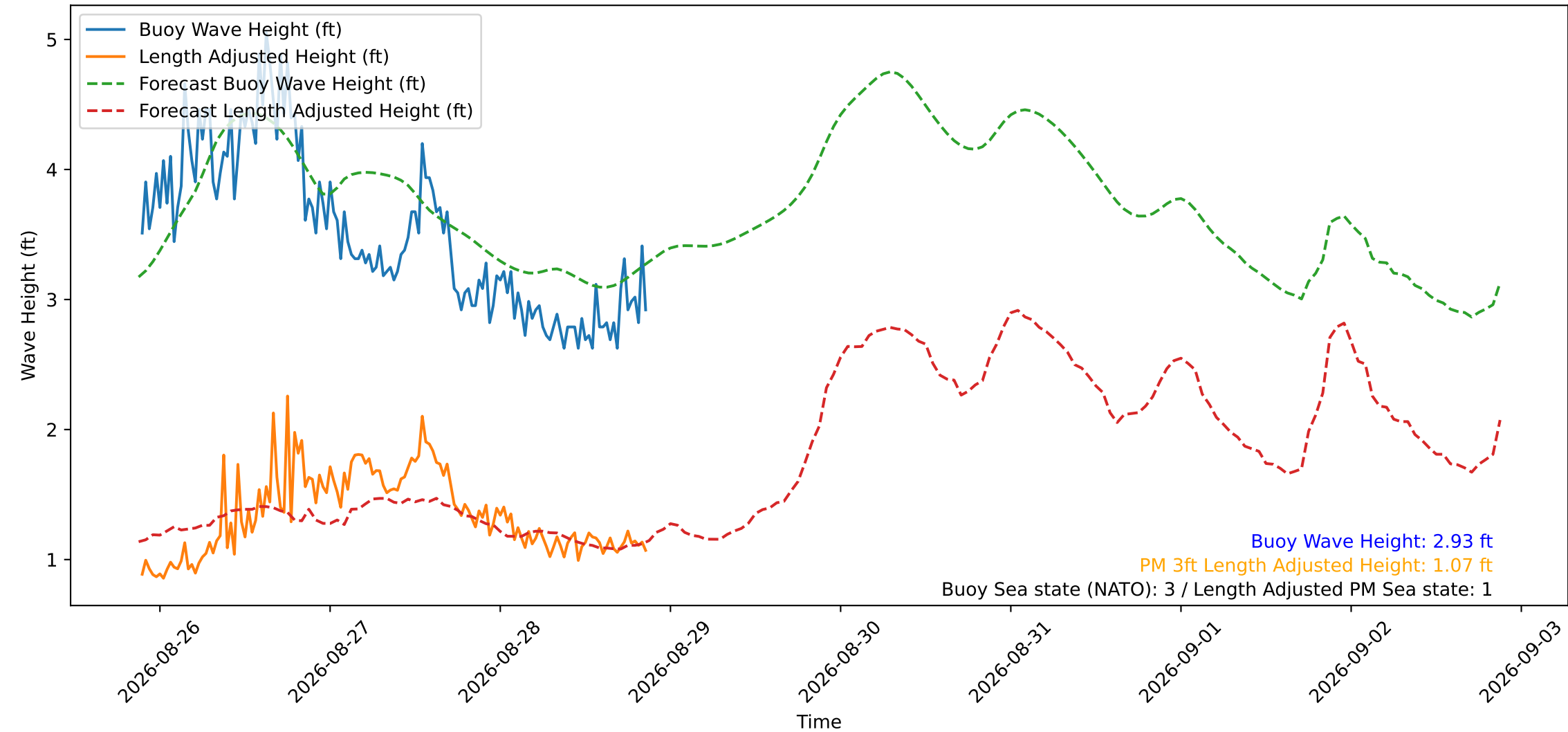
Wave Heights over Time for Red Beach at 2026-08-28 21:20:51
