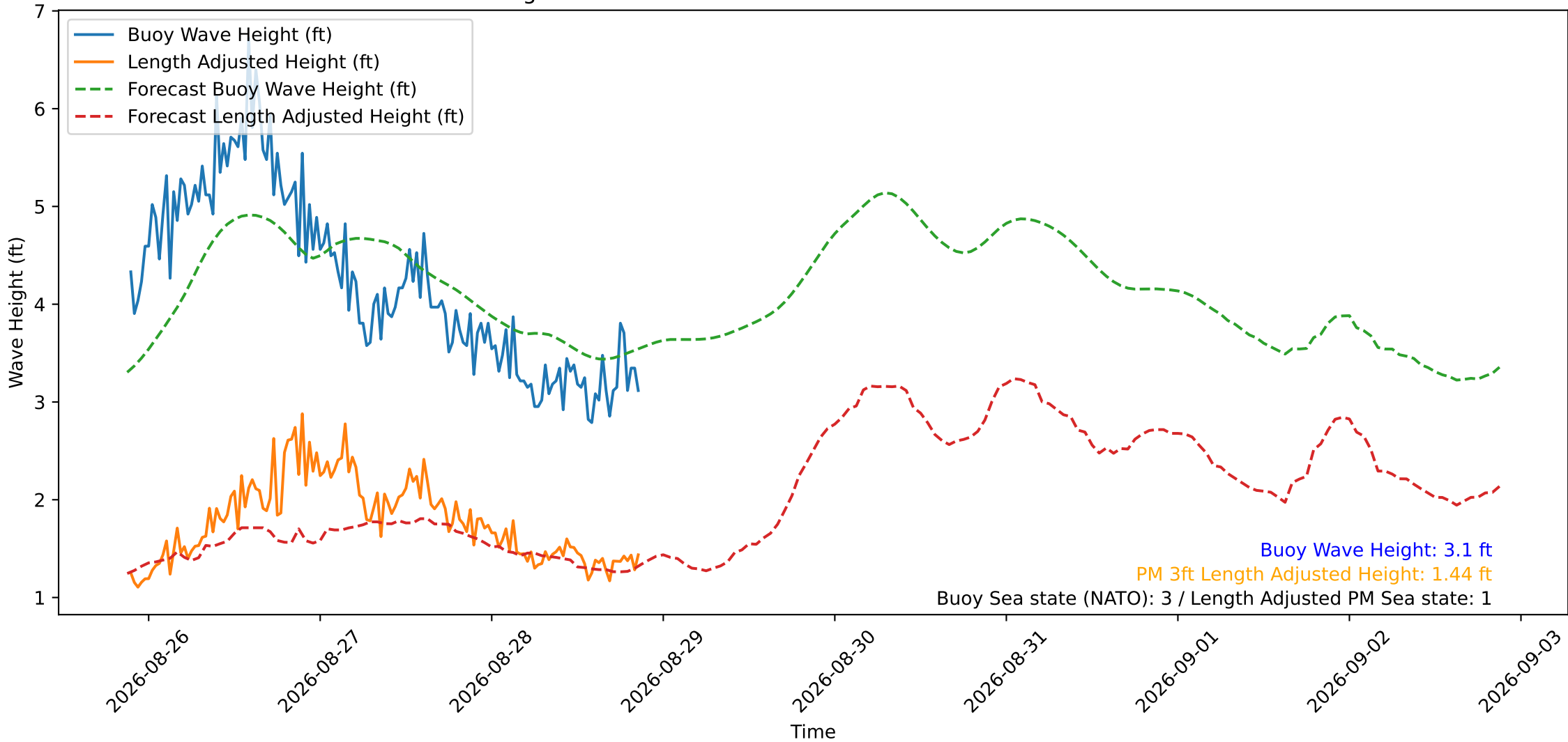
Wave Heights over Time for Oceanside Harbor at 2026-08-28 21:20:30
