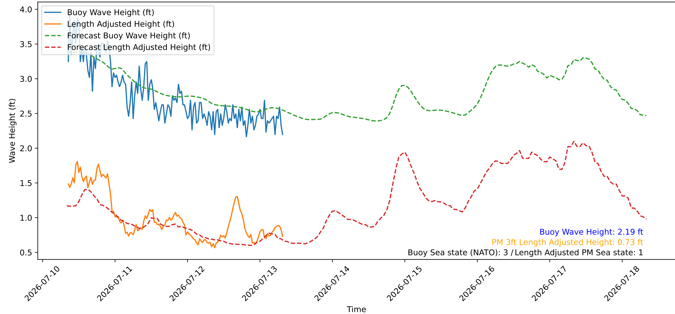
Wave Heights over Time for Red Beach at 2026-07-13 08:20:47
