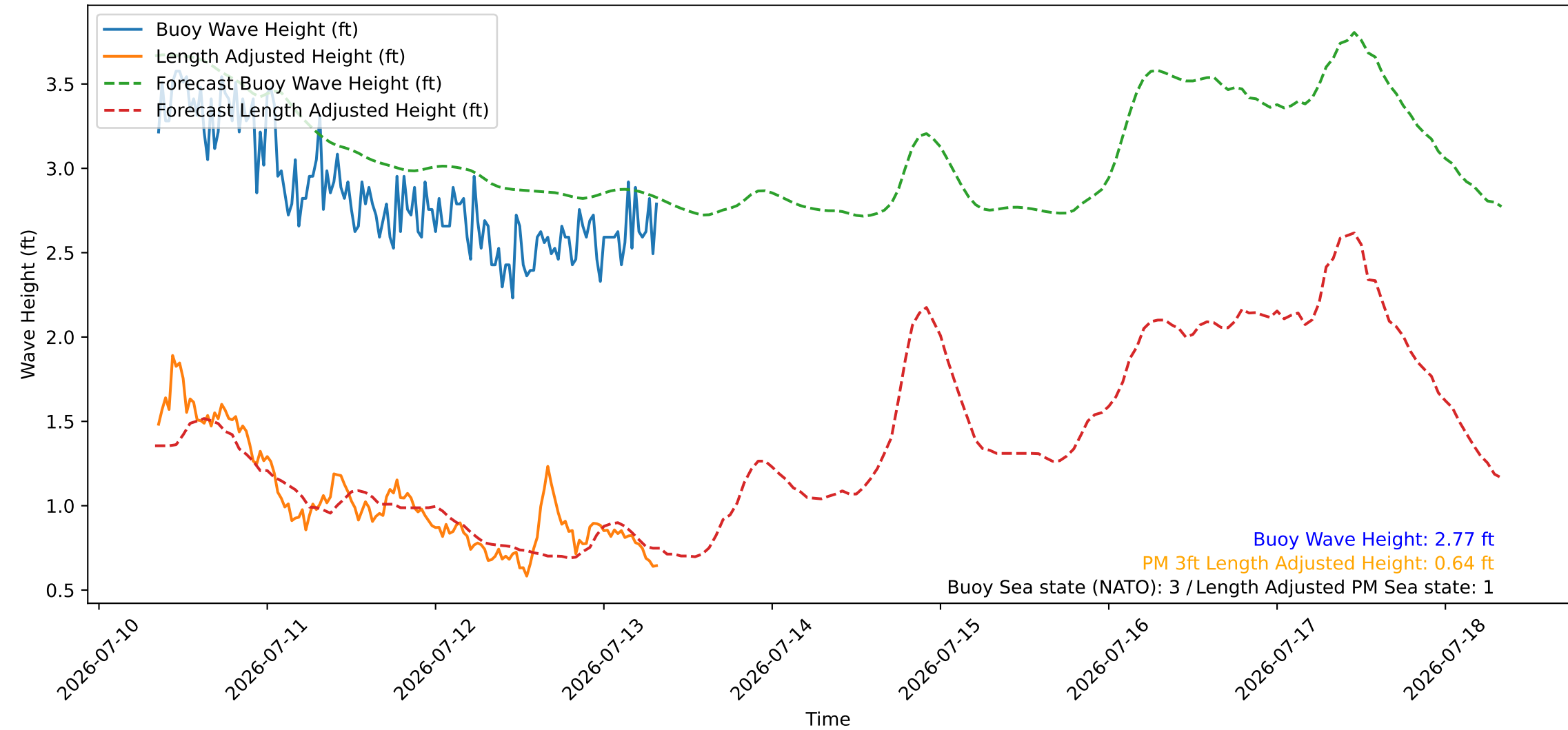
Wave Heights over Time for Green Beach at 2026-07-13 08:21:09
