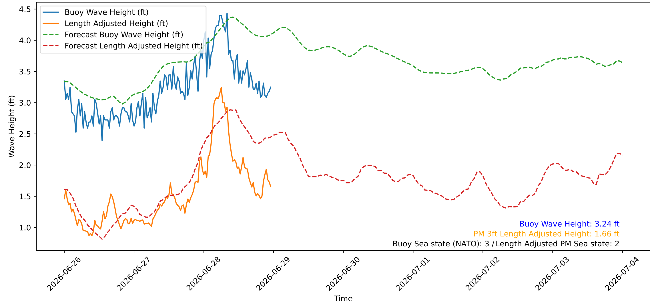
Wave Heights over Time for Oceanside Harbor at 2026-06-28 23:50:26
