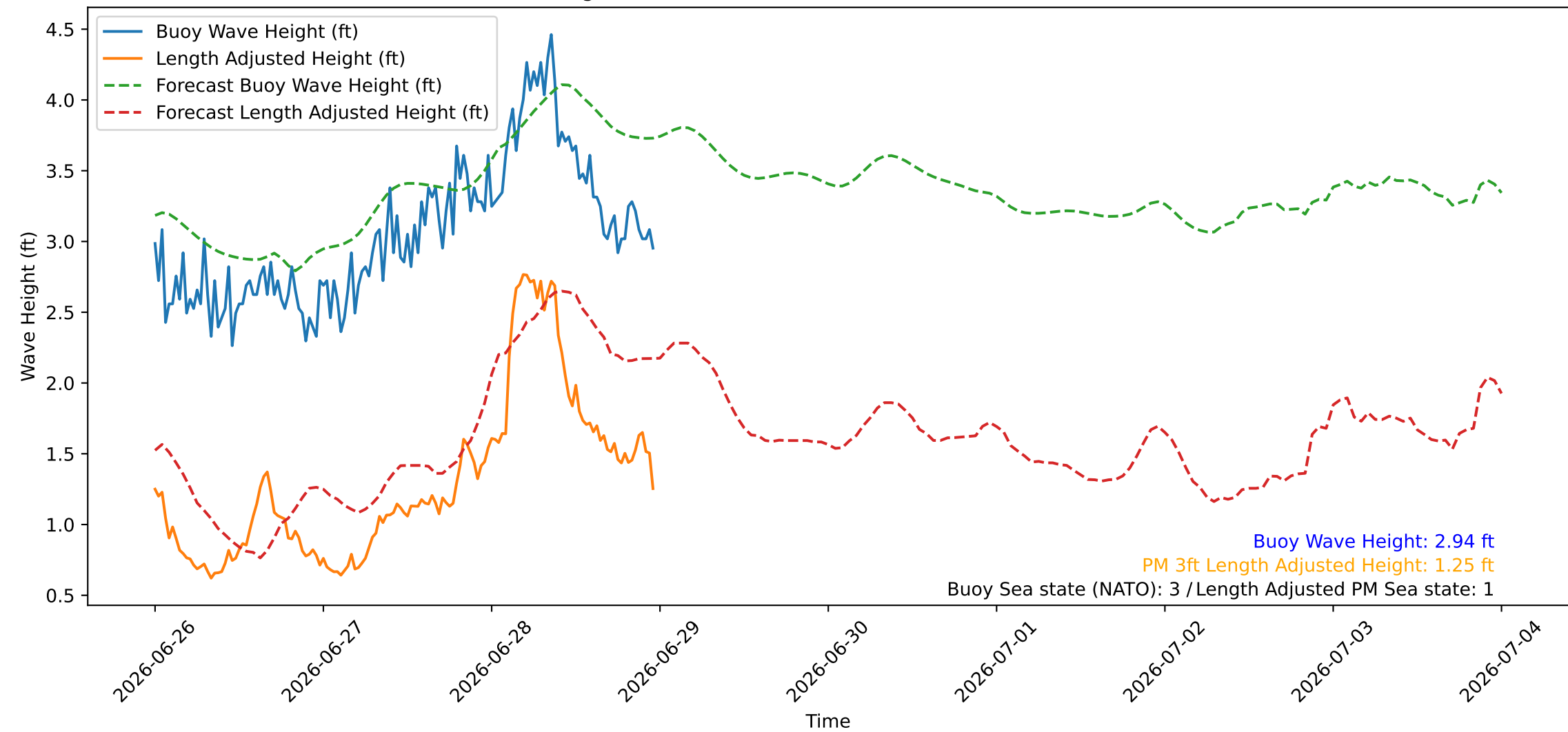
Wave Heights over Time for Red Beach at 2026-06-28 23:50:46
