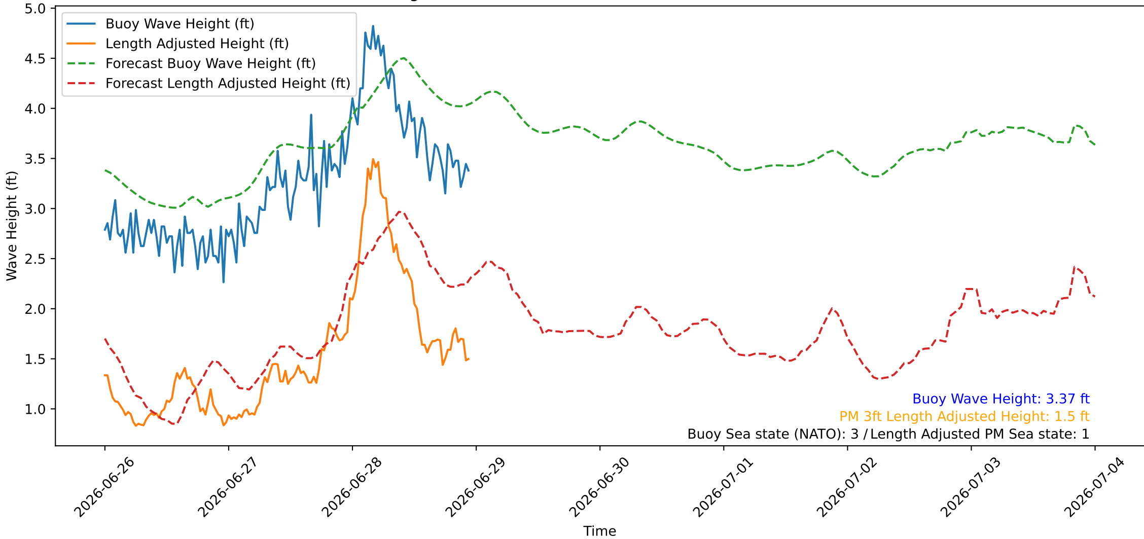
Wave Heights over Time for Green Beach at 2026-06-28 23:51:09
