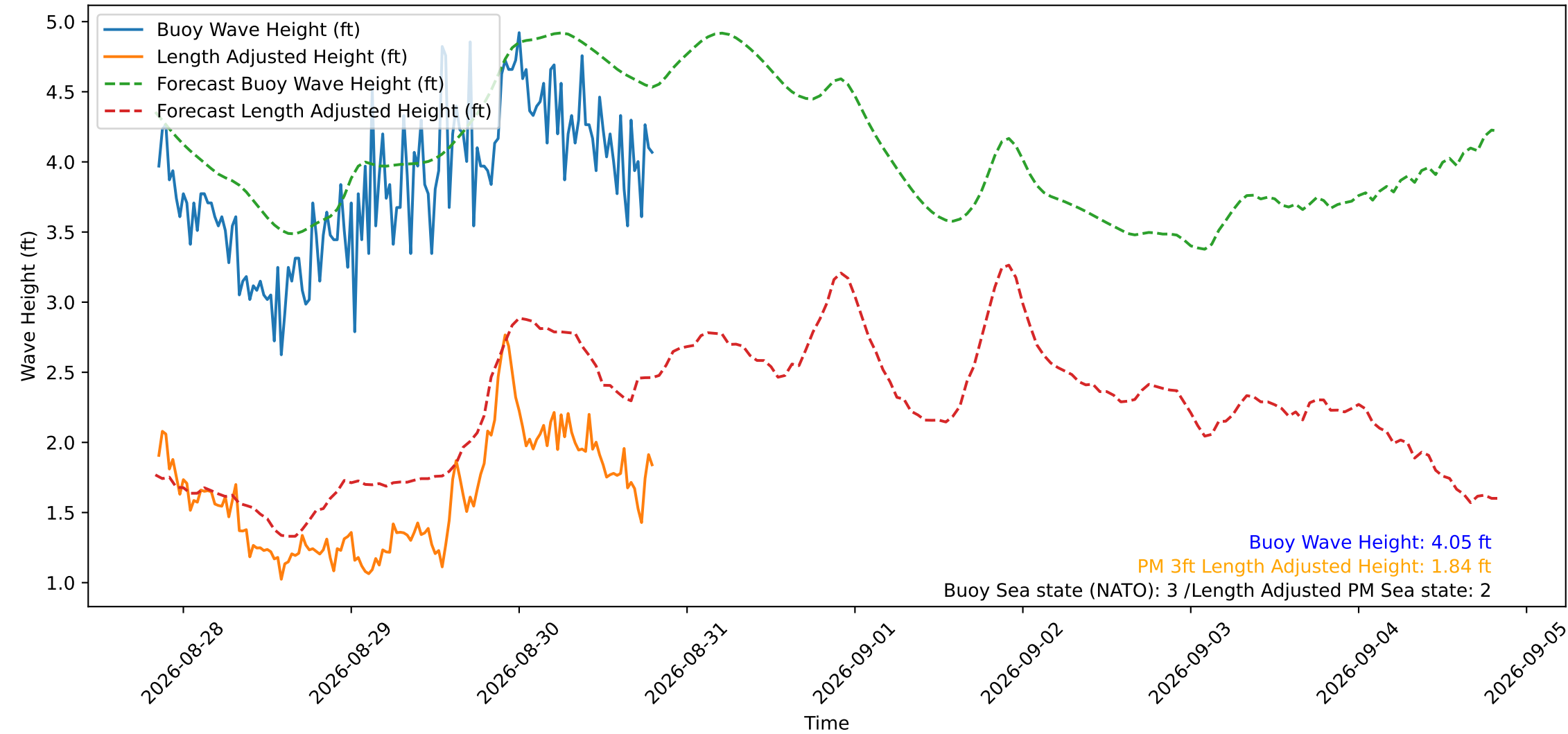
Wave Heights over Time for Green Beach at 2026-08-30 20:01:11
