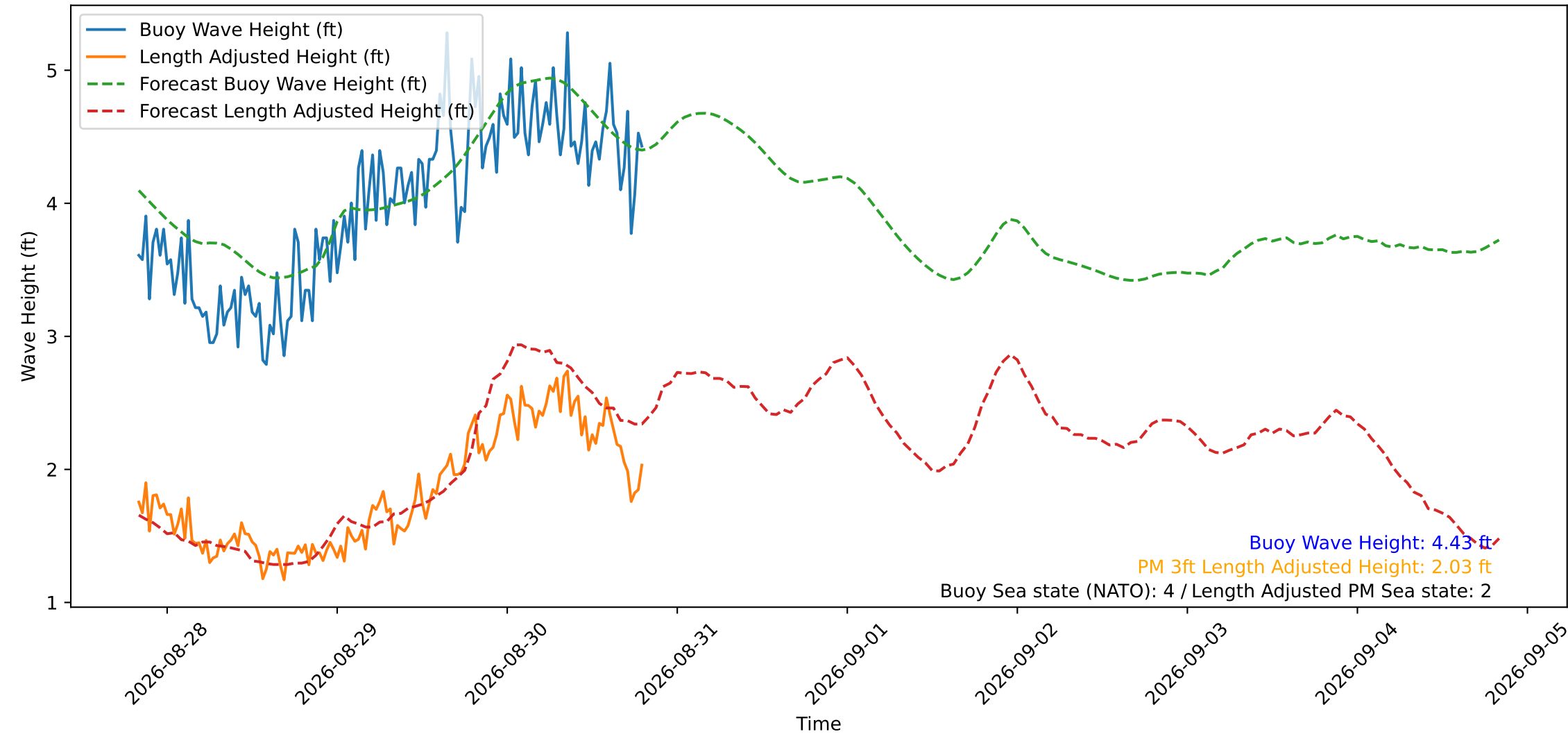
Wave Heights over Time for Oceanside Harbor at 2026-08-30 20:00:29
