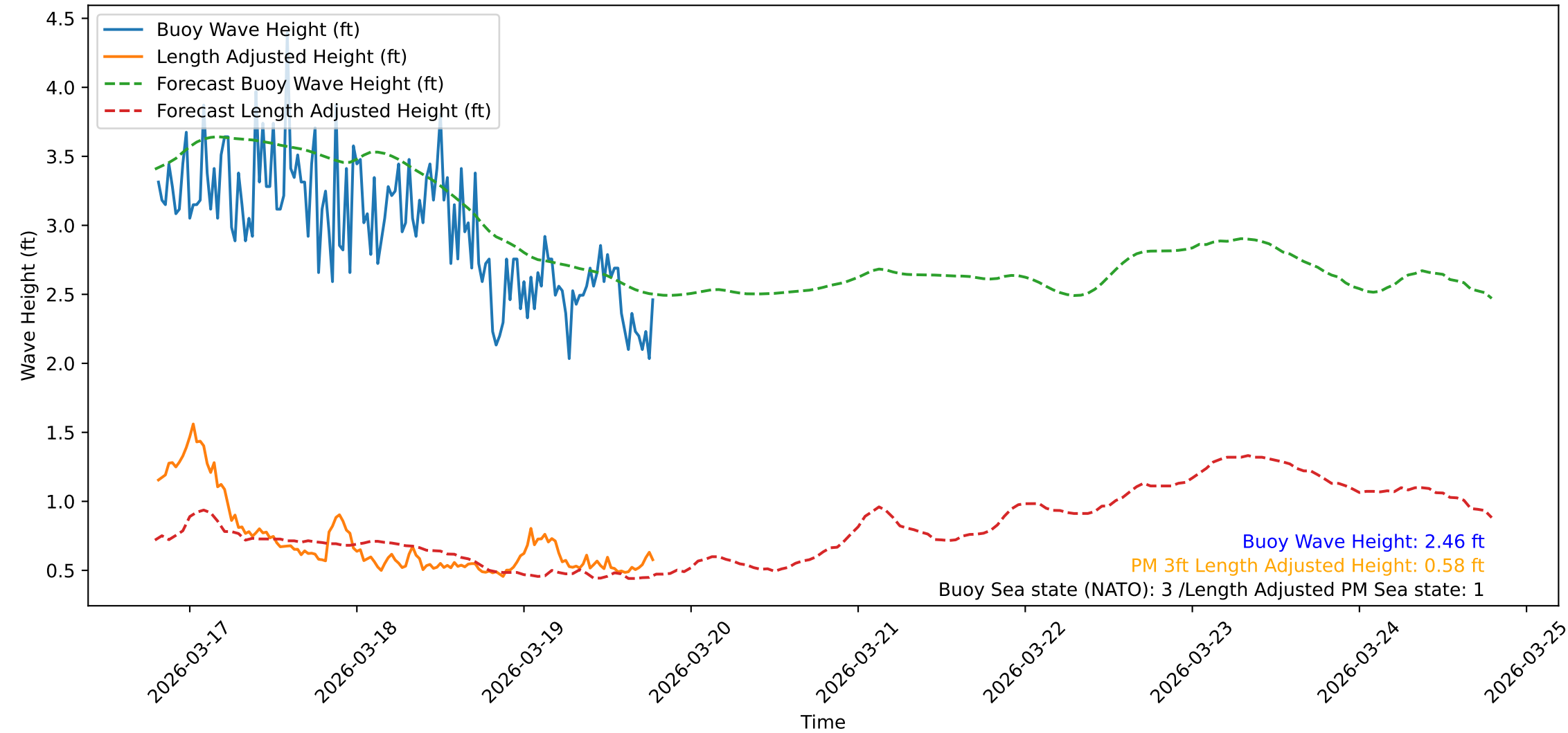
Wave Heights over Time for Oceanside Harbor at 2026-03-19 19:20:31
