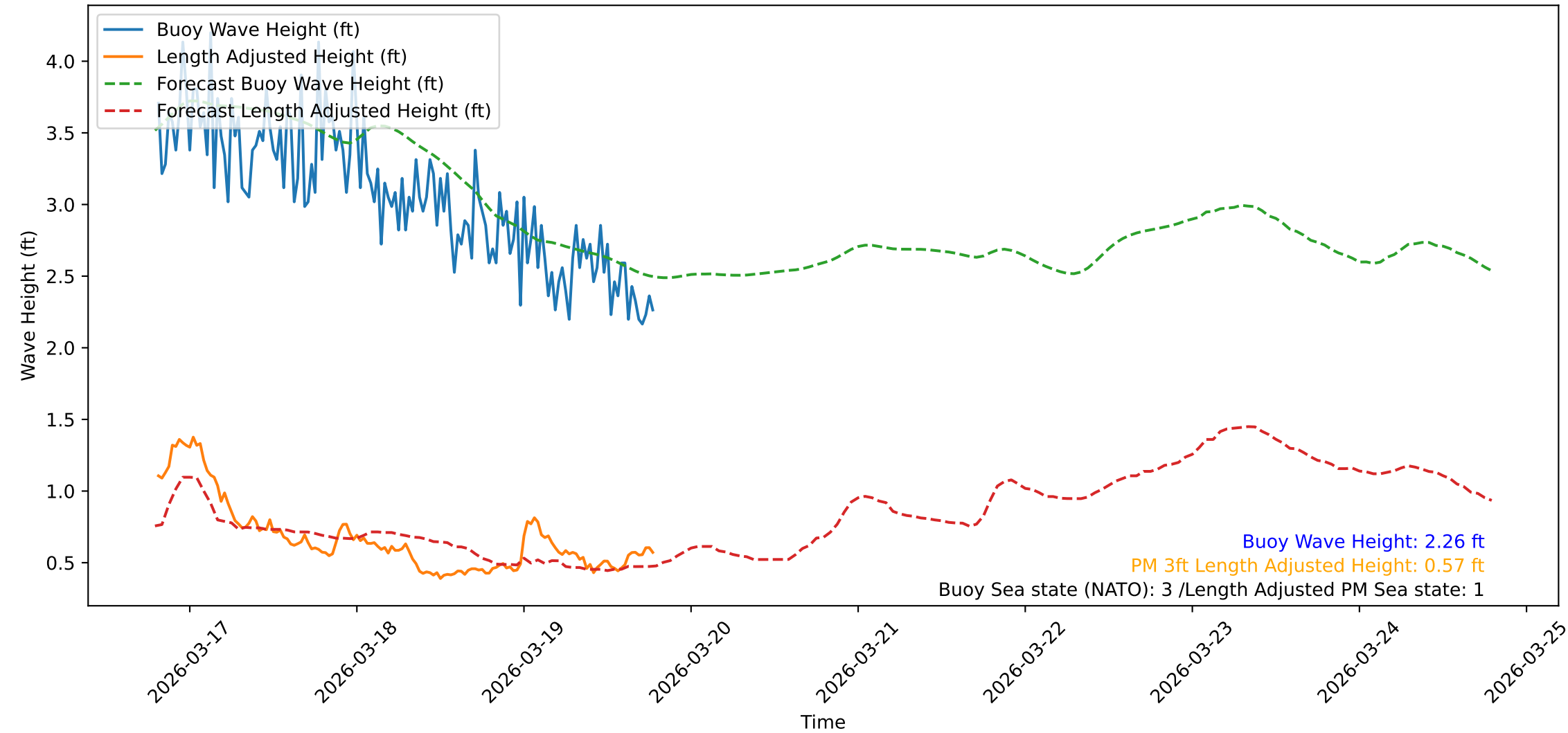
Wave Heights over Time for Green Beach at 2026-03-19 19:21:09
