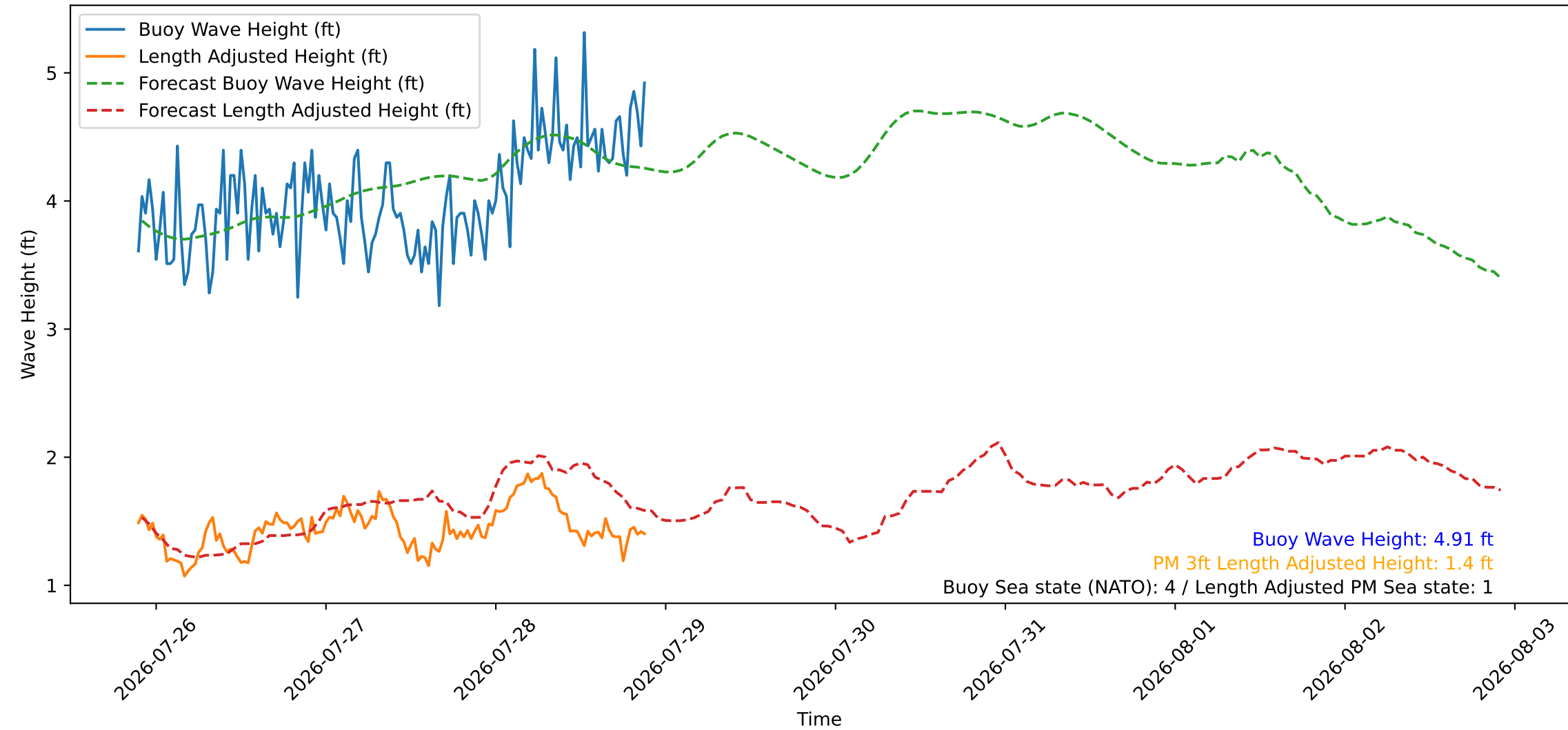
Wave Heights over Time for Oceanside Harbor at 2026-07-28 21:30:26
