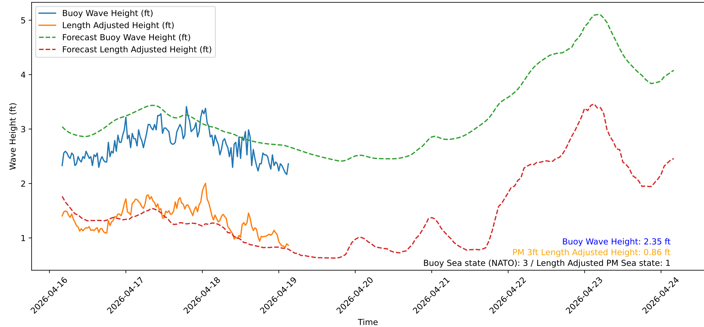
Wave Heights over Time for Oceanside Harbor at 2026-04-19 04:00:31
