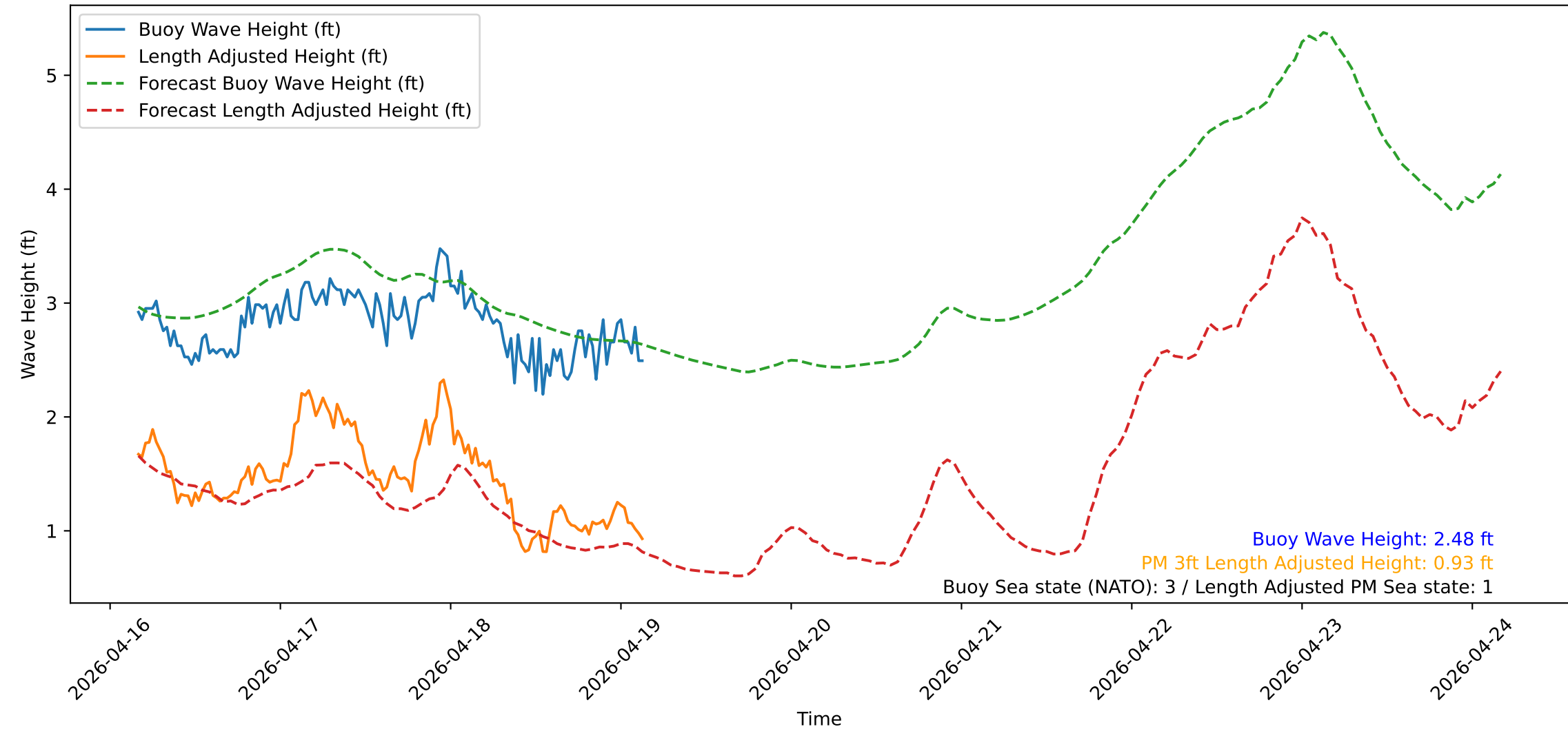
Wave Heights over Time for Green Beach at 2026-04-19 04:01:12
