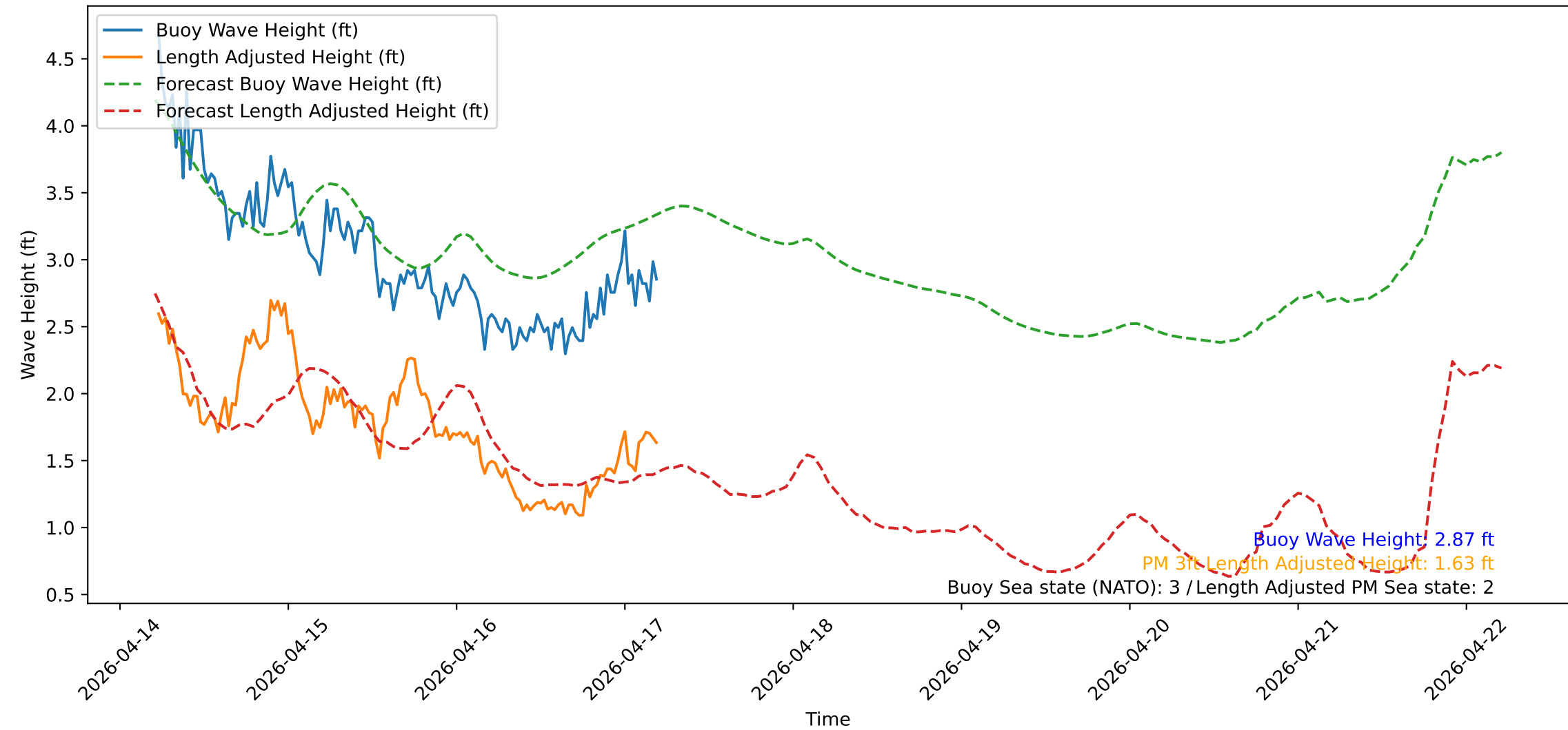
Wave Heights over Time for Oceanside Harbor at 2026-04-17 05:20:31
