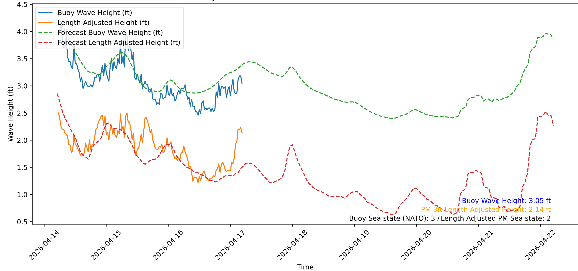
Wave Heights over Time for Green Beach at 2026-04-17 05:21:14
