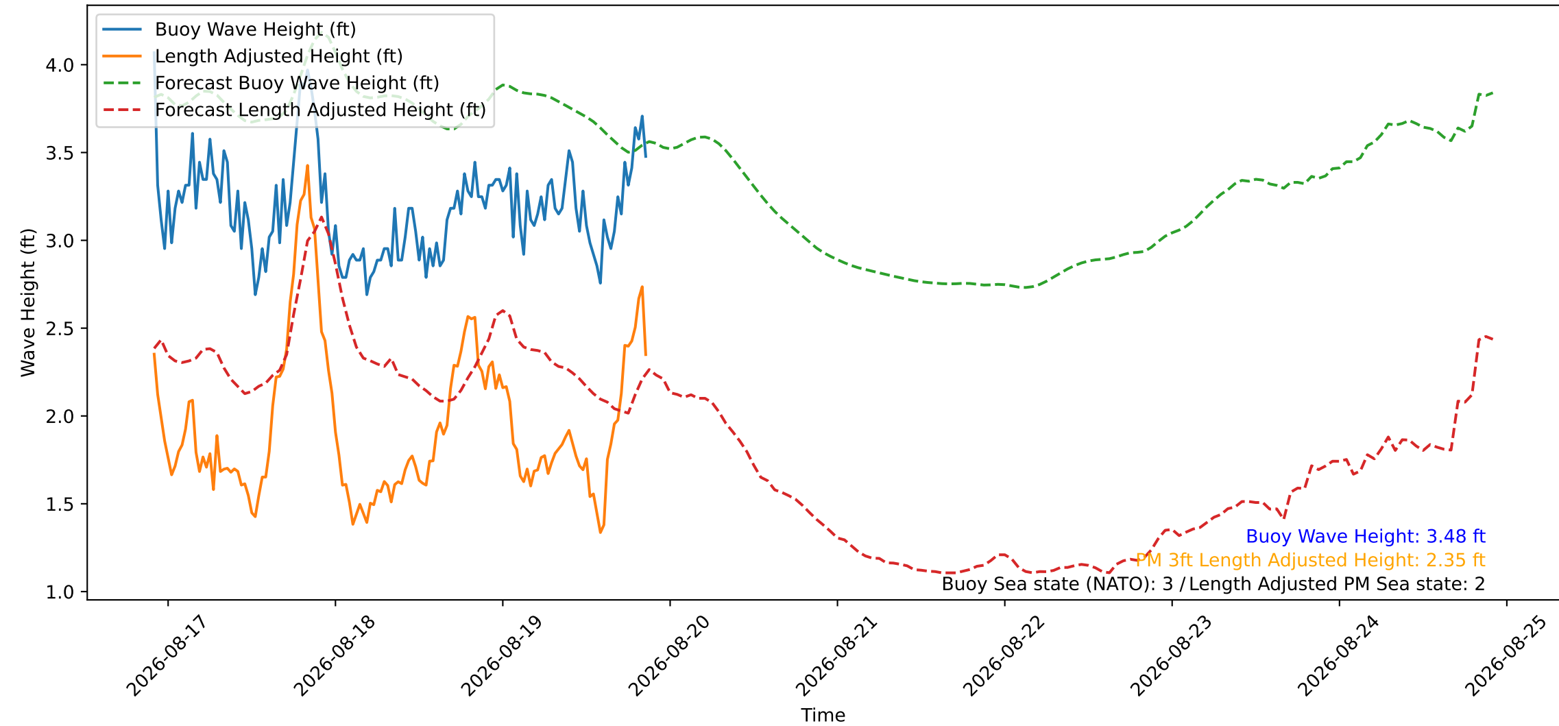
Wave Heights over Time for Green Beach at 2026-08-19 21:31:08
