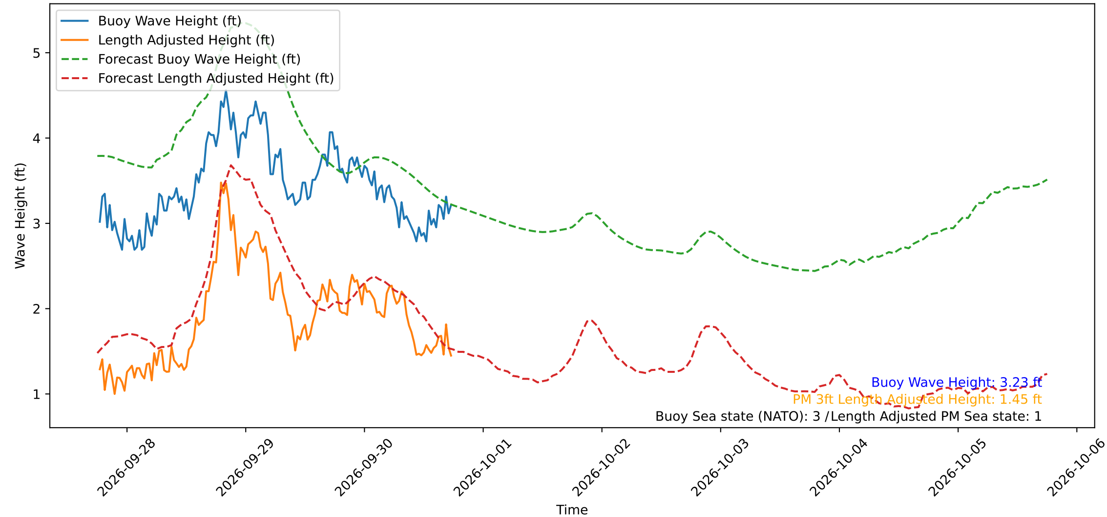
Wave Heights over Time for Green Beach at 2026-09-30 18:11:12
