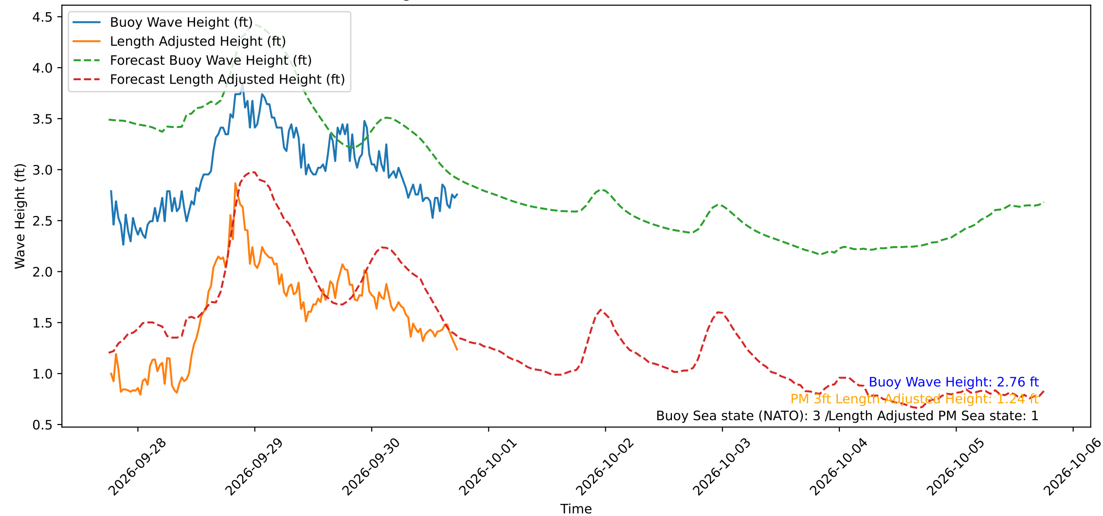
Wave Heights over Time for Red Beach at 2026-09-30 18:10:50
