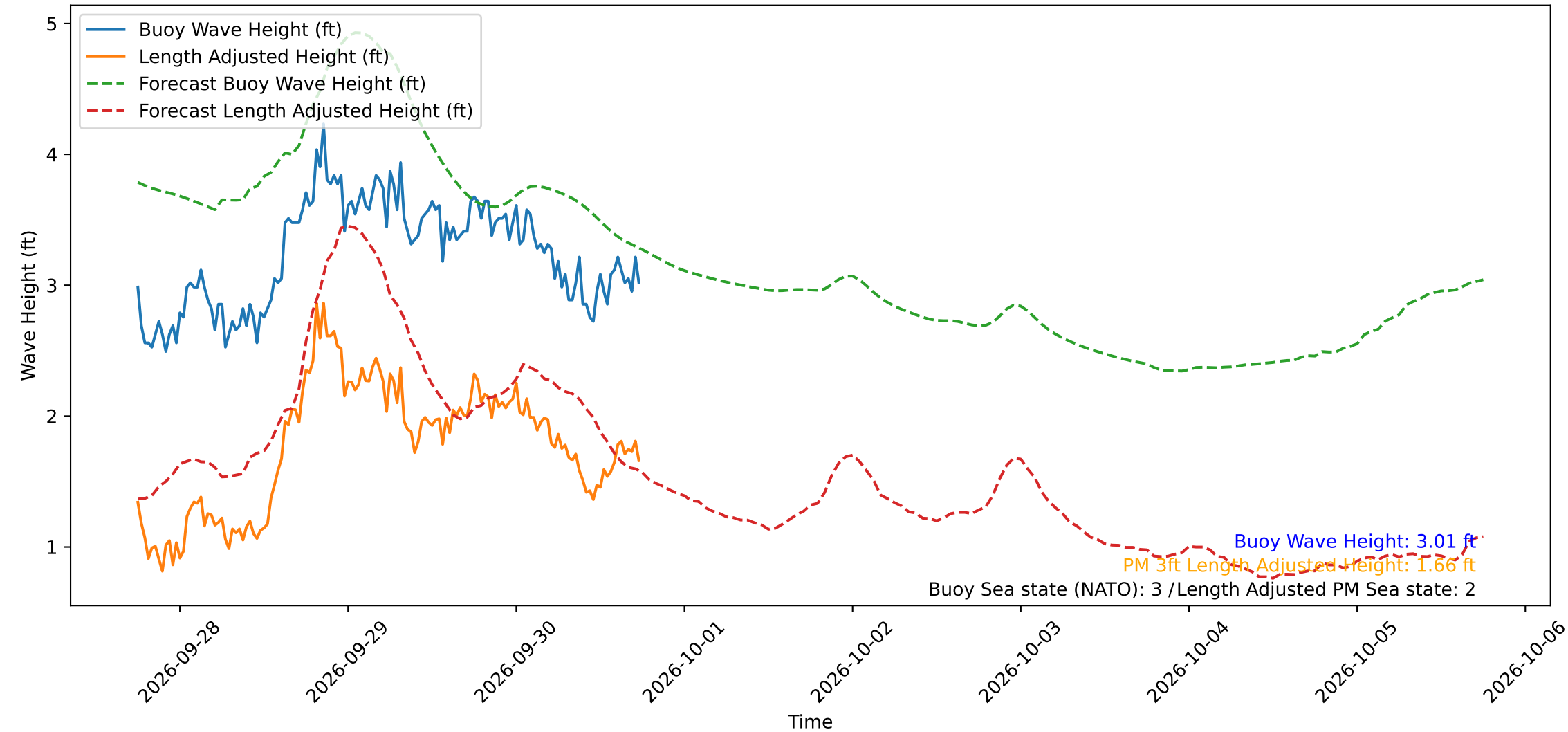
Wave Heights over Time for Oceanside Harbor at 2026-09-30 18:10:30
