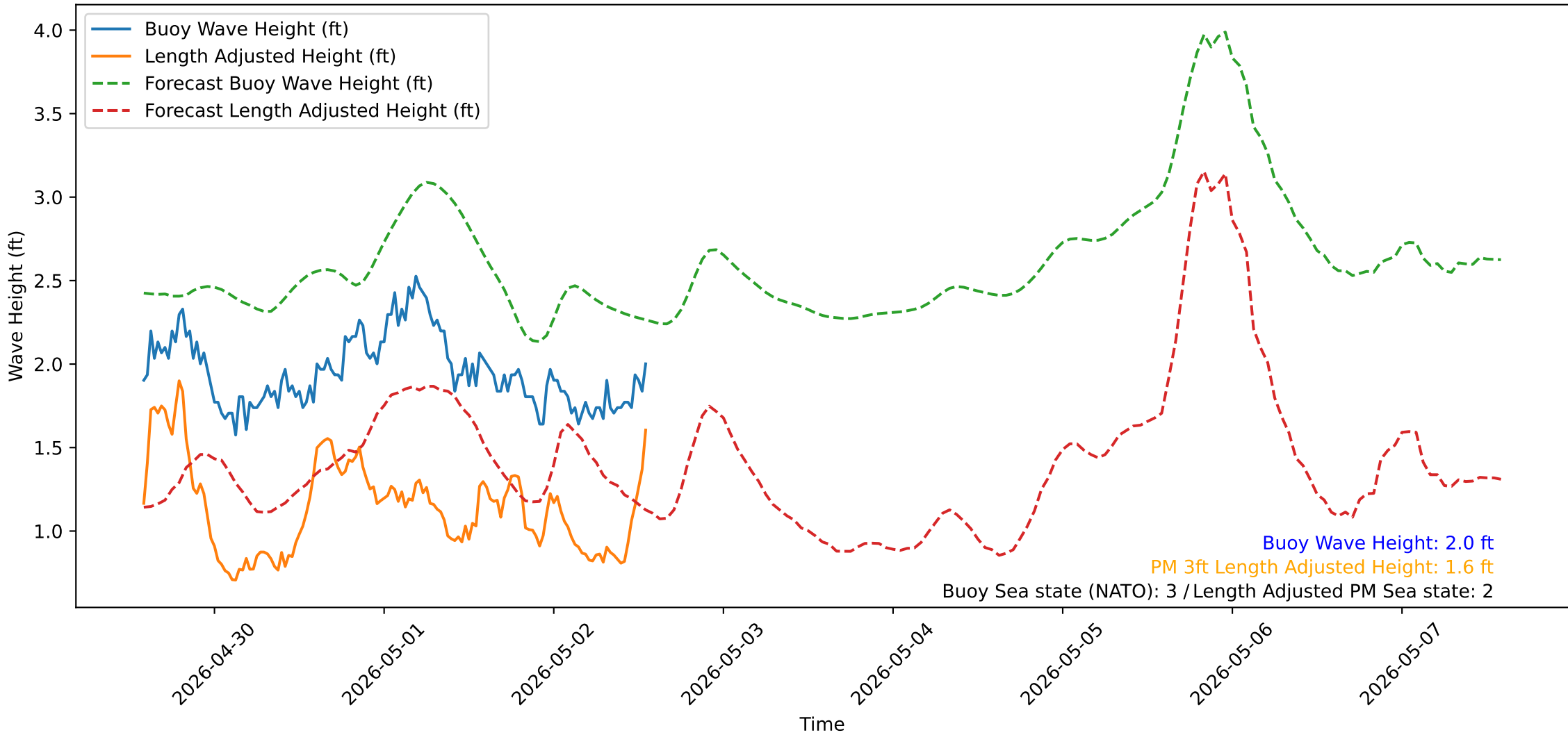
Wave Heights over Time for Red Beach at 2026-05-02 13:50:52
