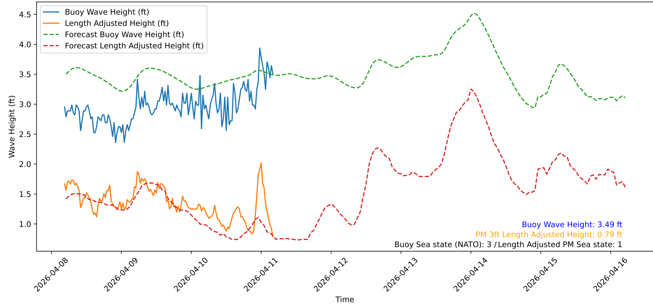
Wave Heights over Time for Green Beach at 2026-04-11 04:41:13
