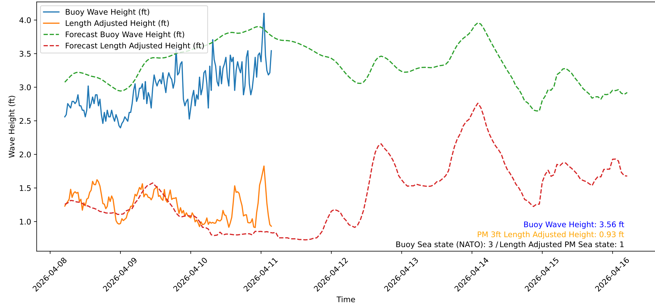
Wave Heights over Time for Red Beach at 2026-04-11 04:40:50
