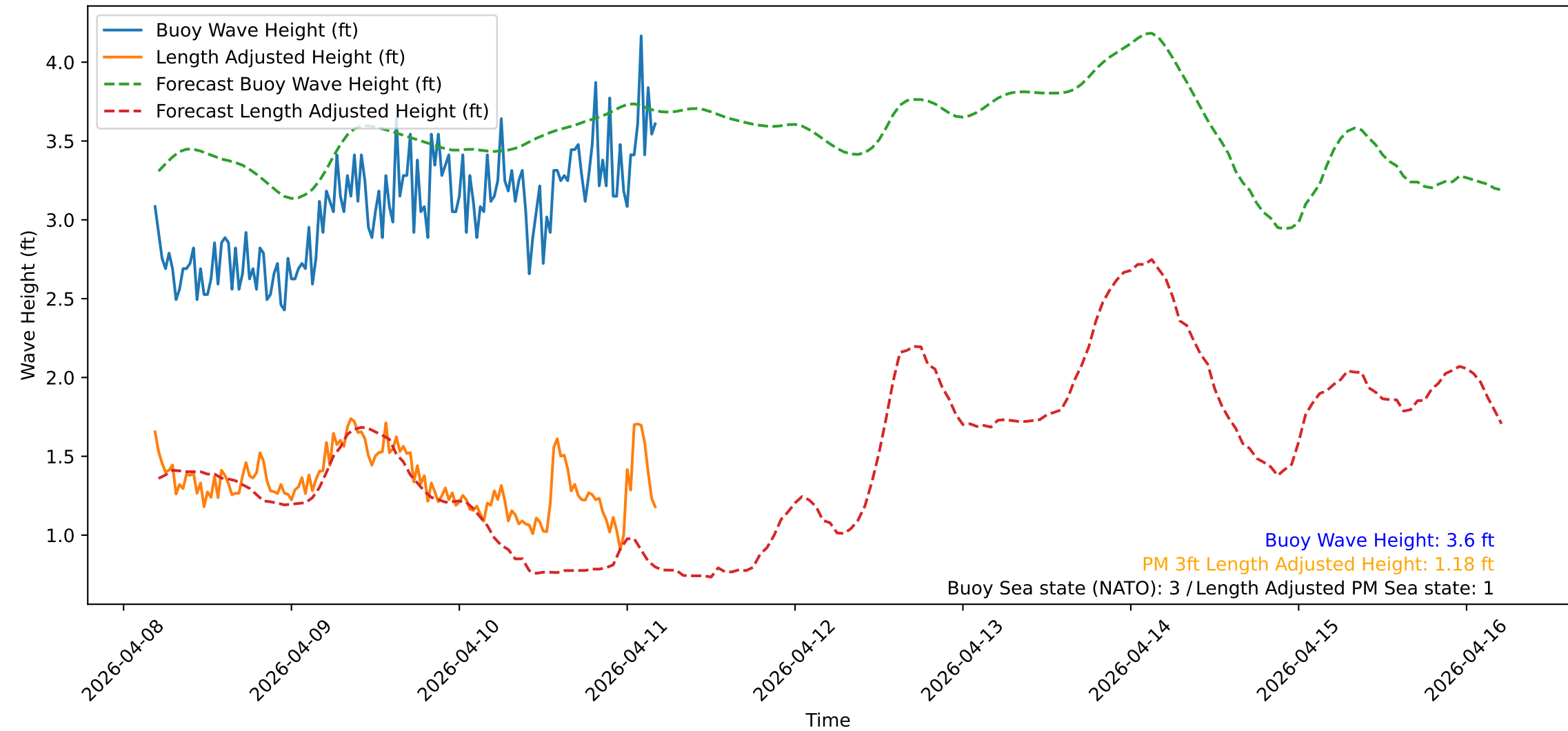
Wave Heights over Time for Oceanside Harbor at 2026-04-11 04:40:31
