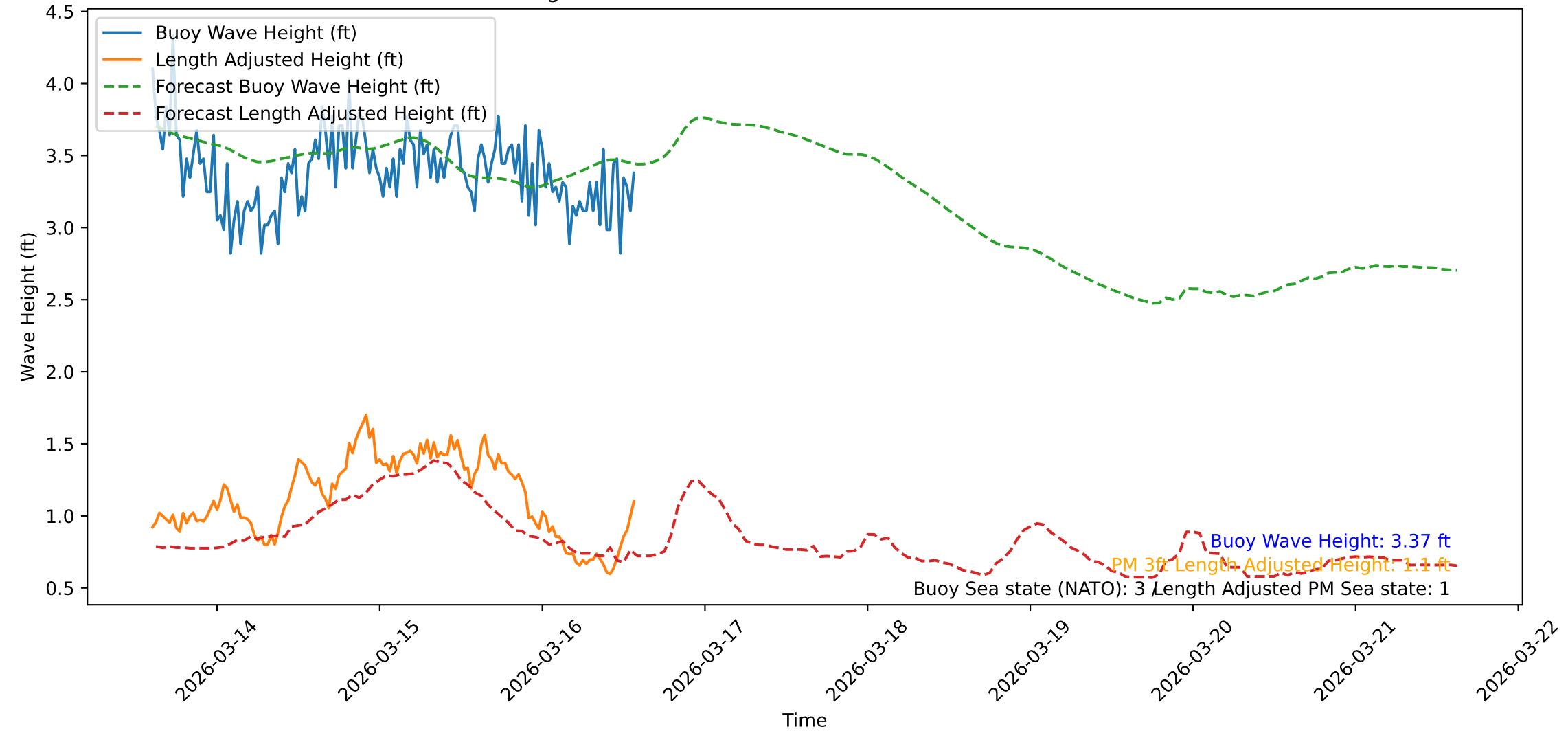
Wave Heights over Time for Green Beach at 2026-03-16 14:31:47
