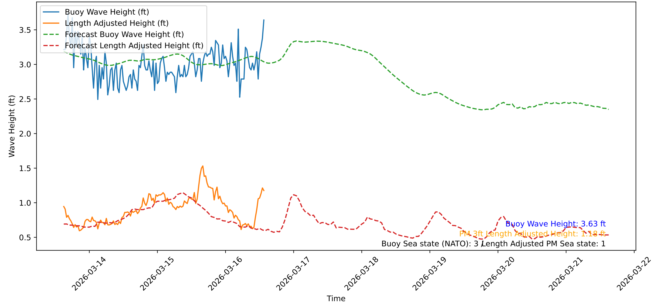
Wave Heights over Time for Red Beach at 2026-03-16 14:31:07
