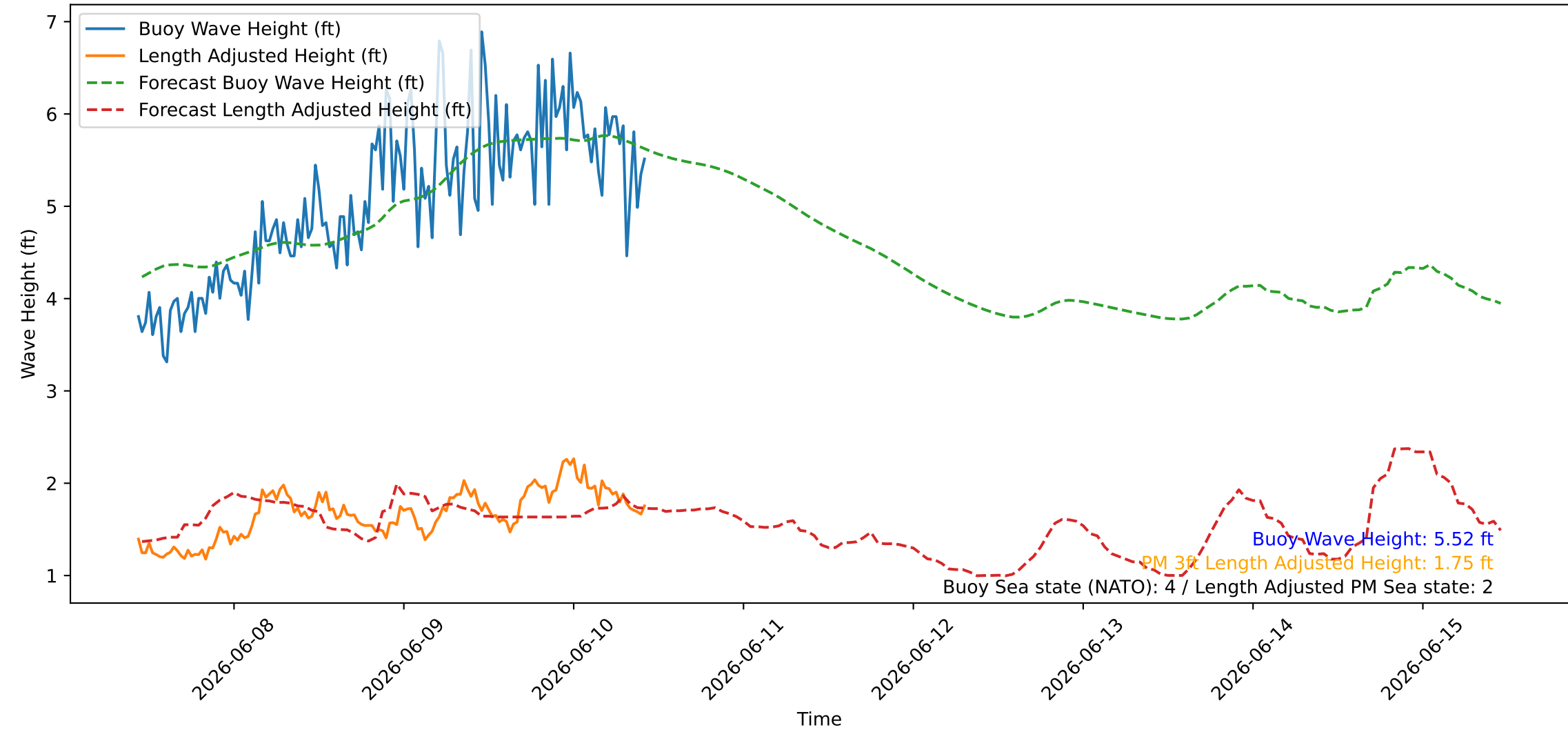
Wave Heights over Time for Green Beach at 2026-06-10 10:41:10
