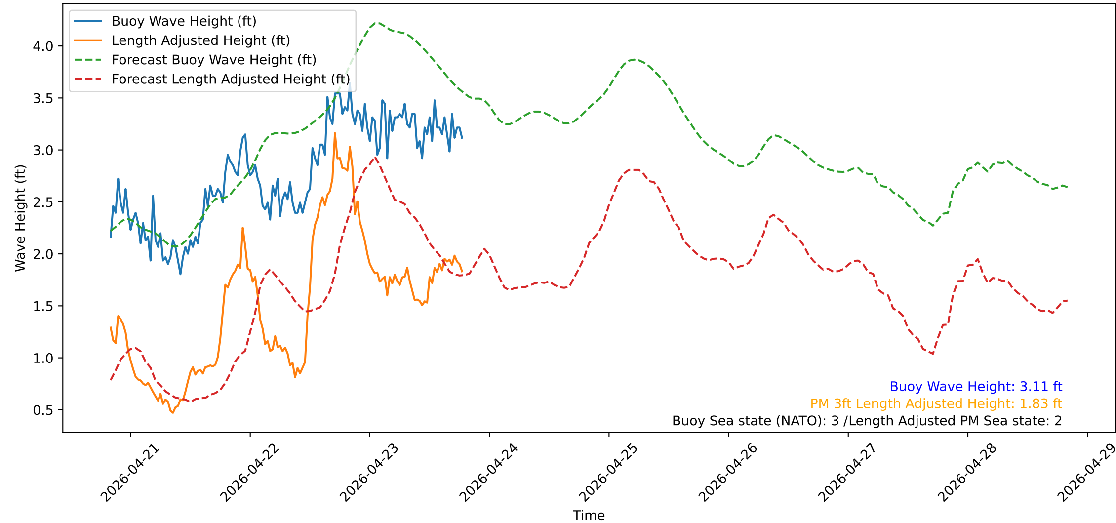
Wave Heights over Time for Red Beach at 2026-04-23 19:30:51
