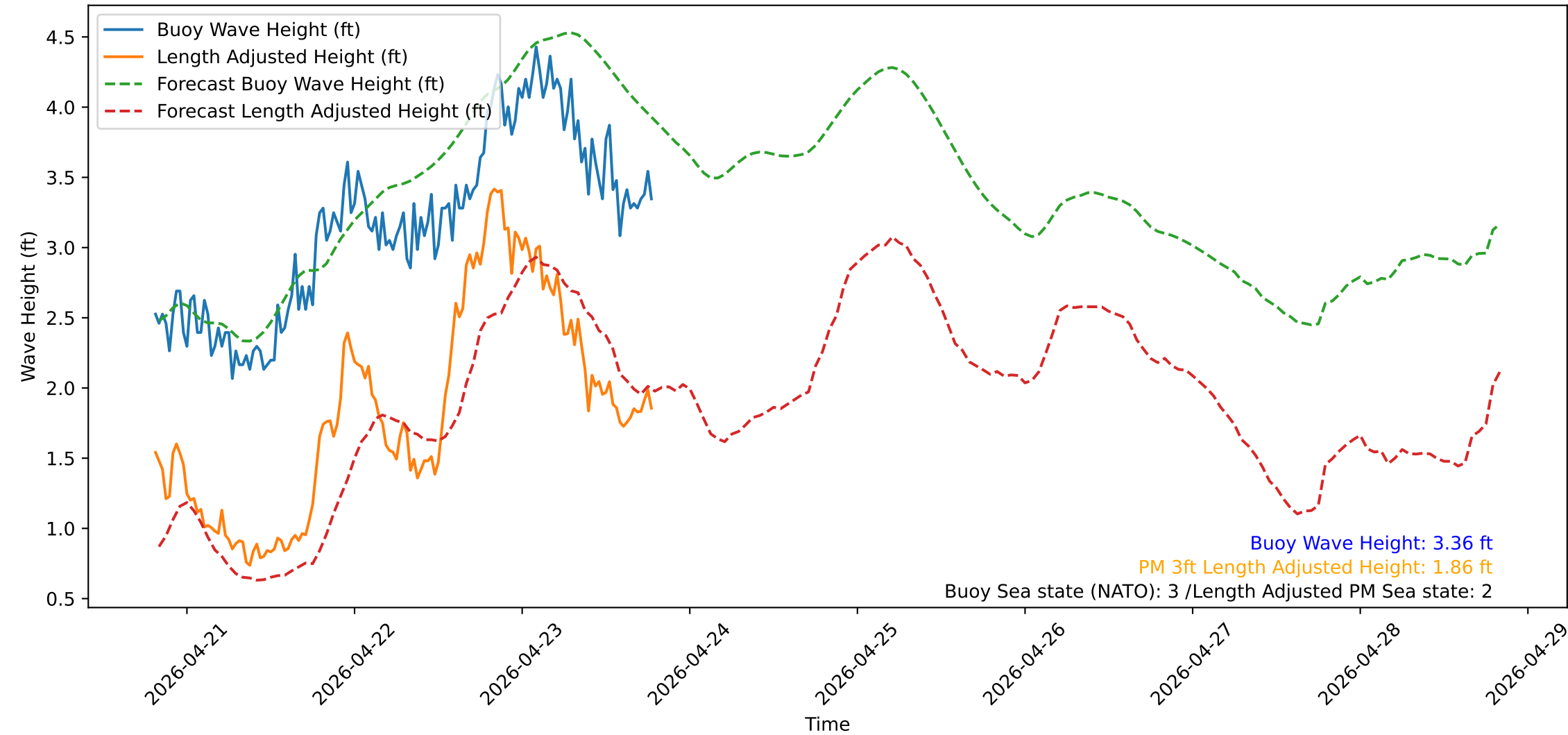
Wave Heights over Time for Oceanside Harbor at 2026-04-23 19:30:32
