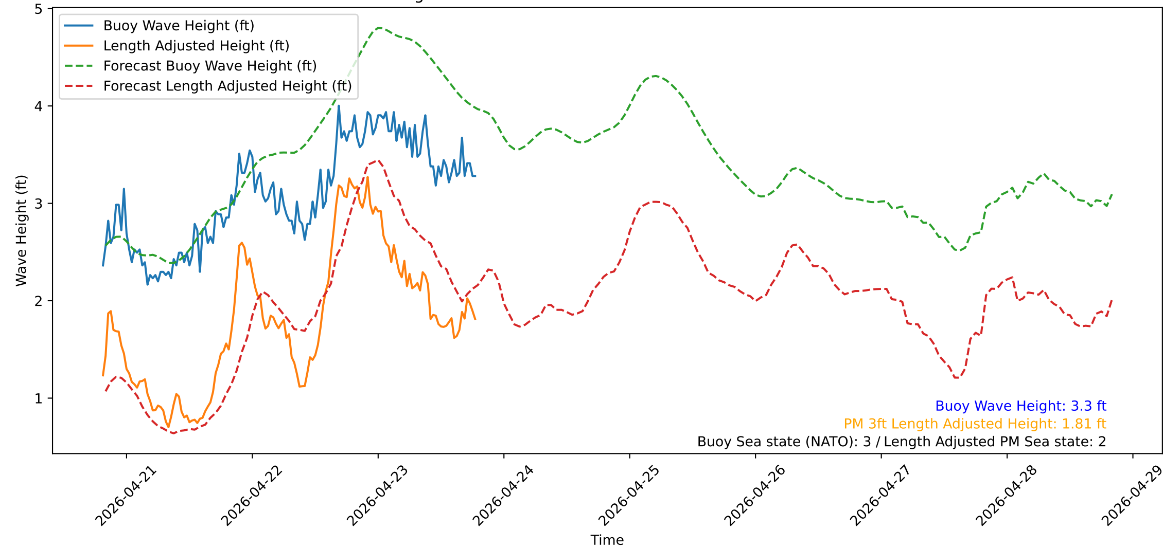
Wave Heights over Time for Green Beach at 2026-04-23 19:31:13
