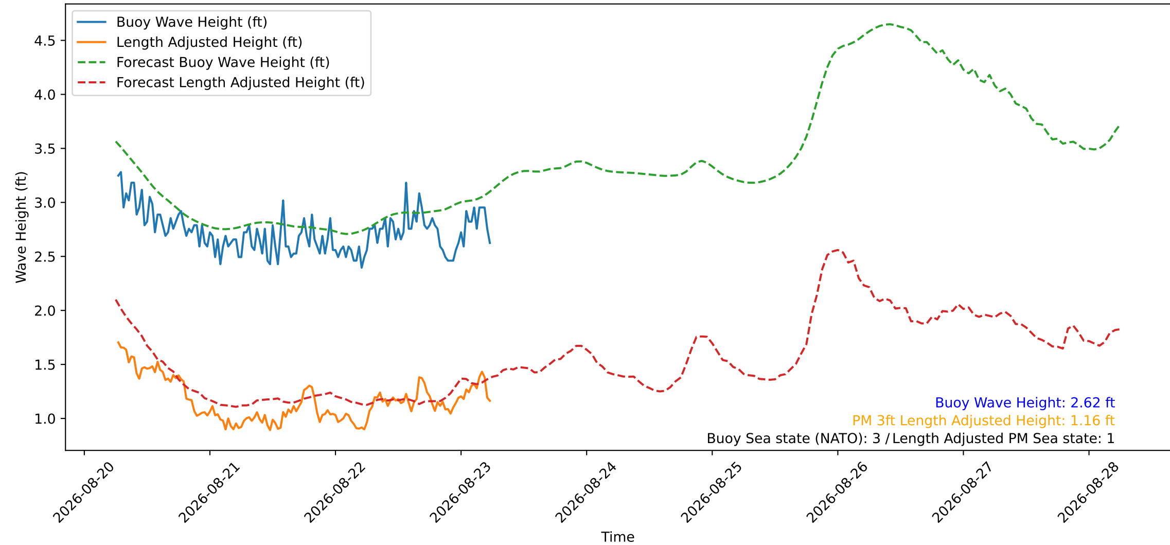
Wave Heights over Time for Green Beach at 2026-08-23 06:21:14
