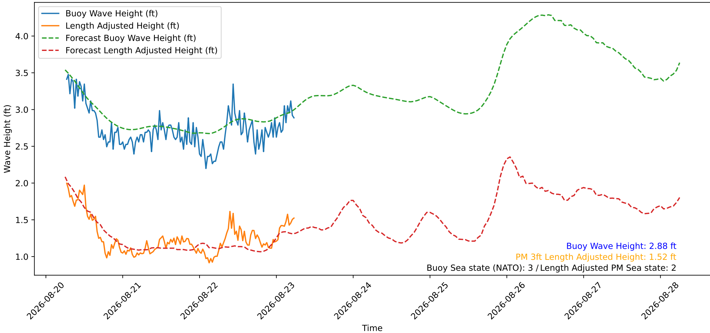
Wave Heights over Time for Oceanside Harbor at 2026-08-23 06:20:29
