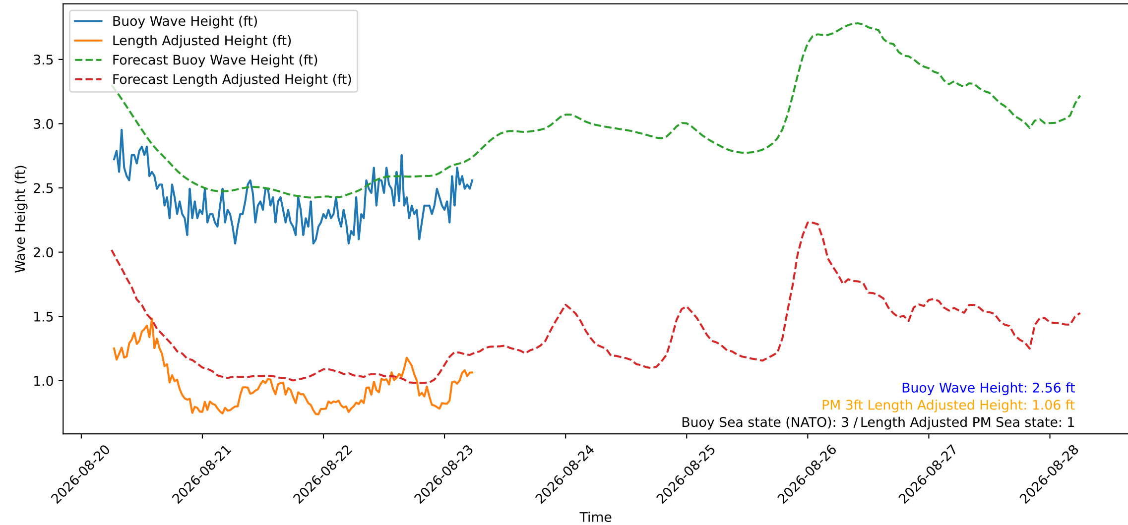
Wave Heights over Time for Red Beach at 2026-08-23 06:20:50
