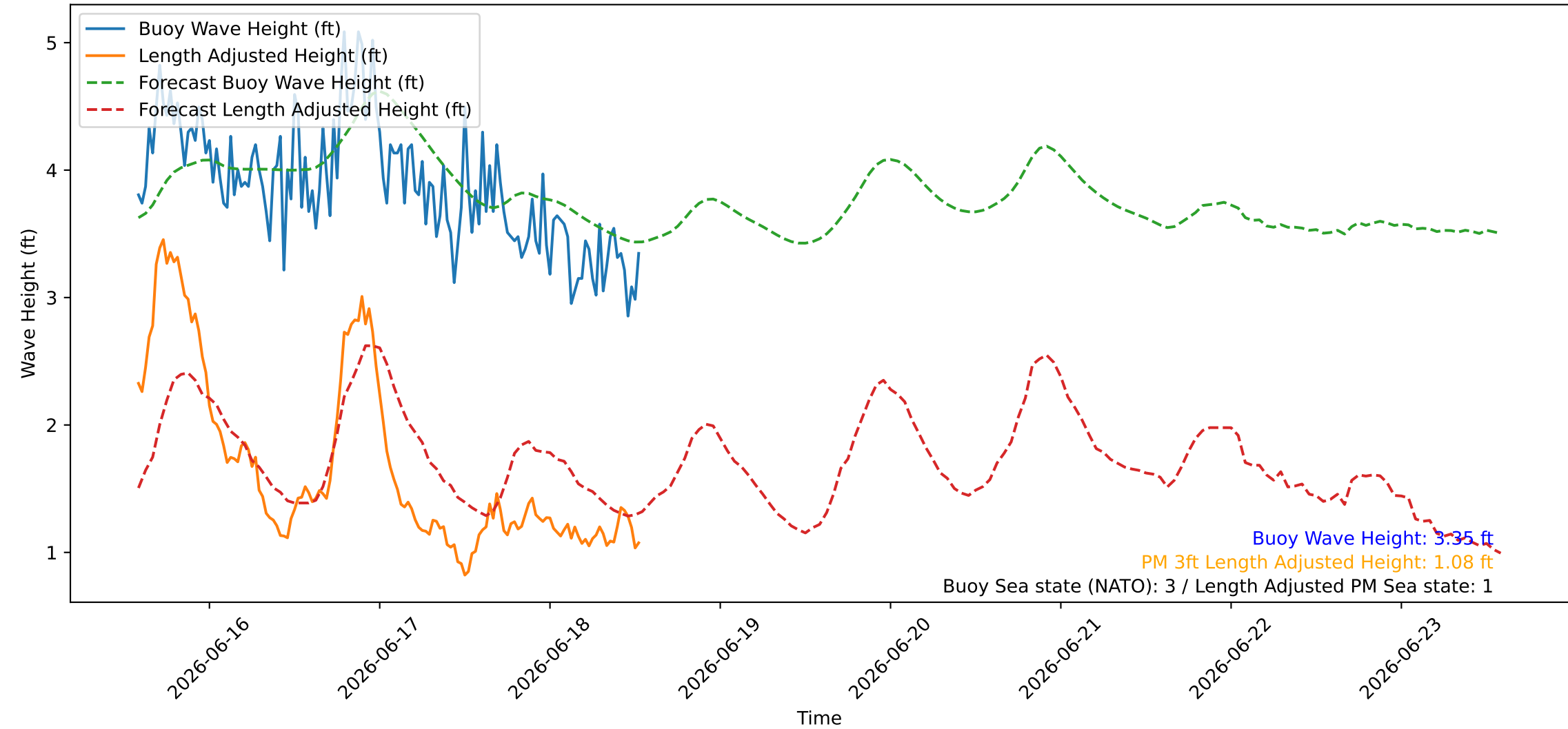
Wave Heights over Time for Green Beach at 2026-06-18 13:51:10
