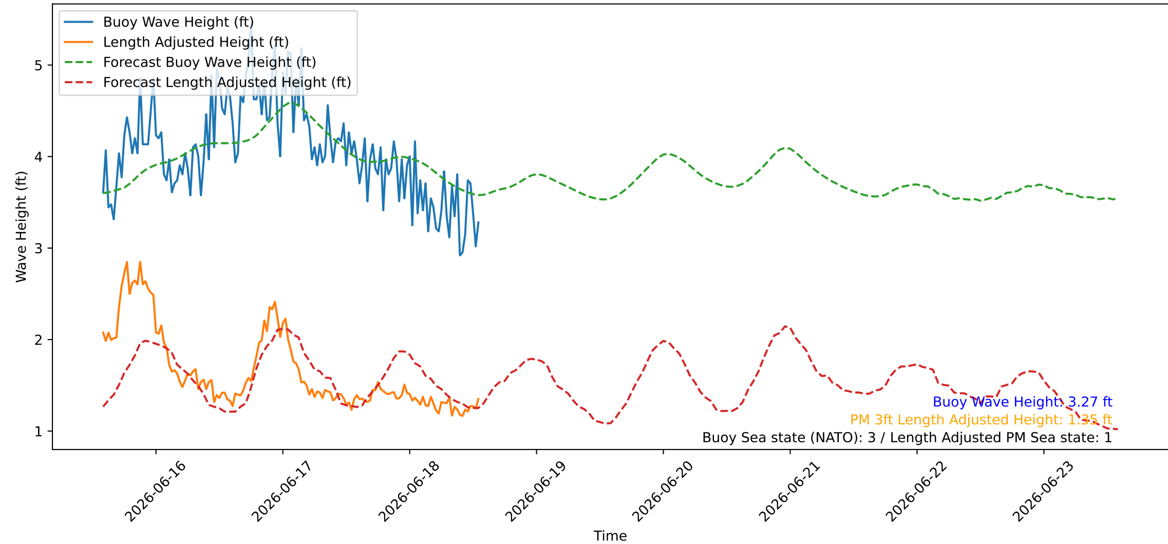
Wave Heights over Time for Oceanside Harbor at 2026-06-18 13:50:27
