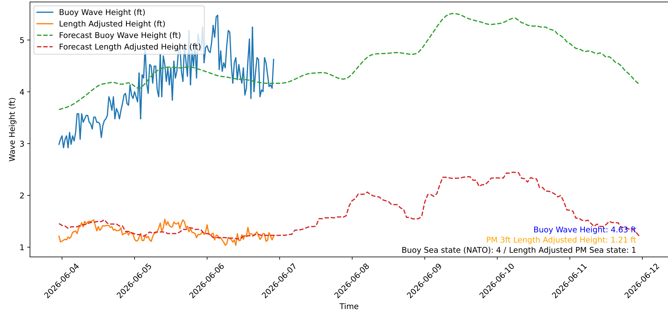
Wave Heights over Time for Oceanside Harbor at 2026-06-06 22:50:26
