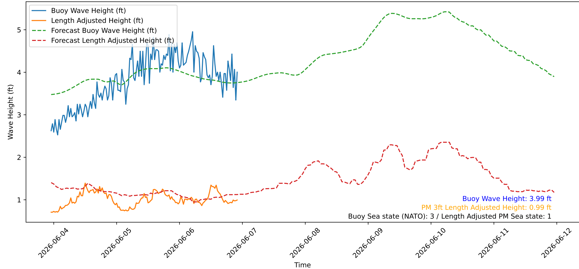
Wave Heights over Time for Red Beach at 2026-06-06 22:50:47
