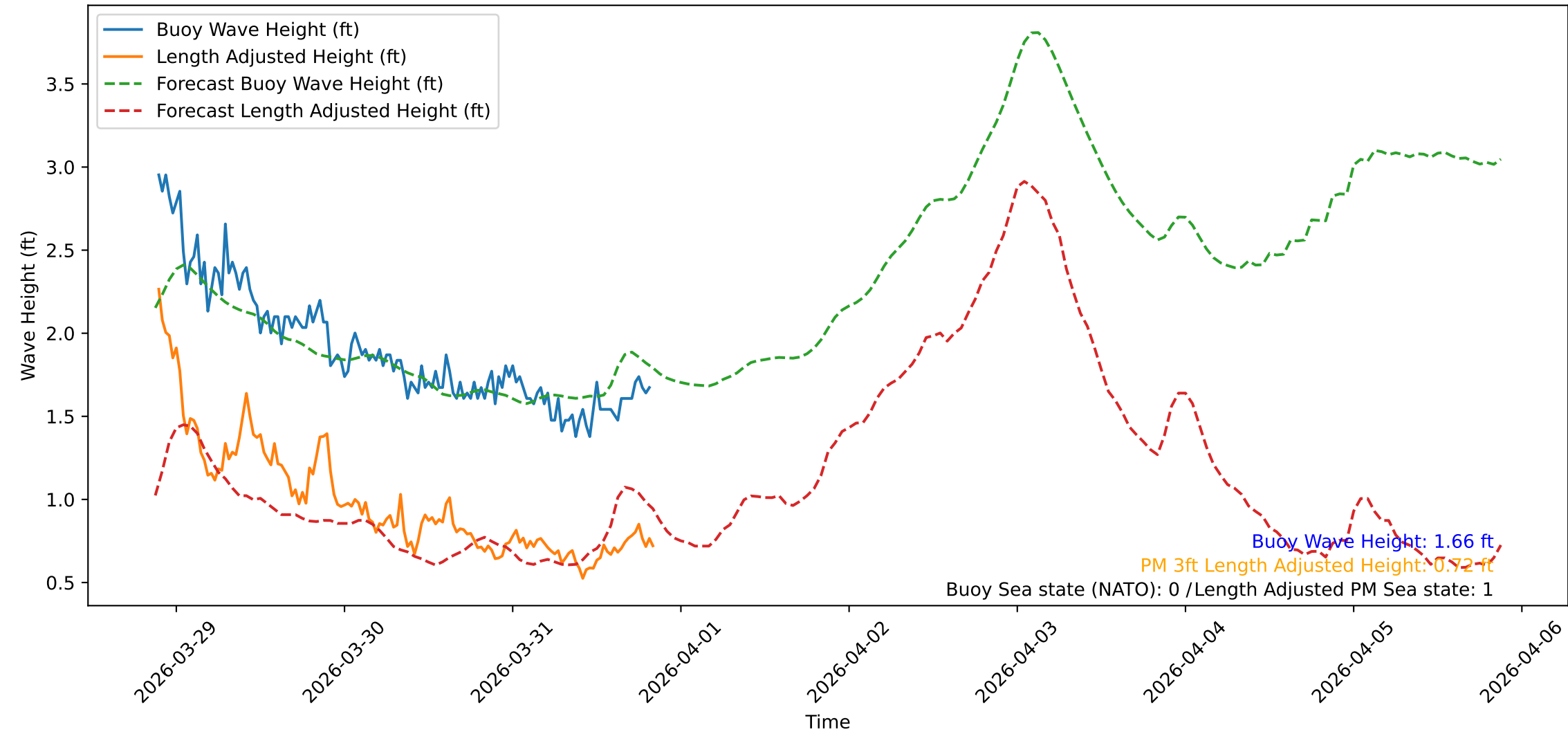
Wave Heights over Time for Red Beach at 2026-03-31 21:00:47
