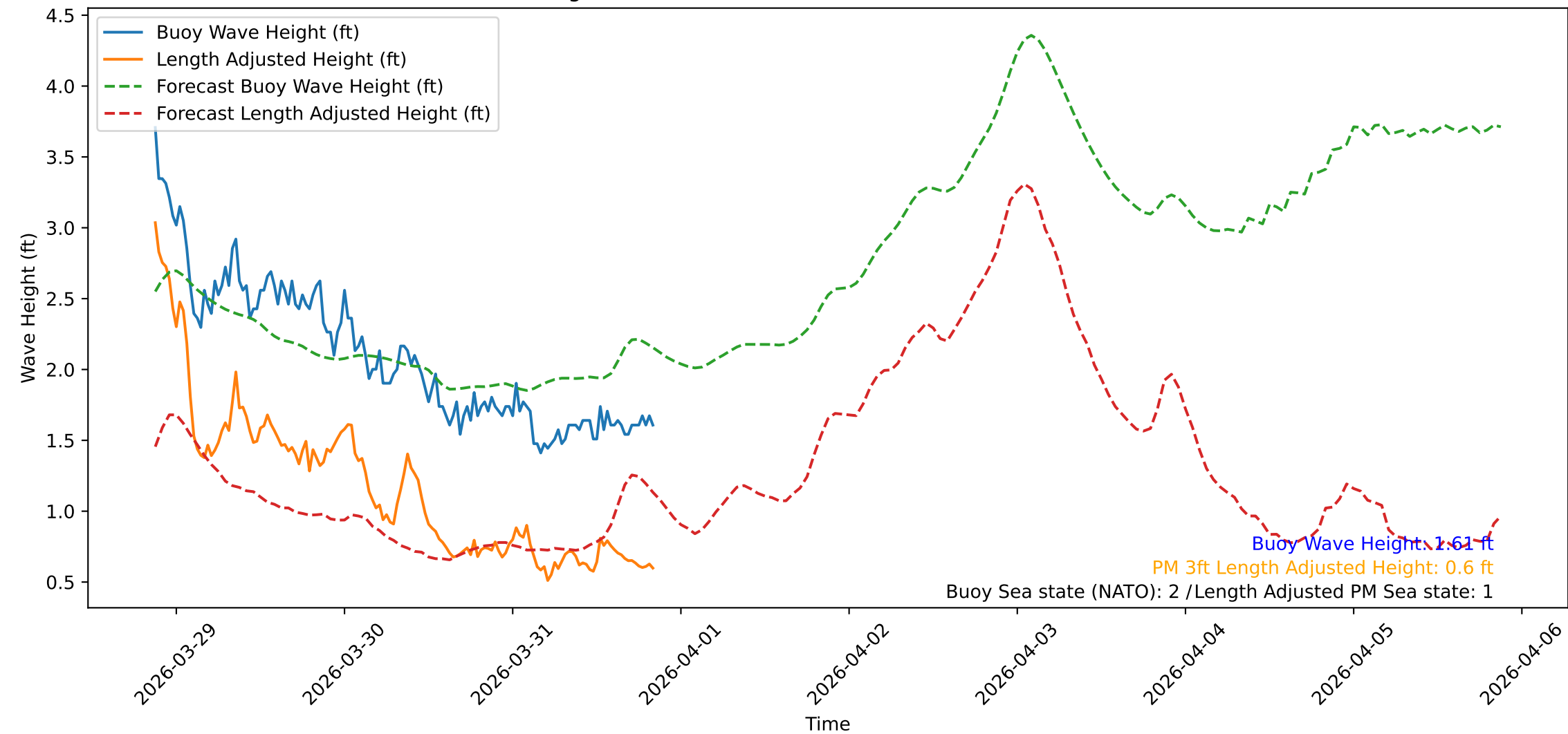
Wave Heights over Time for Green Beach at 2026-03-31 21:01:09
