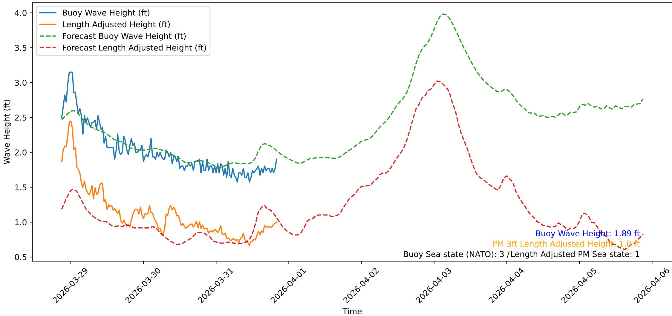
Wave Heights over Time for Oceanside Harbor at 2026-03-31 21:00:31
