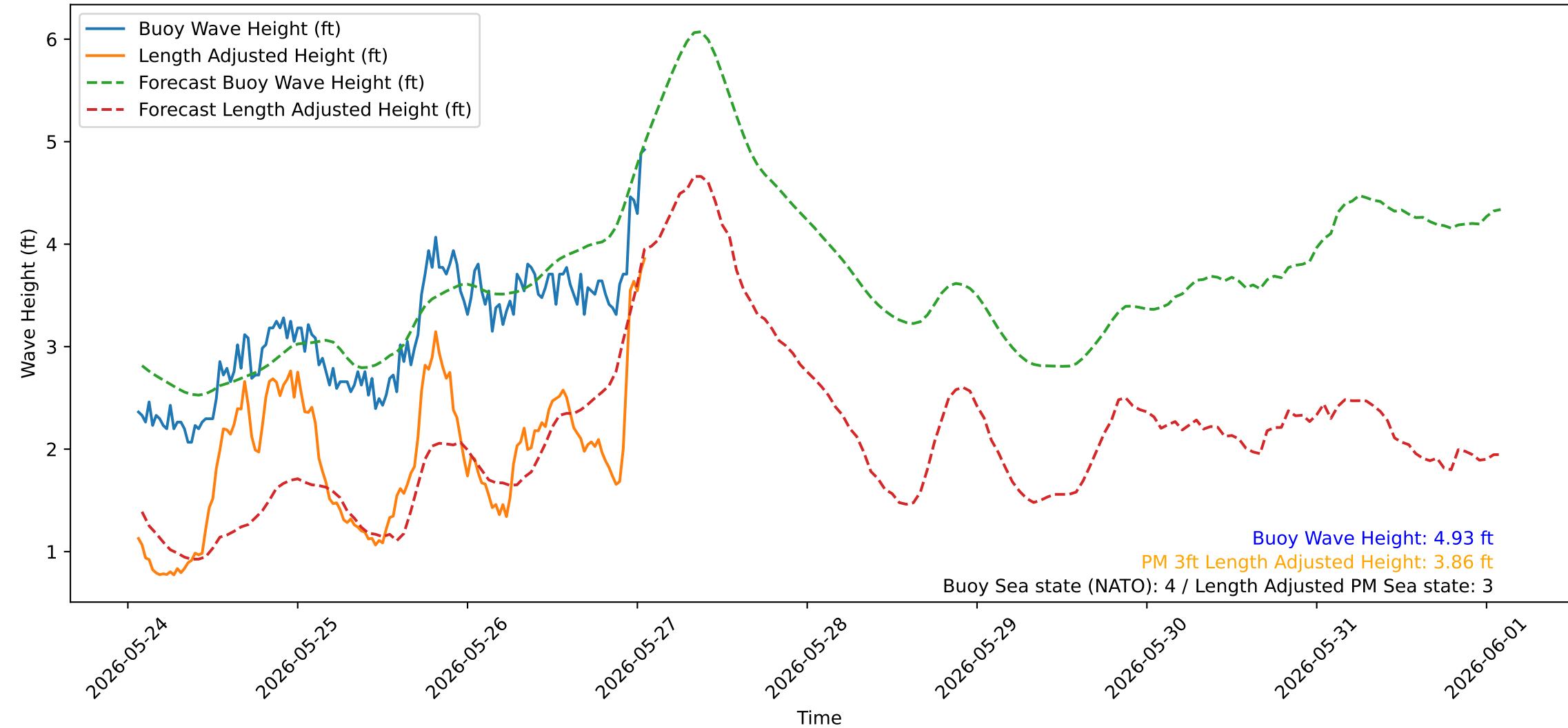
Wave Heights over Time for Green Beach at 2026-05-27 01:41:09
