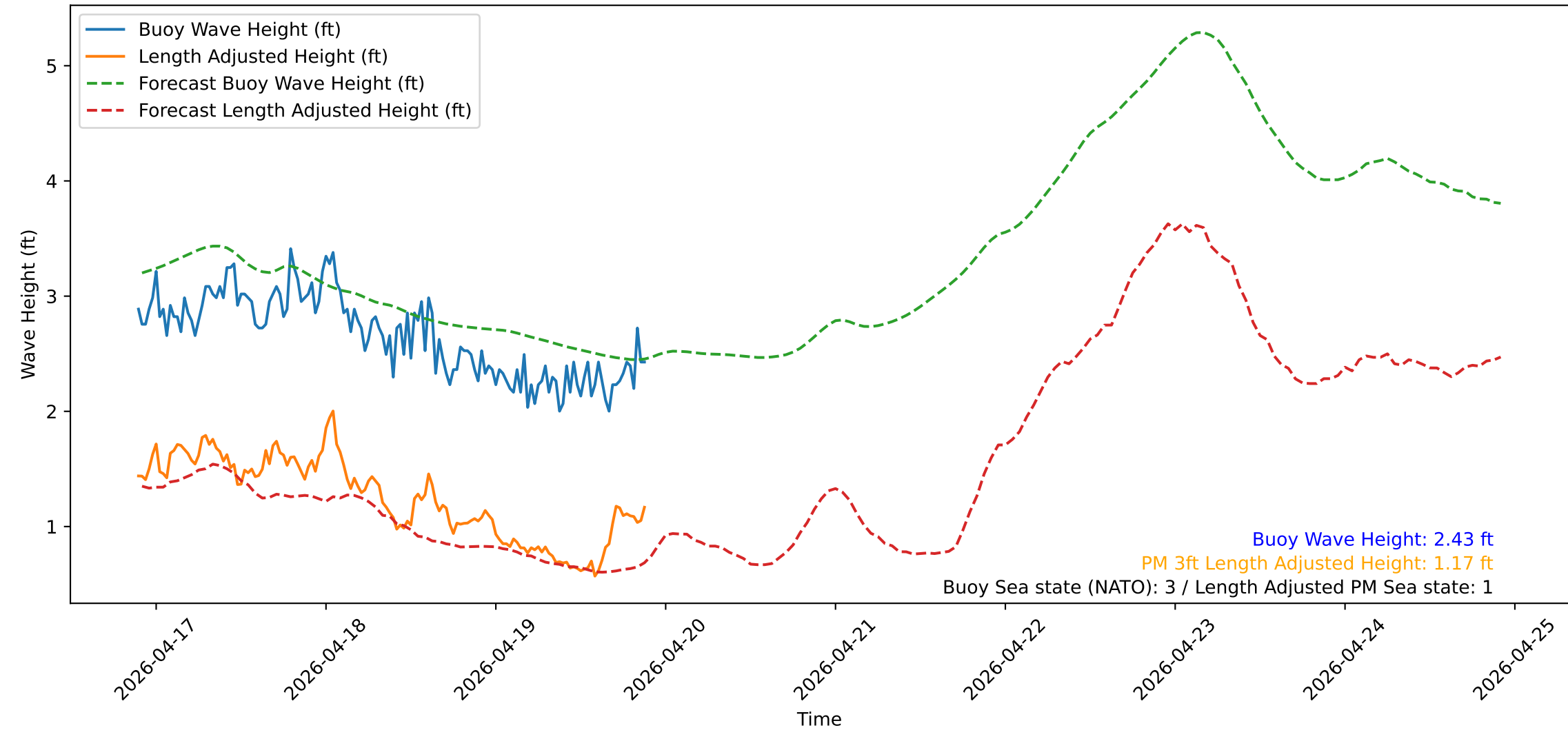
Wave Heights over Time for Oceanside Harbor at 2026-04-19 21:40:31
