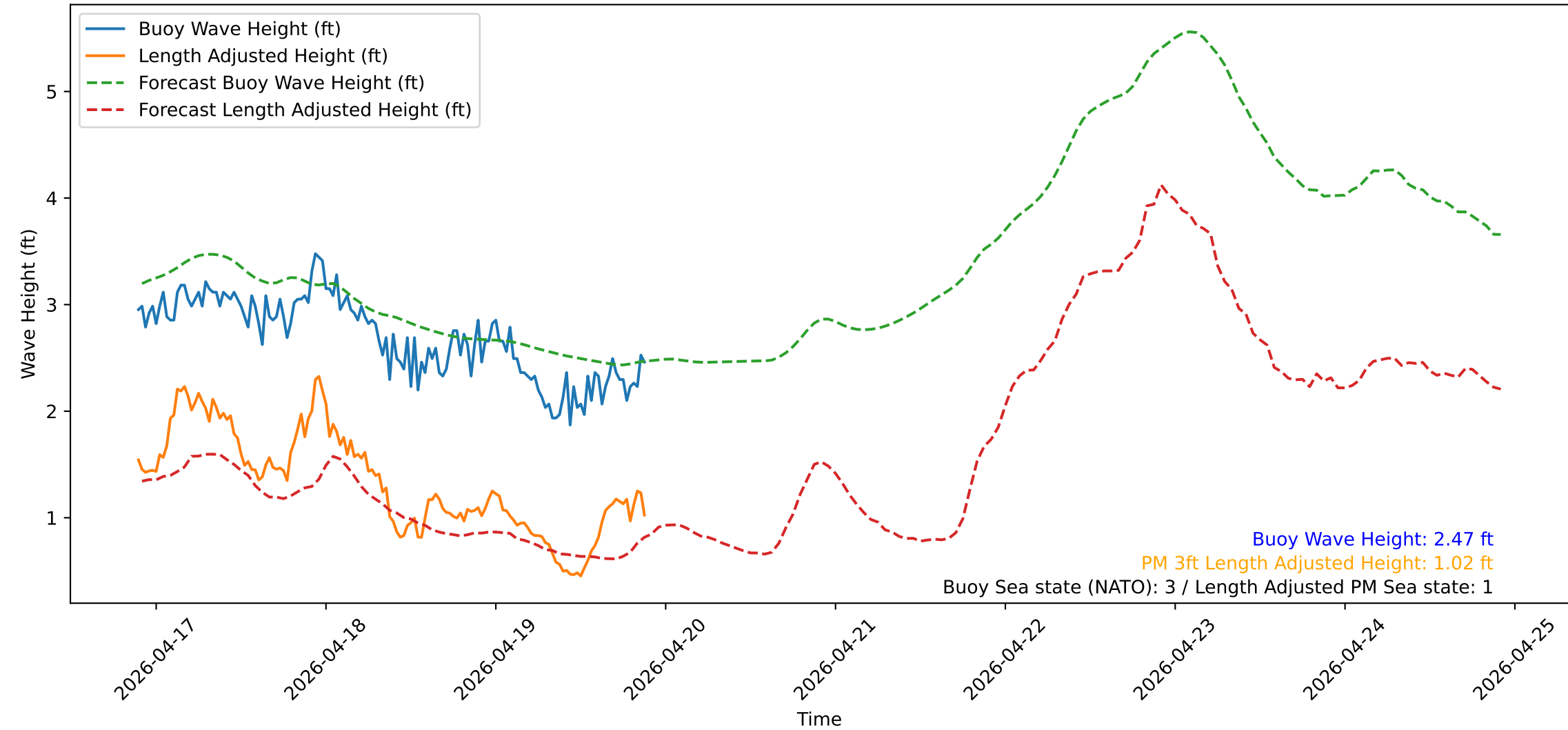
Wave Heights over Time for Green Beach at 2026-04-19 21:41:13
