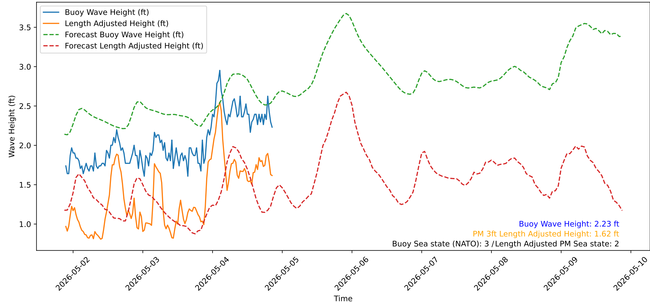
Wave Heights over Time for Red Beach at 2026-05-04 21:10:51
