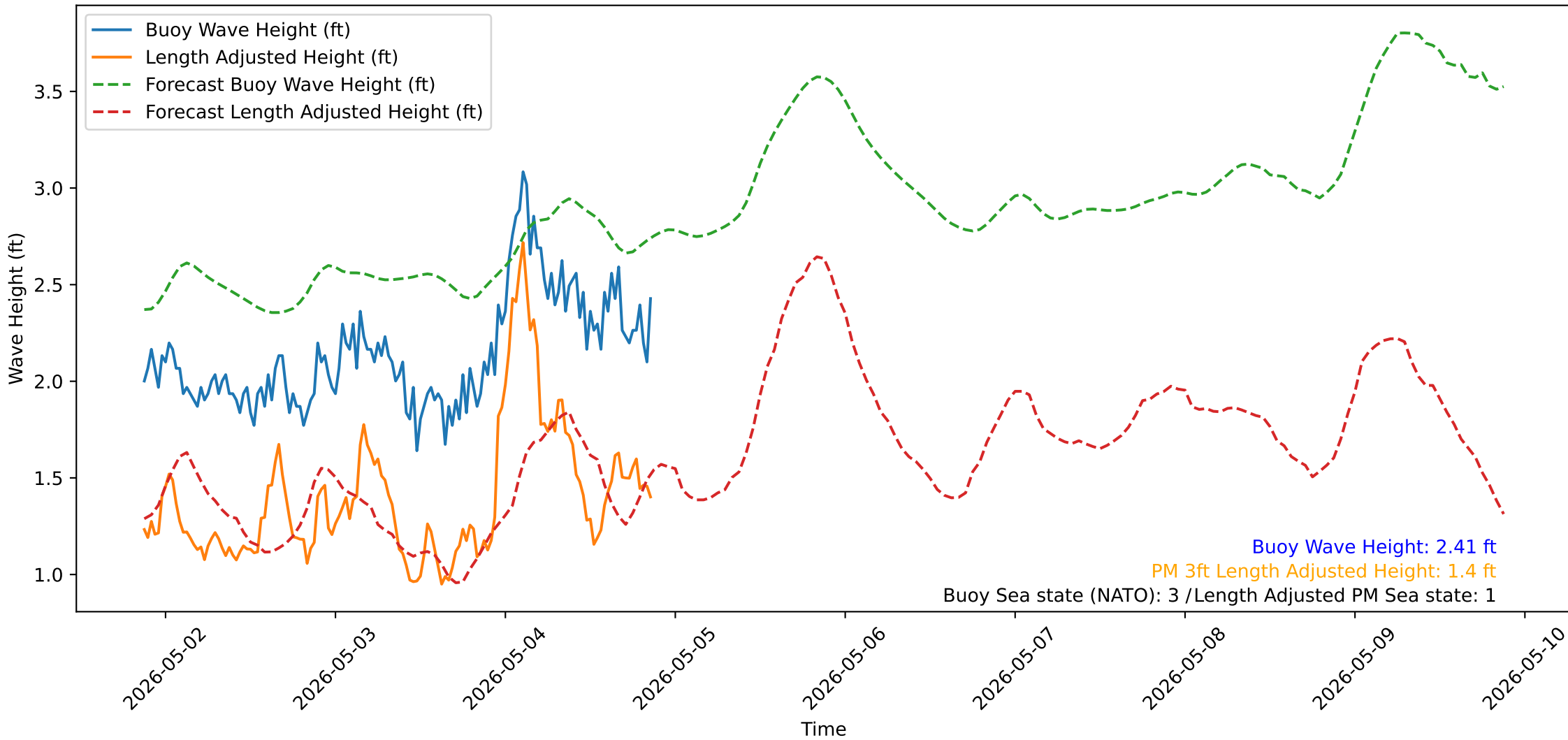
Wave Heights over Time for Oceanside Harbor at 2026-05-04 21:10:32
