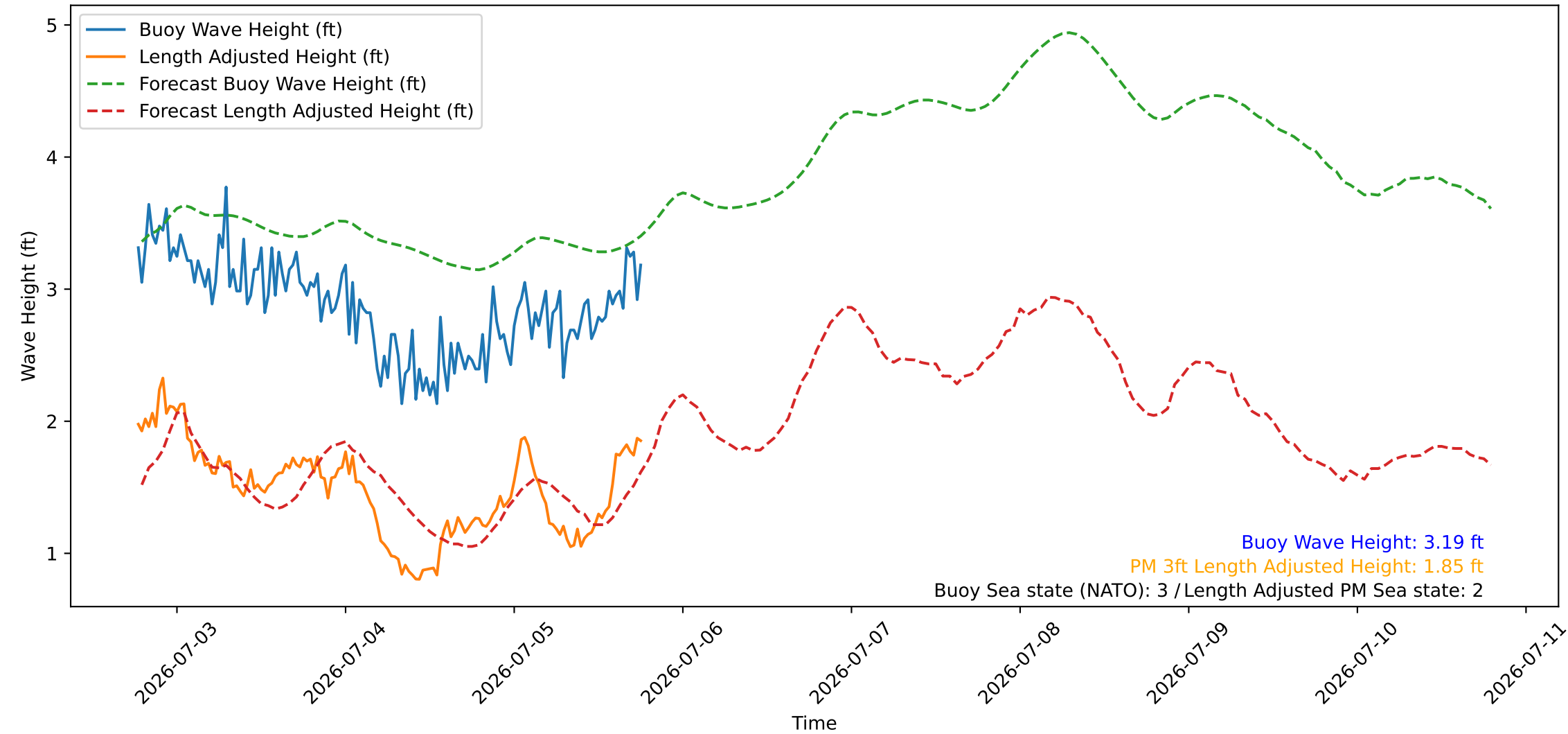
Wave Heights over Time for Oceanside Harbor at 2026-07-05 18:40:27
