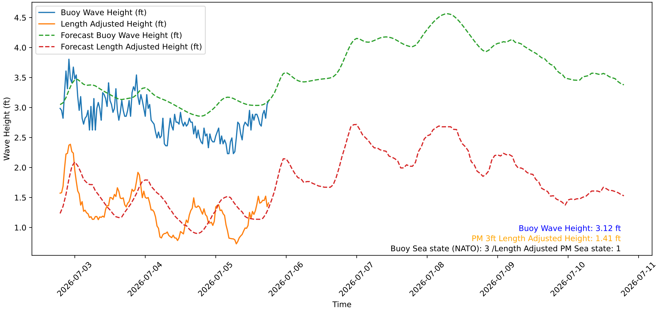
Wave Heights over Time for Red Beach at 2026-07-05 18:40:46
