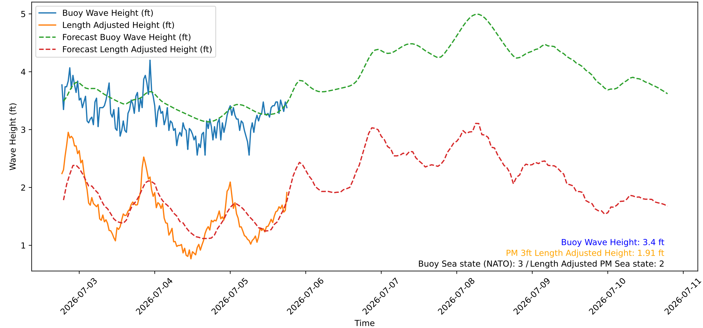
Wave Heights over Time for Green Beach at 2026-07-05 18:41:09
