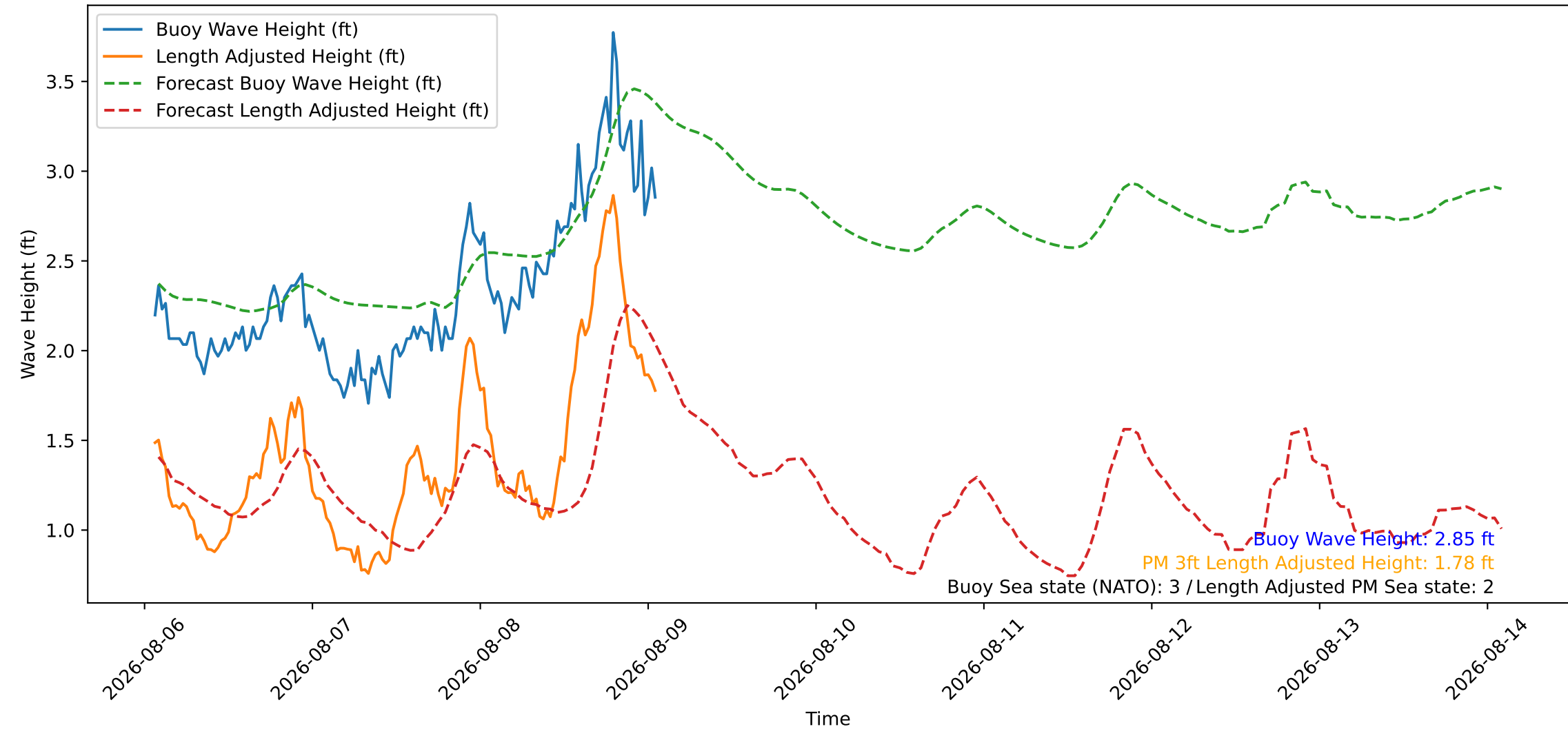
Wave Heights over Time for Green Beach at 2026-08-09 01:41:08
