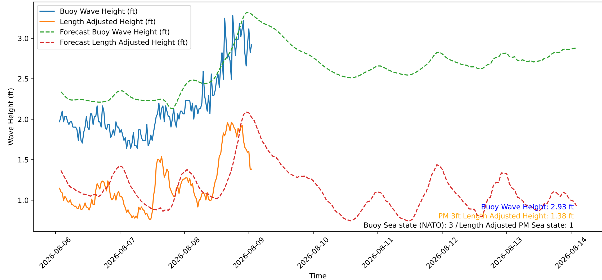
Wave Heights over Time for Oceanside Harbor at 2026-08-09 01:40:26
