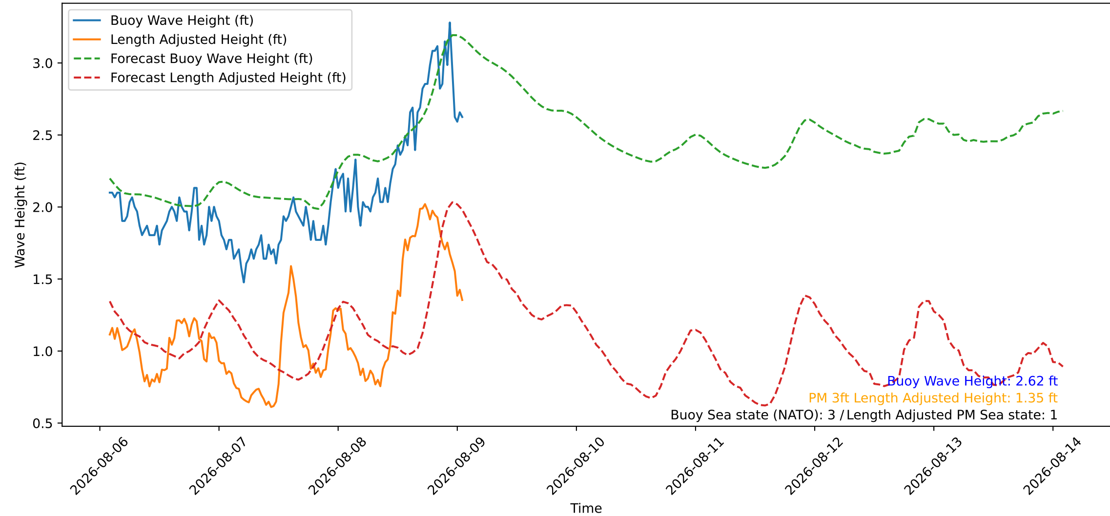
Wave Heights over Time for Red Beach at 2026-08-09 01:40:46
