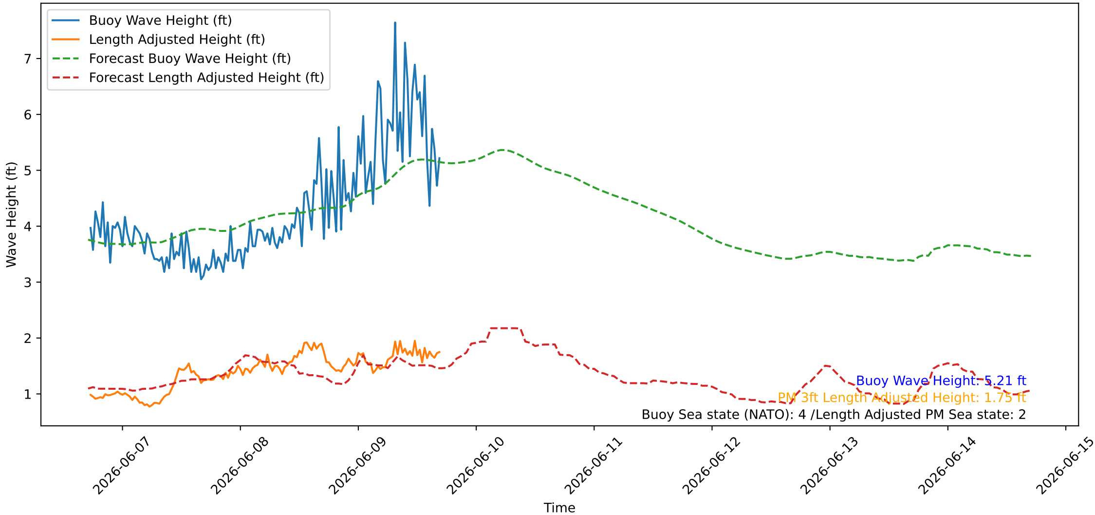
Wave Heights over Time for Red Beach at 2026-06-09 17:10:45
