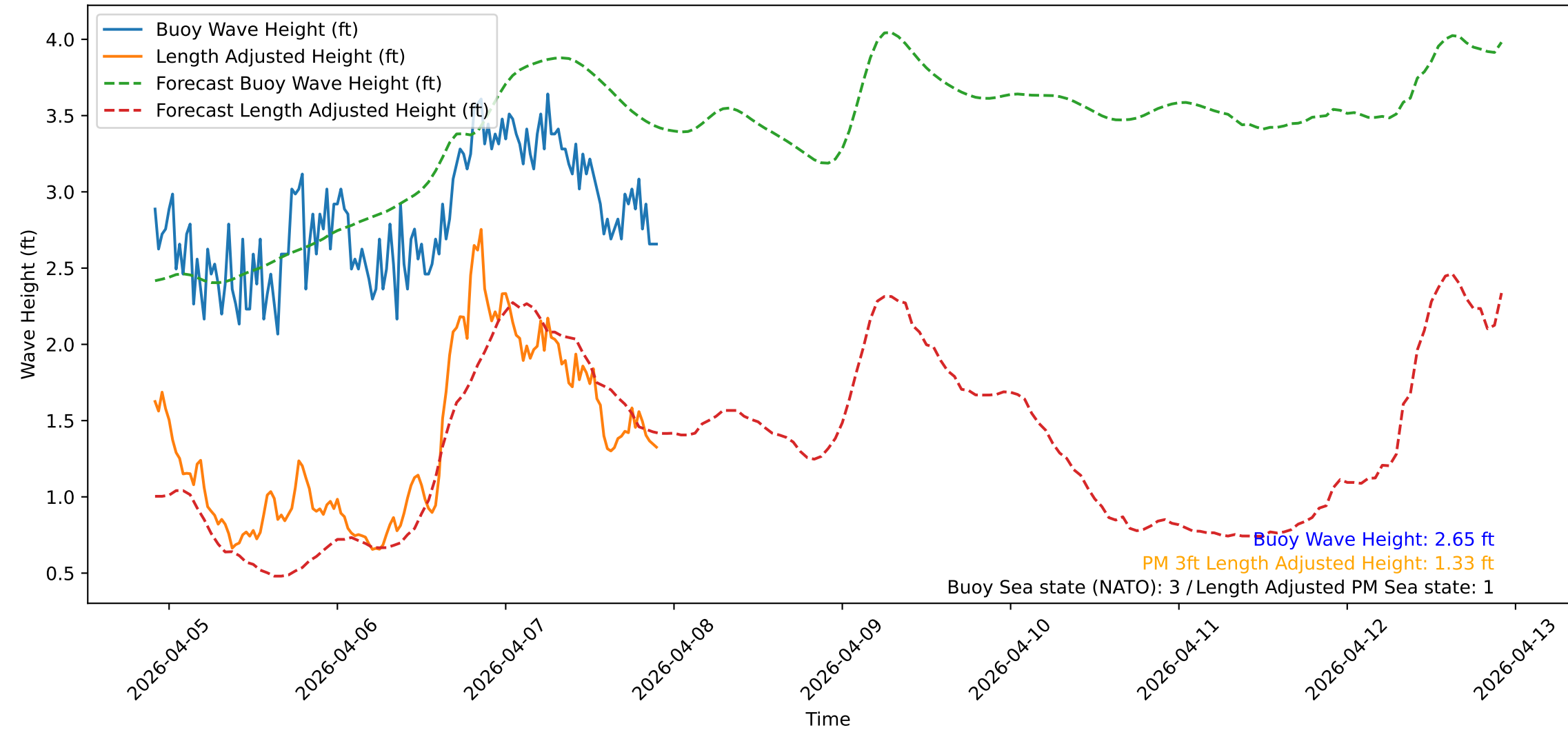
Wave Heights over Time for Oceanside Harbor at 2026-04-07 22:10:31
