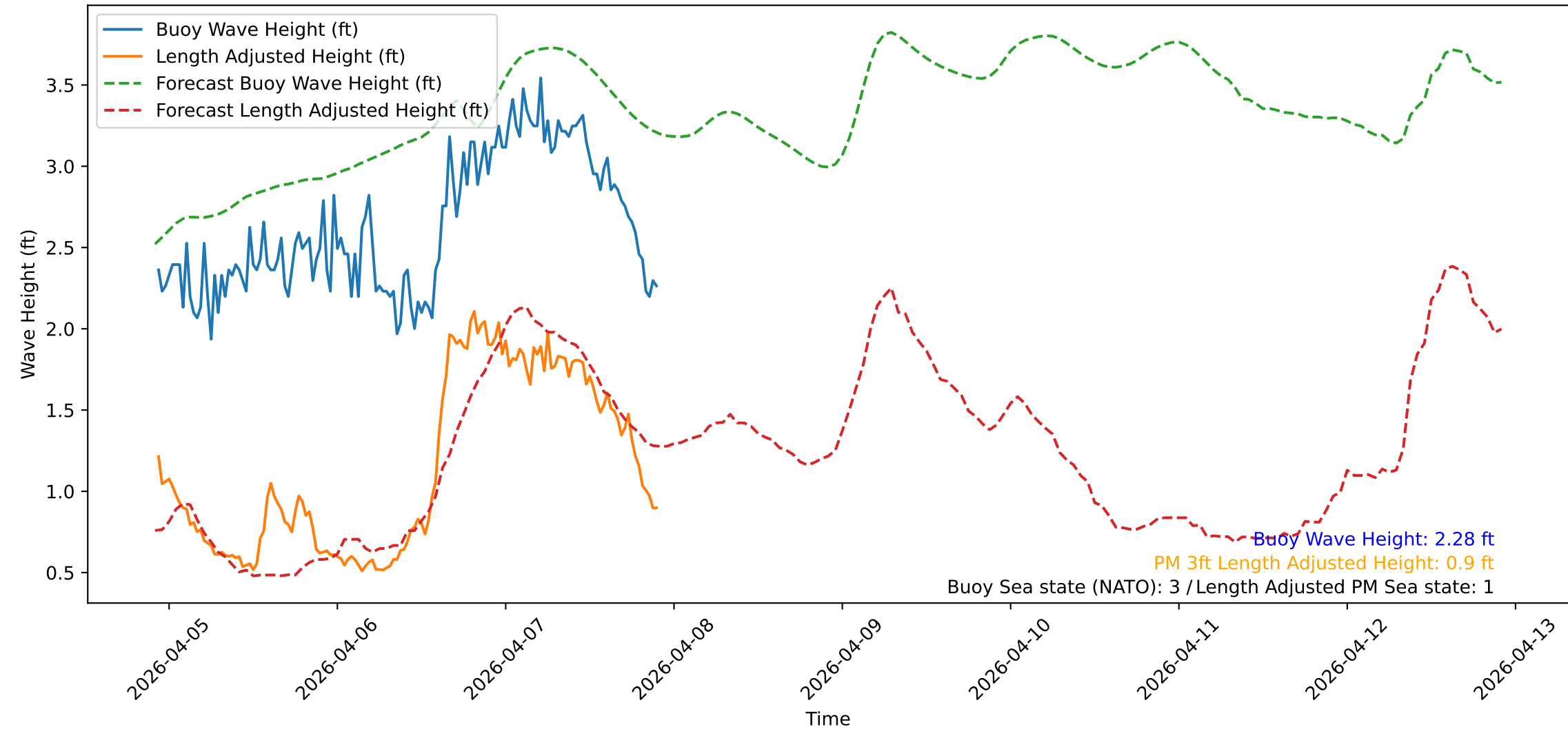
Wave Heights over Time for Red Beach at 2026-04-07 22:10:47
