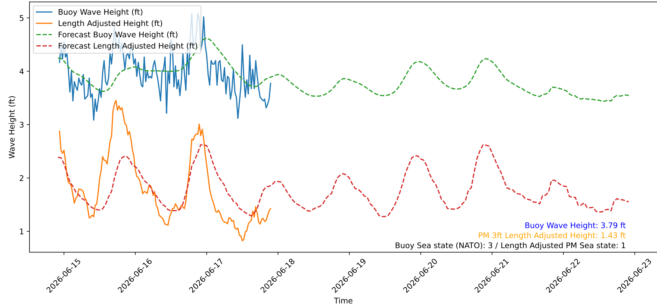
Wave Heights over Time for Green Beach at 2026-06-17 22:21:09
