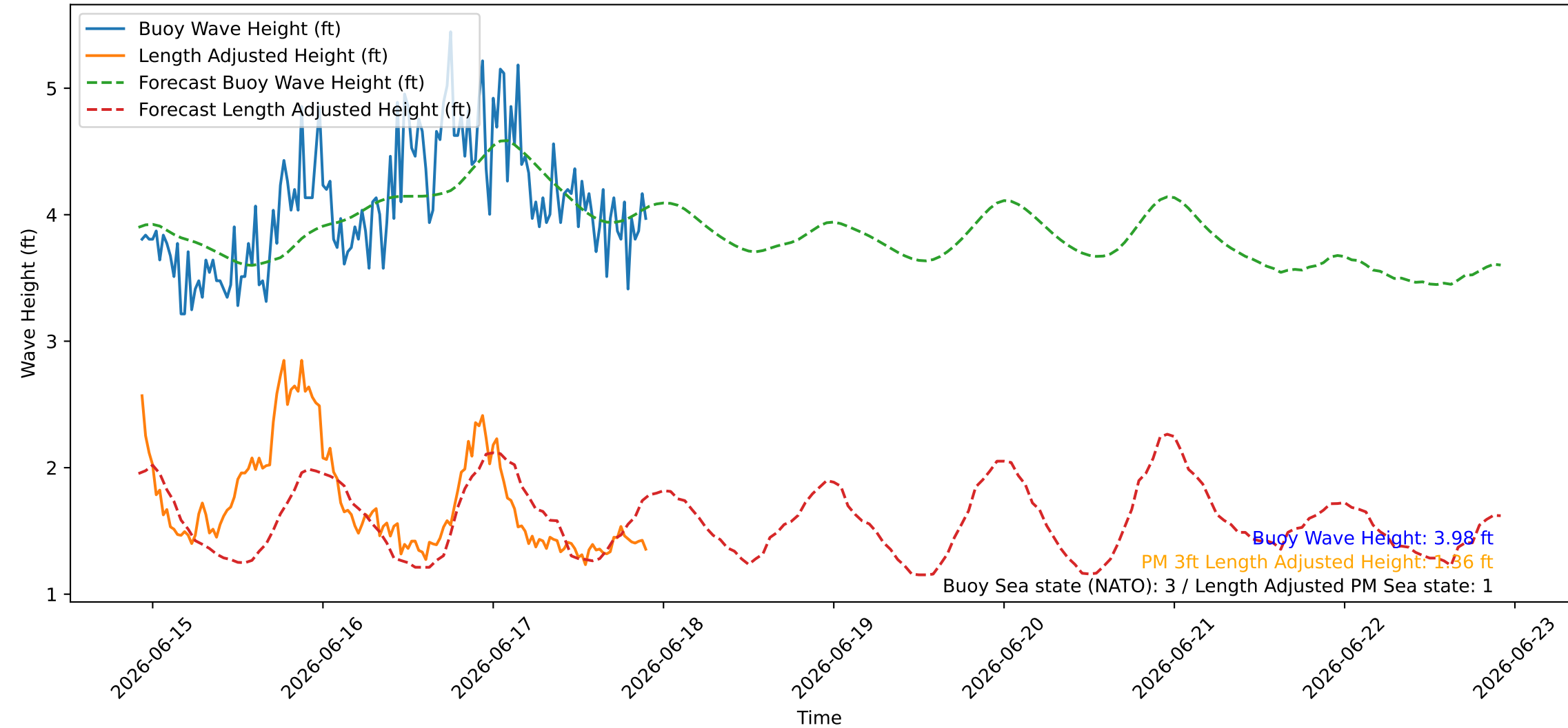
Wave Heights over Time for Oceanside Harbor at 2026-06-17 22:20:26
