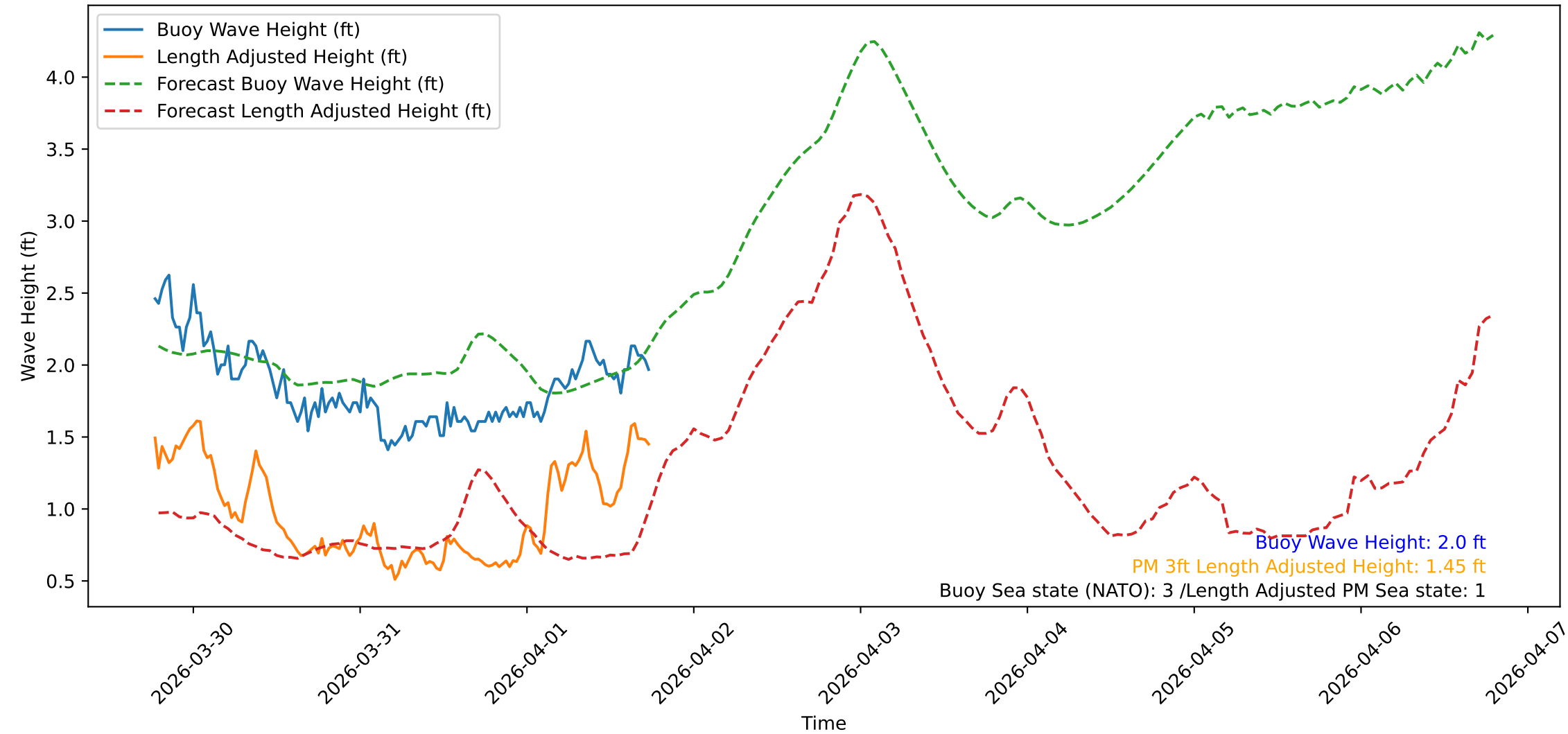
Wave Heights over Time for Green Beach at 2026-04-01 18:31:09
