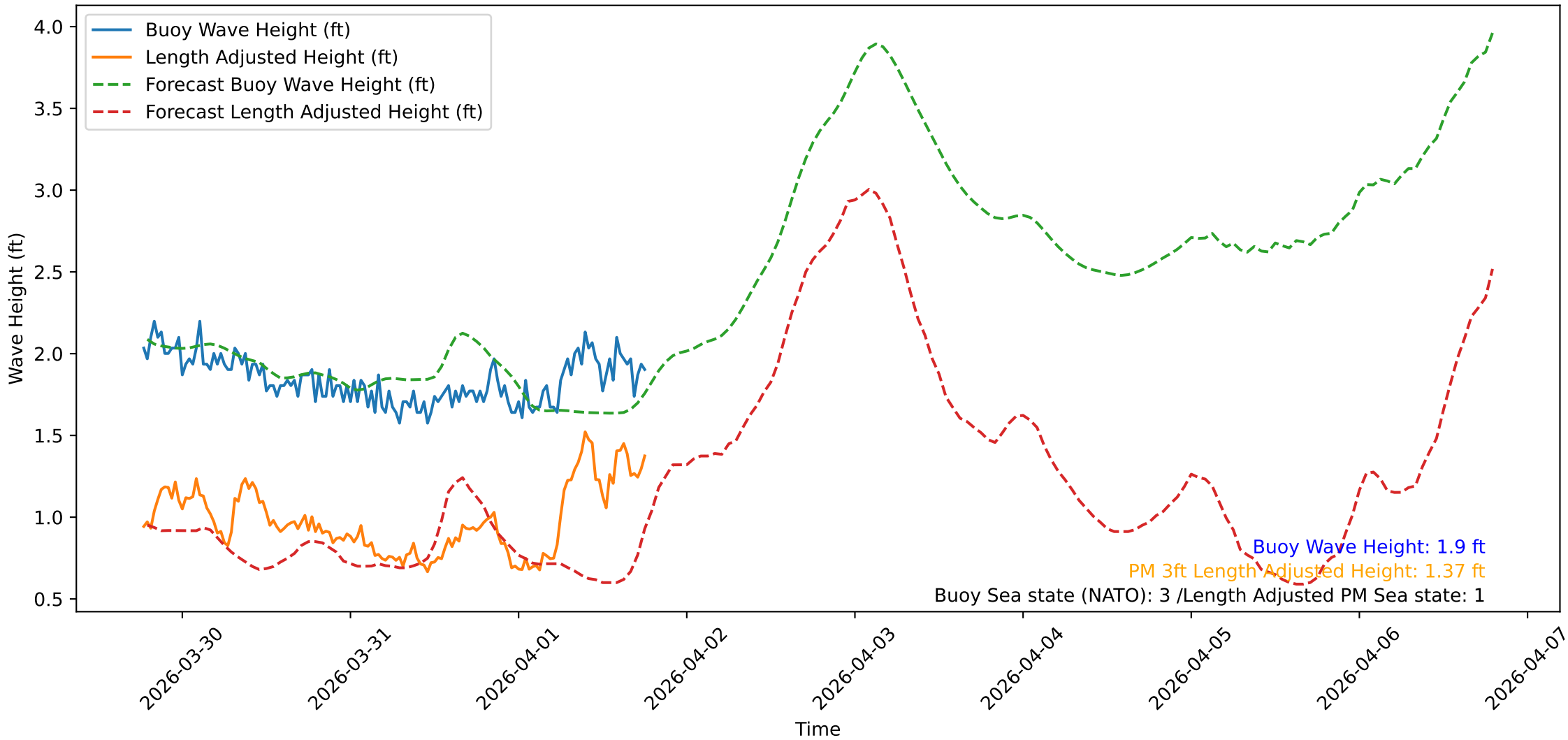
Wave Heights over Time for Oceanside Harbor at 2026-04-01 18:30:31
