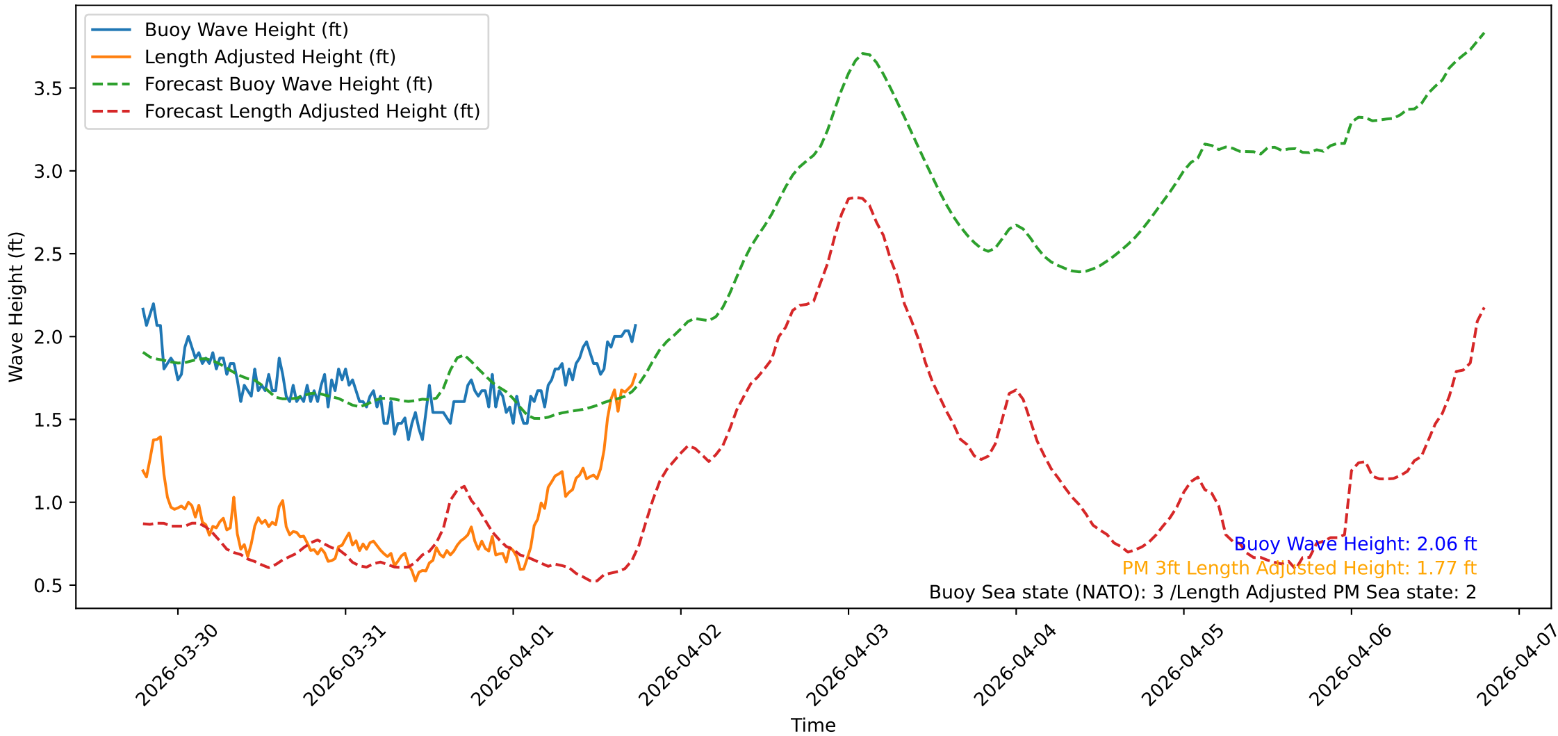
Wave Heights over Time for Red Beach at 2026-04-01 18:30:47
