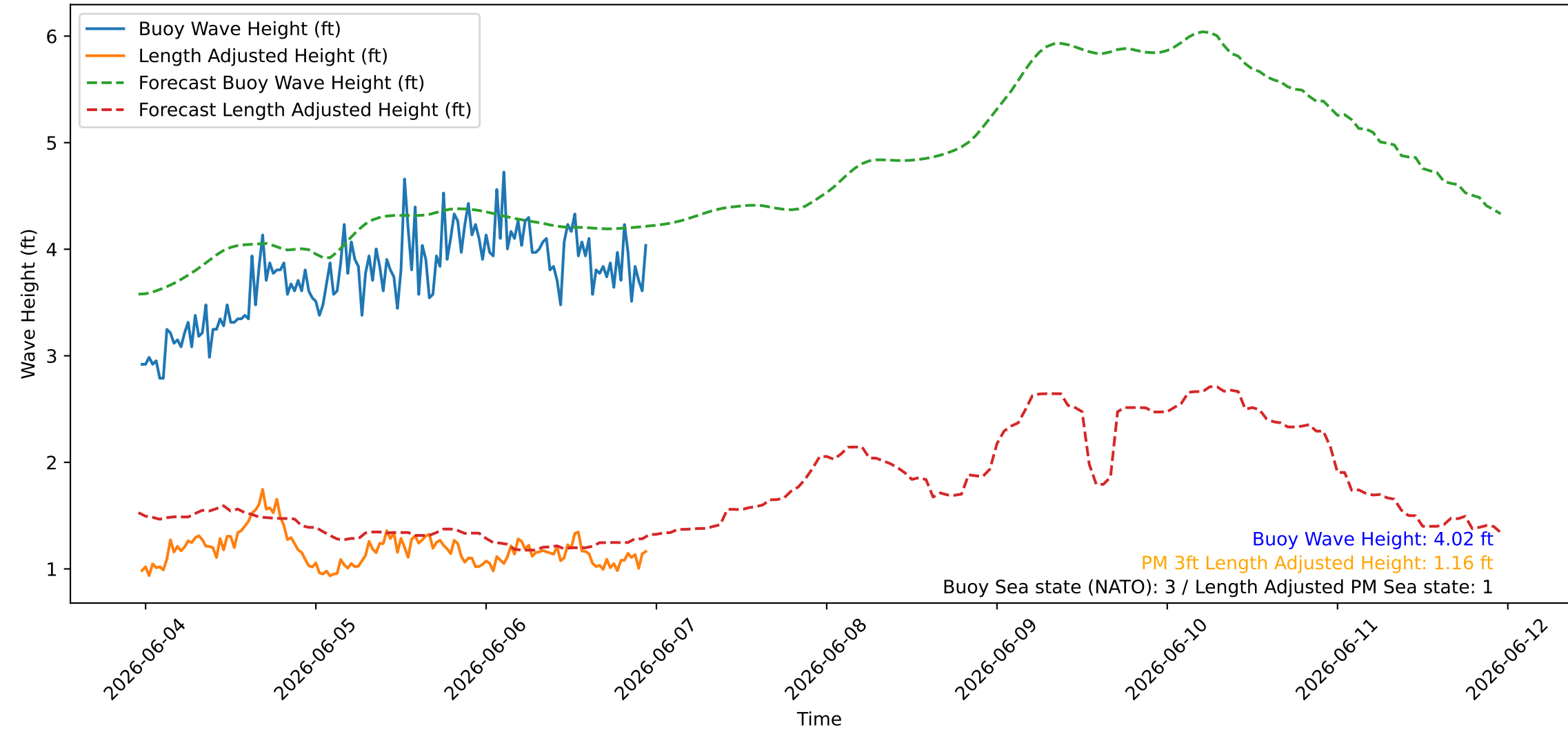
Wave Heights over Time for Green Beach at 2026-06-06 23:21:09
