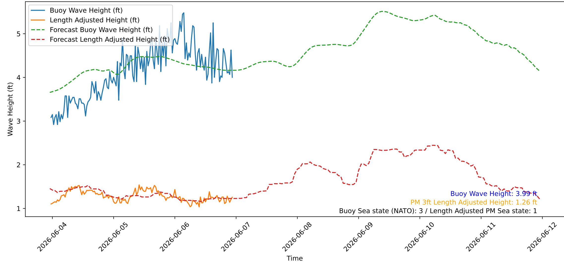
Wave Heights over Time for Oceanside Harbor at 2026-06-06 23:20:26
