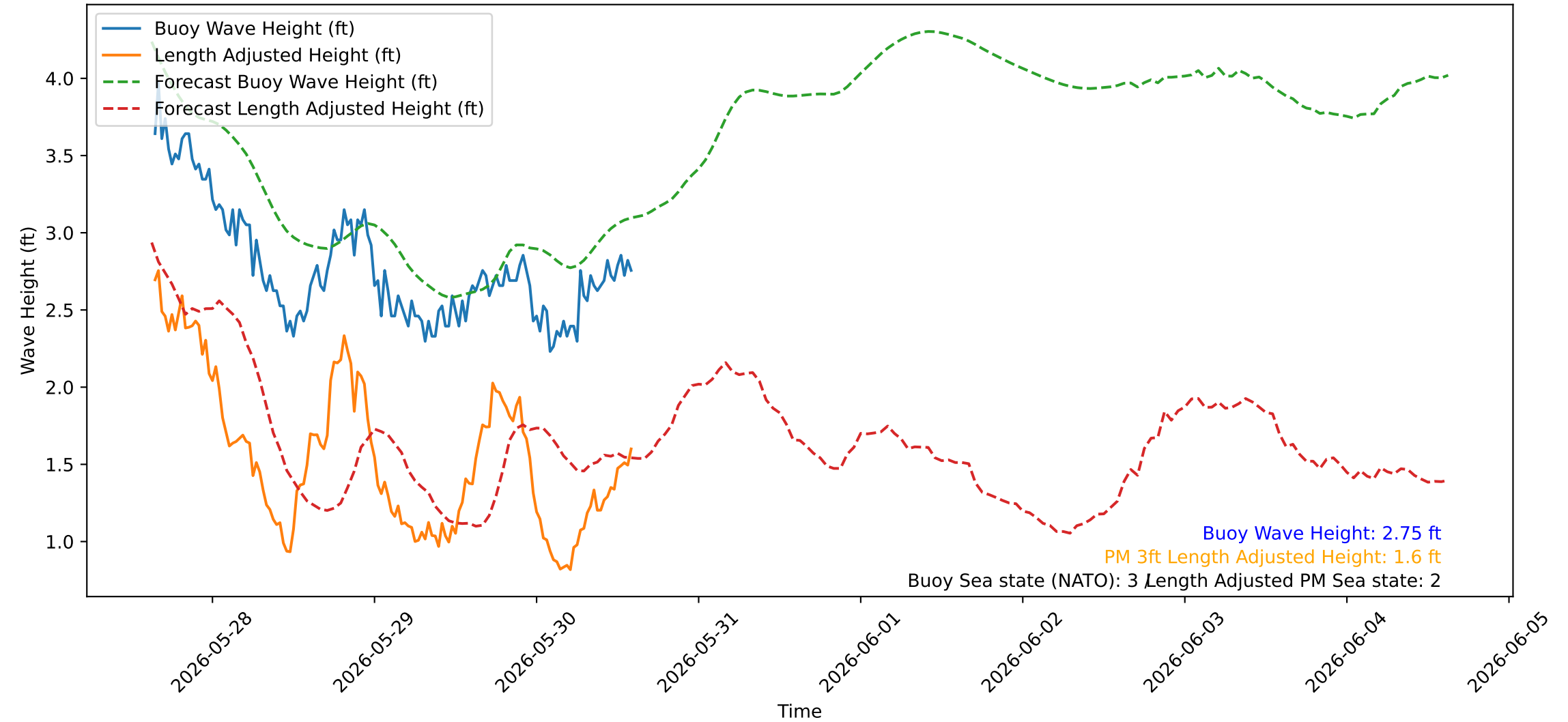
Wave Heights over Time for Red Beach at 2026-05-30 15:20:45
