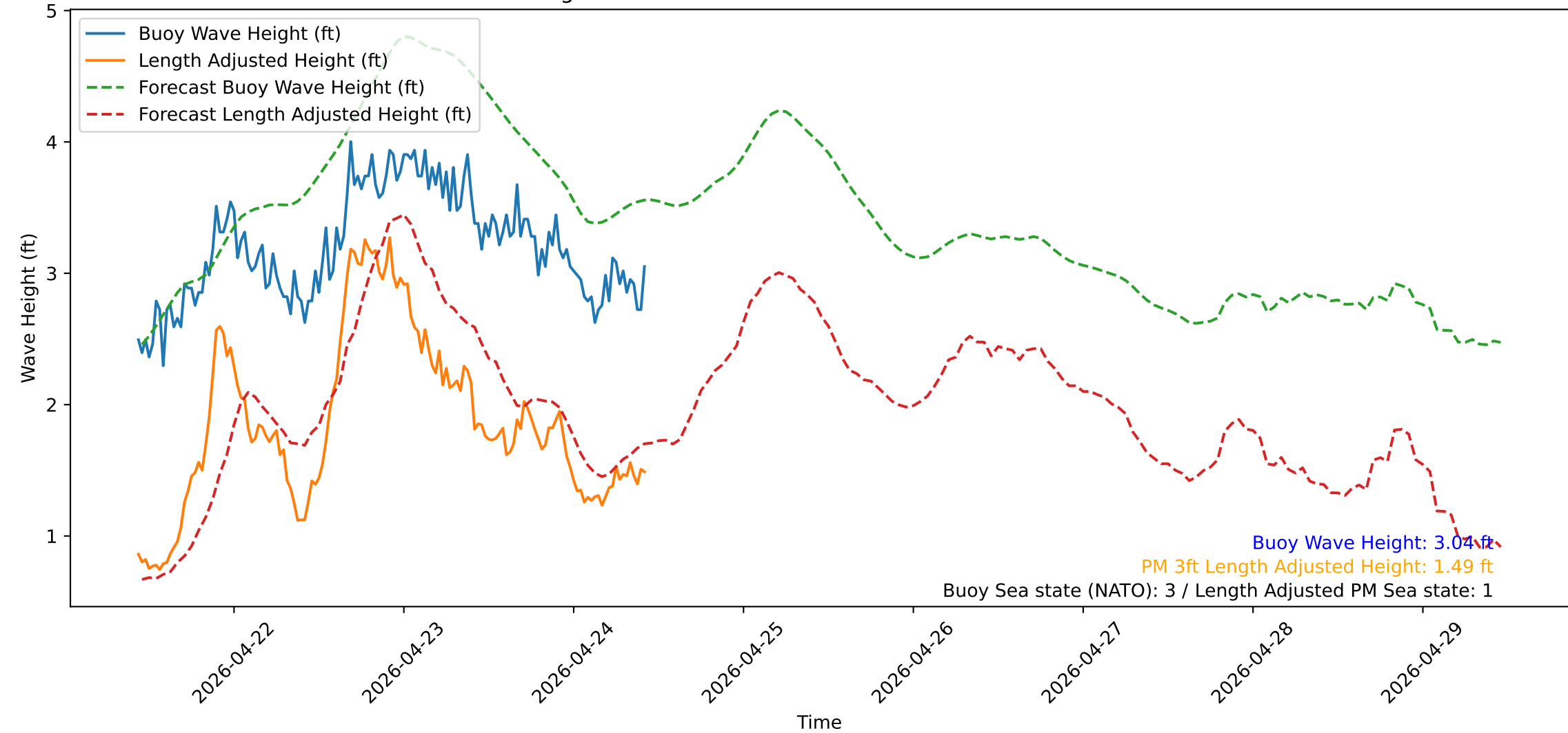
Wave Heights over Time for Green Beach at 2026-04-24 10:41:13
