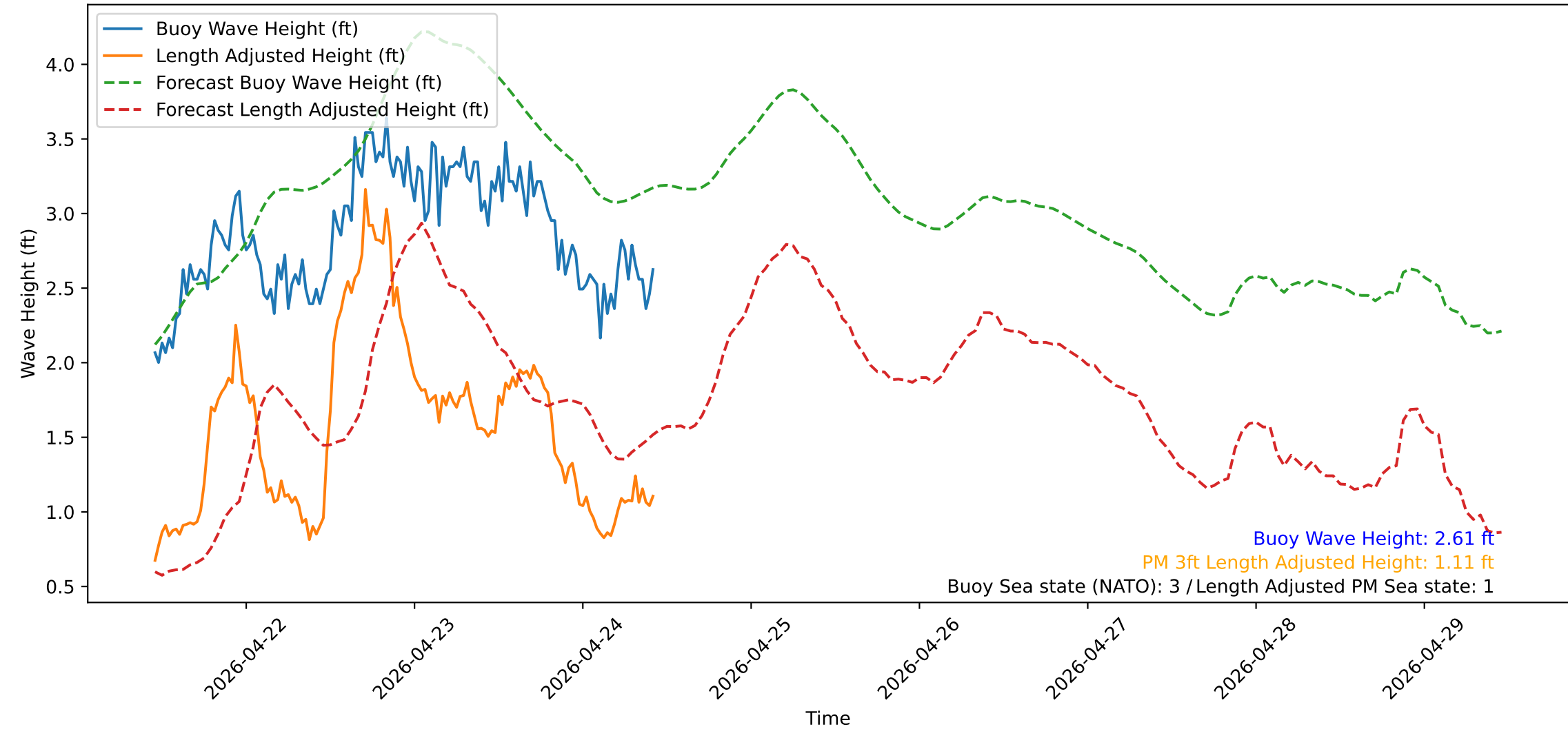
Wave Heights over Time for Red Beach at 2026-04-24 10:40:50
