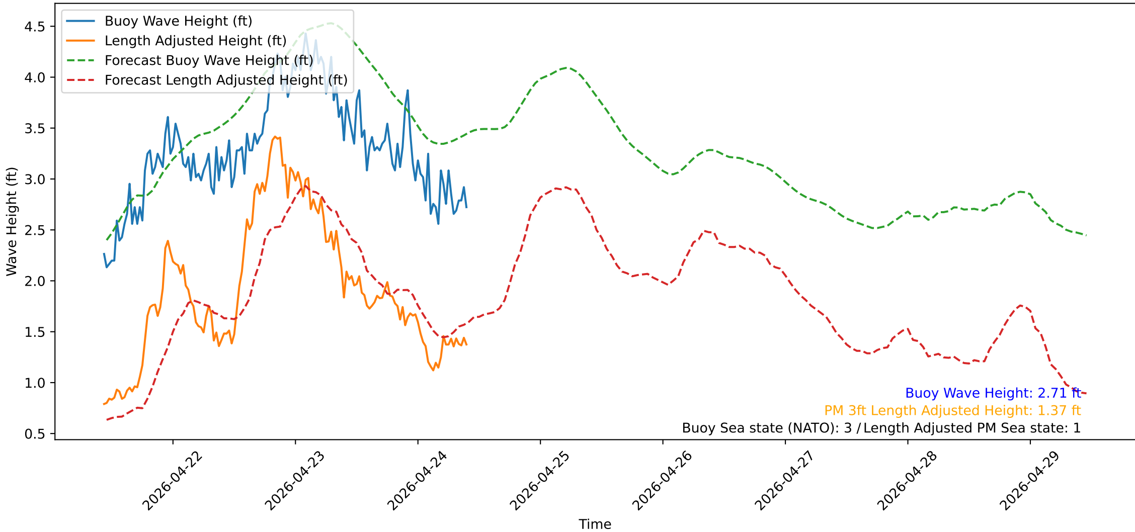
Wave Heights over Time for Oceanside Harbor at 2026-04-24 10:40:31
